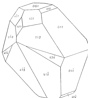
Fig. 5. Clinographic drawing of a crystal of leadhillite.
