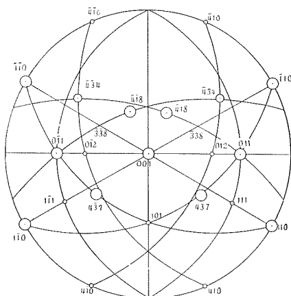
Fig. 4. Stereographic projection of the forms of leadhillite.
