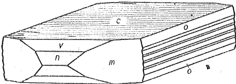
Fig. 10. Crystal of prehnite.
