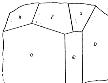
Fig. 12. Crystal of diopside. Type ii.
