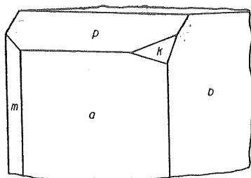
Fig. 11. Crystal of diopside. Type i.
