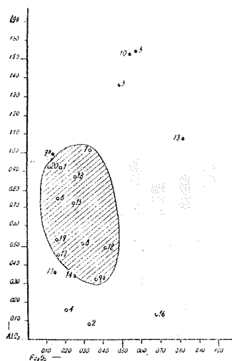
Fig. 3. Relation of Al_2O_3 - Fe_2O_3 each weight %.
