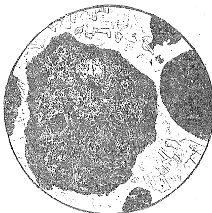
Fig. 5. Pisolitic graphite ore. \times 15
