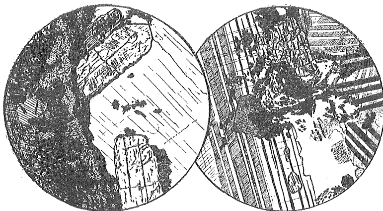
Fig. 2 The graphite accompanied by the pyroxene gabbro \times 35
