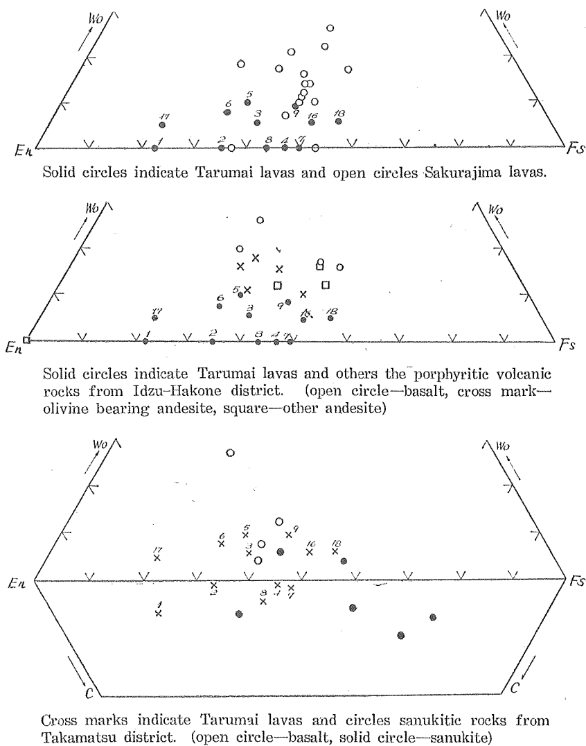
Figure 9. Diagrams showing Norm pyroxene.
