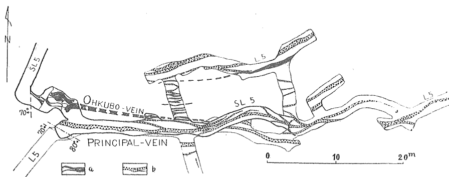
Fig. 3. Horizontal plan of ore bodies on No. 5. sublevel (80 m level) and No. 5 level (85 m level) a : Siliceous Vein b : Sulphide Vein
