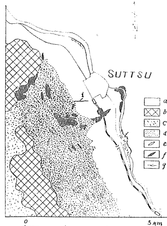
Fig. 2. Geological sketch map of the Suttu area (by OHMACHI and KIKUCHI)
