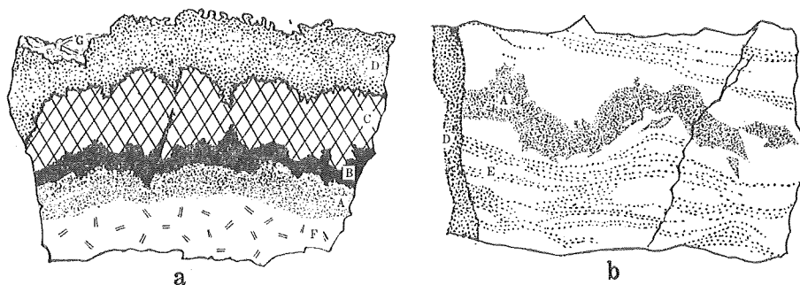
Fig. 4. Drawing of specimens of ore from the Ohkubo vein. \frac{1}{2} \times
