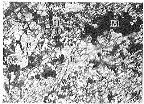
T. ISHIKAWA: Xenoliths included in the lavas from Volcano Tarumai.
