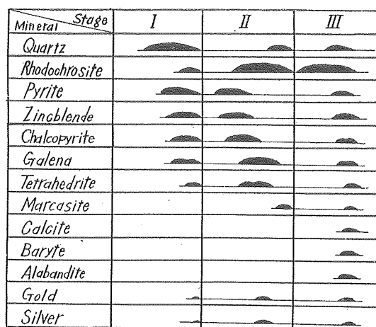
Figure 1. Crystallization in the Yakumo mine.
