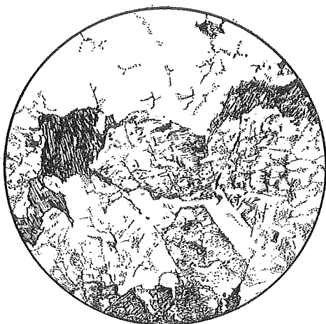
Fig. 2. Granitic rock of the Hikamiyama type. Northern part of Mt. Hikami. Diam. 4mm. Glomeroporphyritic aggregation of quartz, highly chloritized biotite with intercalating epidote and altered feldspars.
