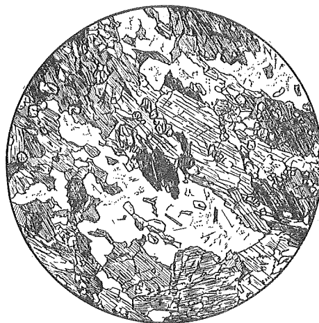
Fig. 15. Amphibolite. Tsubosawa Valley. Diam. 4mm. Green hornblende, diopside, plagioclase and sphene.
