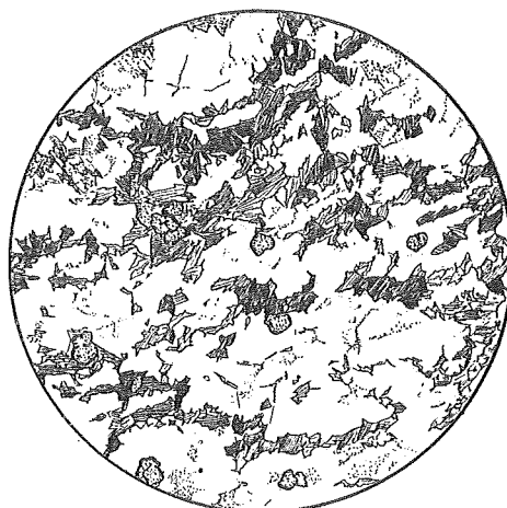
Fig. 7. Tsubosawa biotite gneiss. Tsubosawa Valley. Diam. 4mm. Quartz, plagioclase, biotite and sericite flakes arranged in a band, and garnet with a small amount of sphene, zircon and apatite.
