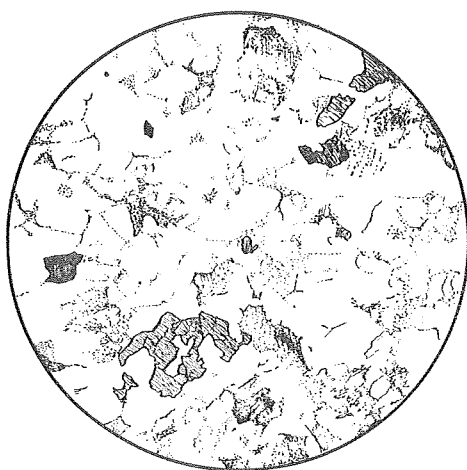
Fig. 14. The aplitic part in the Tsubosawa gneiss. Tsubosawa Valley. Diam. 4mm. Composed essentially of quartz and potash feldspar with accessory plagioclase and tourmaline.
