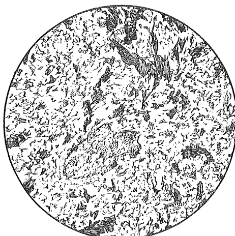
Fig. 17. Meta-porphyrite. Tsubosawa Valley. Diam. 4mm. Relict plagioclase and green hornblende surrounded by recrystallized groundmass composed of plagioclase, green hornblende and biotite.
