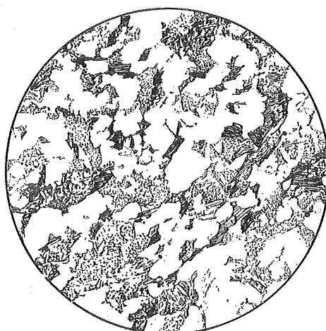
Fig. 9. Tsubosawa gneiss showing hornfels texture. Northern part of Takata city. Diam. 4mm. Principally quartz, plagioclase, biotite and muscovite.
