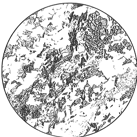
Fig. 10. Tsubosawa gneiss containing large garnet grains which were crushed by post action. Tsubosawa Valley. Diam. 4 mm.
