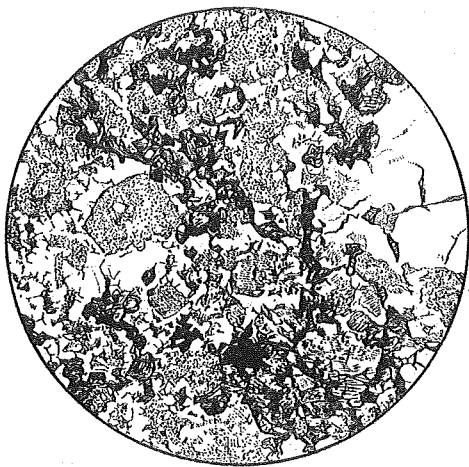
Fig. 4. Brecciated part of granitic rock of the Hikamiyama type. North eastern margin of the plutonic mass. Diam. 4mm. Brecciated quartz and feldspars, with epidote and chlorite.
