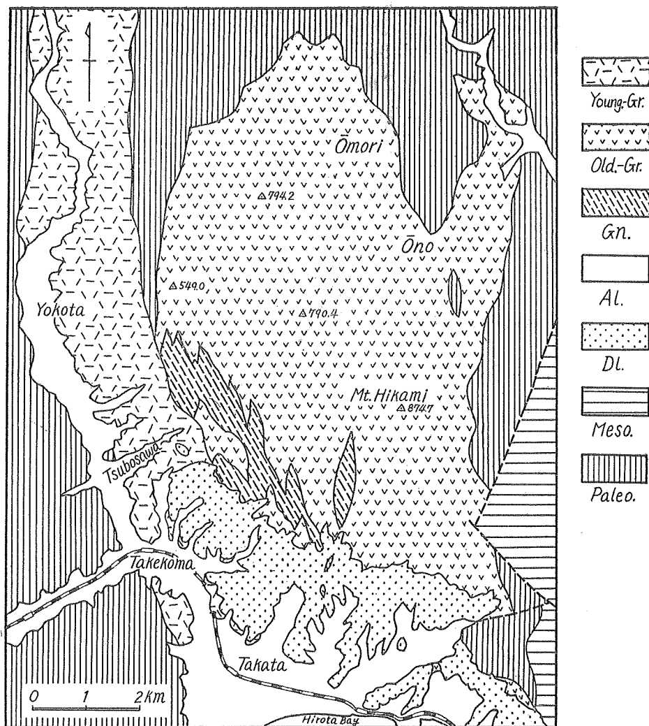
Fig. 1. Geological map of the vicinity of Mt. Hikami in southern part of the Kitakami mountain region.
