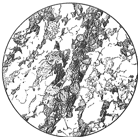
Fig. 8. Tsubosawa biotite gneiss. Northern part of Takata city. Diam. 1.5mm. The rock character is same to that of Fig. 7.
