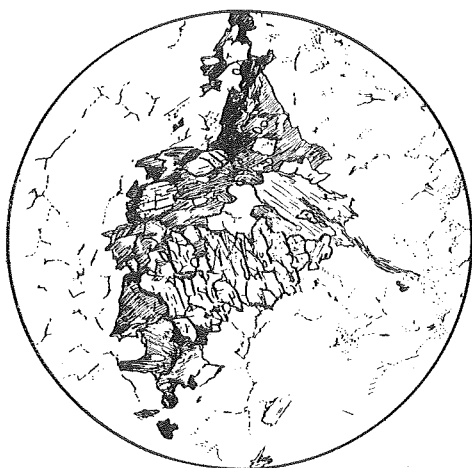
Fig. 12. Tsubosawa gneiss. The north part of Takata city. Diam. 1.5mm. Composed of andalusite, sillimanite after muscovite, biotite, quartz, and feldspars.
