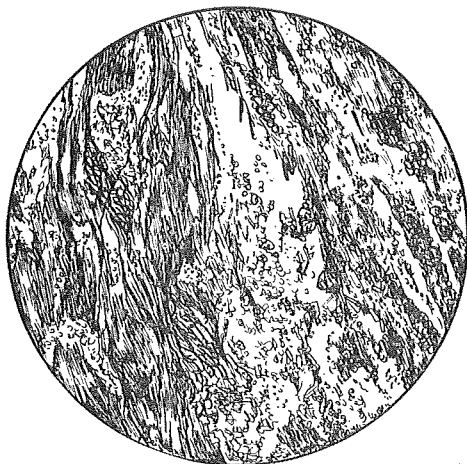
Fig. 16. Amphibolite of particular type. Tsubosawa Valley. Diam. 1.5mm. Fibrous green hornblende developed from green hornblende which partly remains; base-ment is mainly composed of quartz which includes minor epidote.
