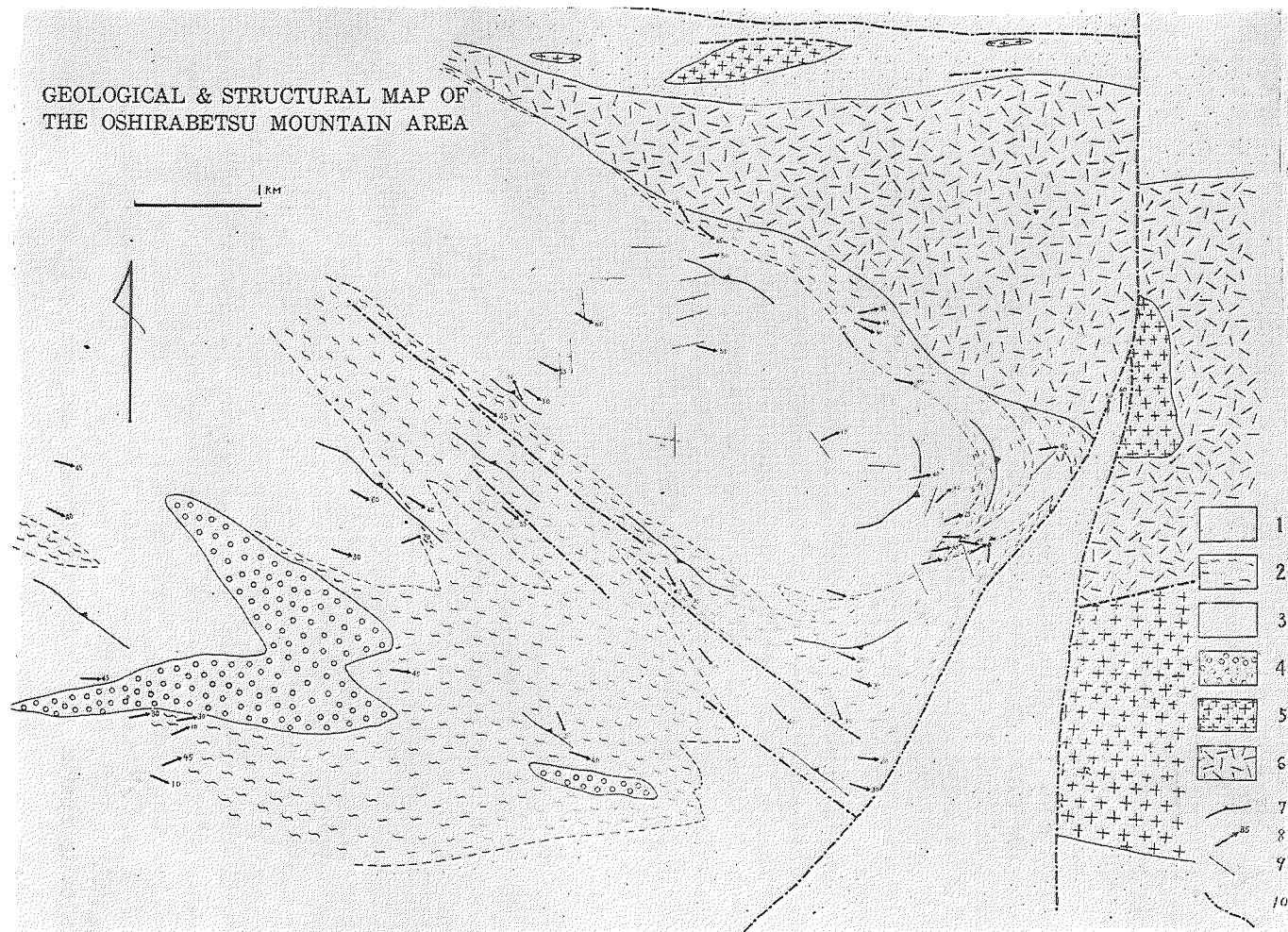
Fig. 2. Geological and structural map of the Oshirabetsu mountain area.
