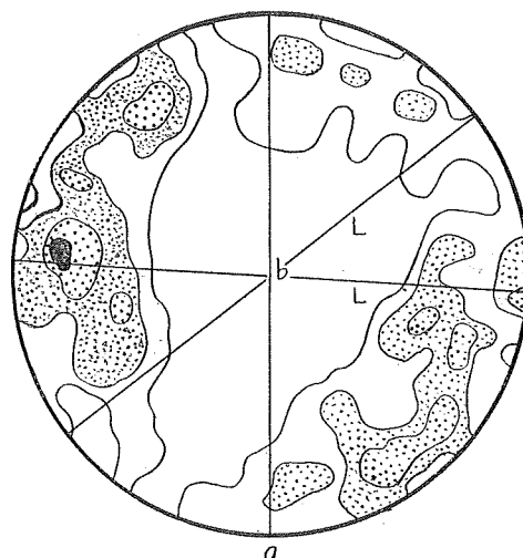
Fig. 23. 180 quartz axes from cordierite migmatite (0-221). Contours 1-3-5-7%.
