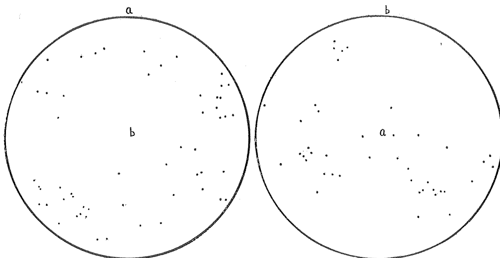
Fig. 6. Axes of quartz grains from Fig. 5.
