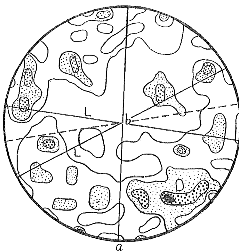
Fig. 17. 232 quartz axes from cordierite migmatite (0-105). Contours 1-2-3-4%.
