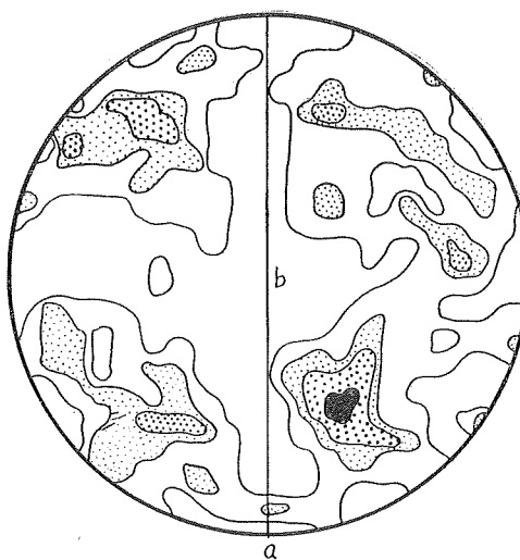
Fig. 15. 244 quartz axes from mylonitic banded gneiss (0-109). Contours 1-2-3-4%.
