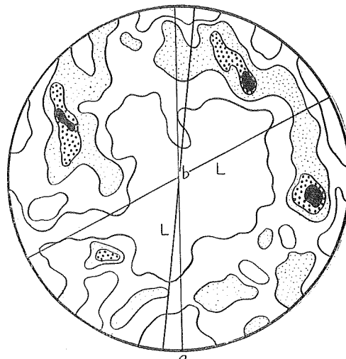
Fig. 11. 246 quartz axes from banded gneiss (0-19). Contours 1-2-3-4%.
