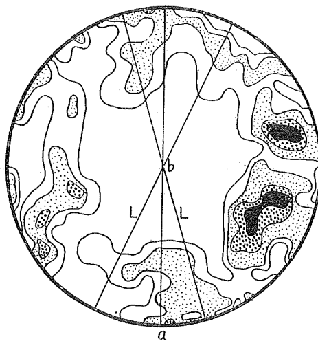
Fig. 19. 100 quartz axes from cordierite migmatite (0-23). Contours 1-3-4-6%.
