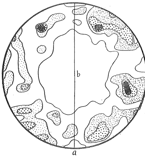
Fig. 9. 299 quartz axes from banded gneiss (0-271). Contours 1-2-3-5%.
