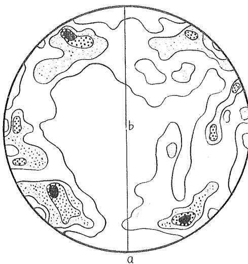
Fig. 13. 196 quartz axes from banded gneiss (0-106). Contours 1-2-3-4%.
