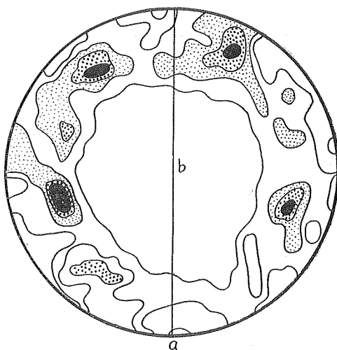
Fig. 8. 260 \frac{1}{2} quartz axes from schistose hornfels (0-267). Contours 1-2-3-4%.
