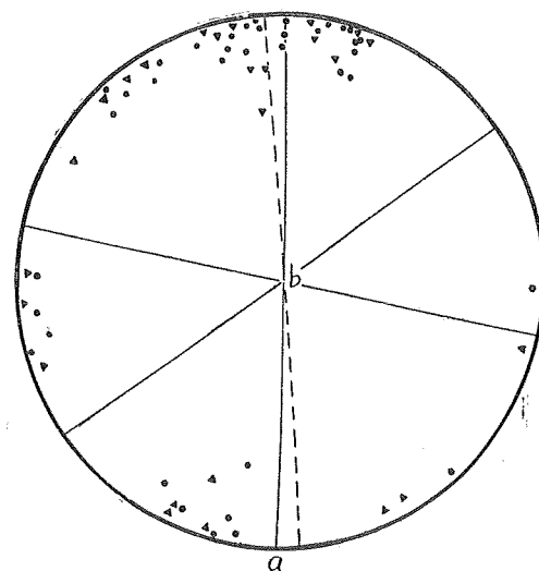
Fig. 27. Poles of Böhm lamellae in quartz grains (filled circles) and that of fractures in plagioclase grains (filled triangles)
