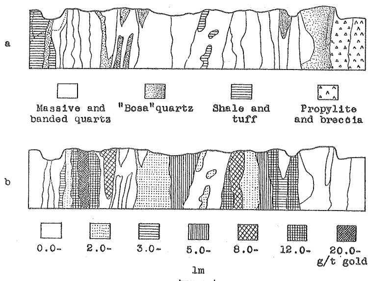
Fig. 3. A profile of the Sumiyoshi 1st Vein.
