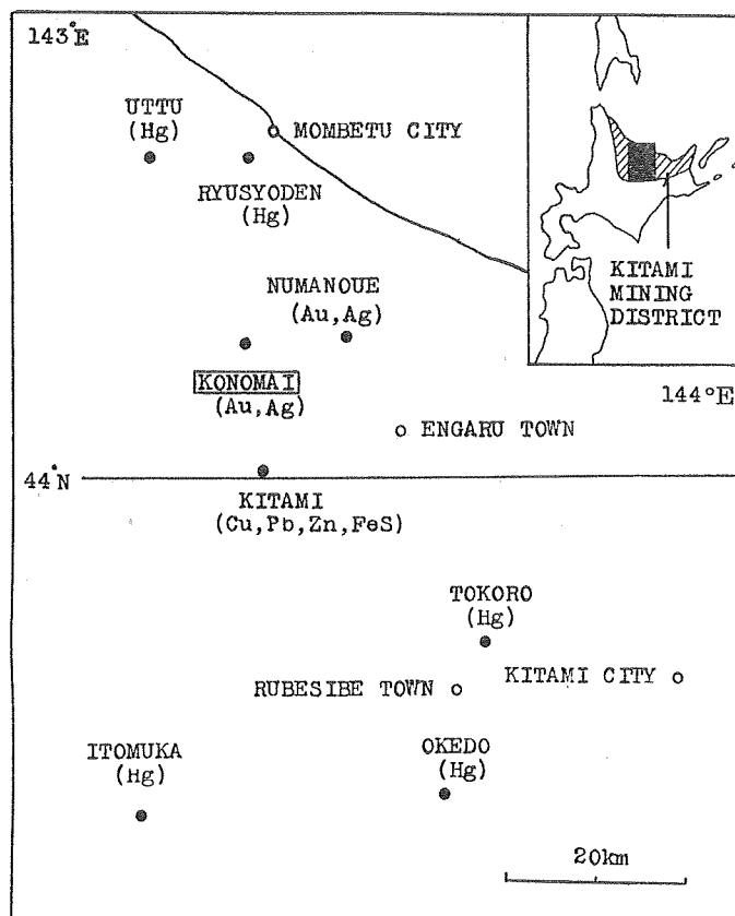
Fig. 1. Index map showing location of the Konomai Mine, Hokkaido.
