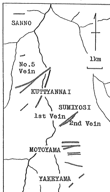
Fig. 2. Distribution of the Sanno, Kutyannai, Sumiyoshi, Motoyama and Yakeyama Ore Deposits of the Konomai Mine.
