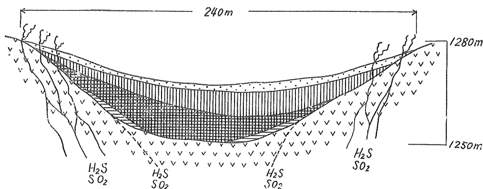
Fig. 7. Diagrammatic profile of the "Ôfuki" ore deposit. (Symbols are the same as those in Fig. 4.)
