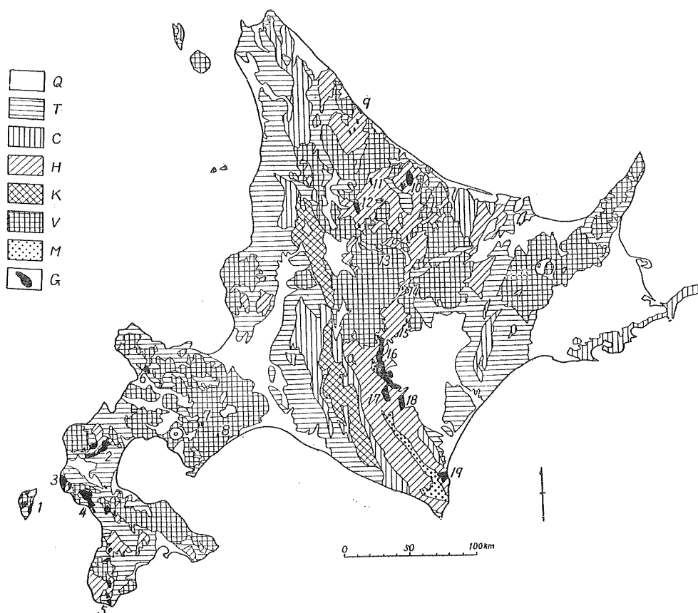
Fig. 1. Distribution map of granitic rocks of Hokkaido
