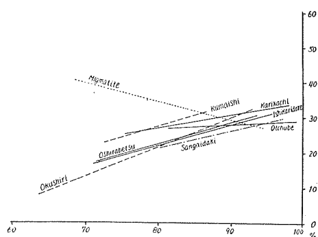
Fig. 4a. Quartz
