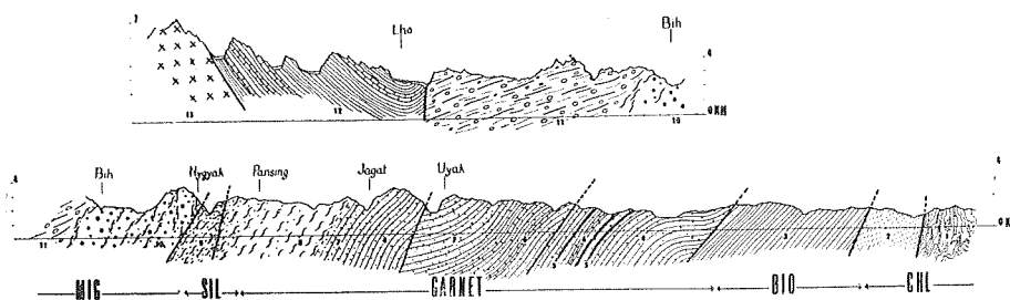
Fig. 2. Section across the central Nepal Himalaya along the Pass of Samri to Larkya Pass.
