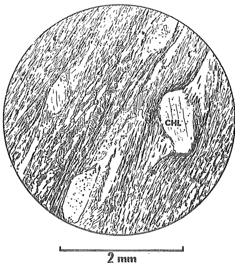
Fig. 3. Chloritoid chlorite schist near Tharp village CHL: chloritoid
