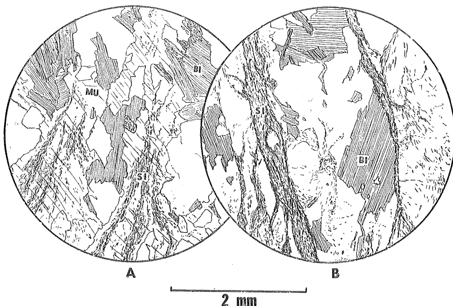
Fig. 7. Sillimanite mica gneiss near the village of Nygyak.
