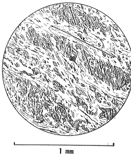
Fig. 4. Sketch showing intersection of the schistosity. S_1 : earlier formed s-plane, characteristic mineral association being chlorite and albite. S_2 : later-formed s-plane, being characterized by an alignment of sericite flakes.
