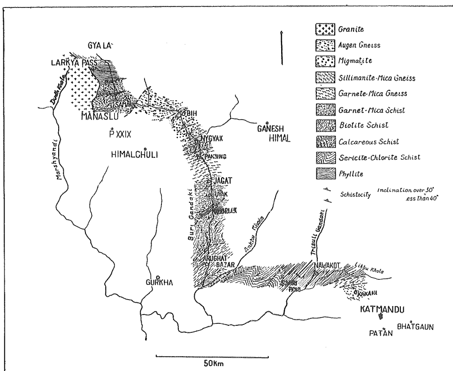
Fig. 1. Geological traverse map along the expedition route.
