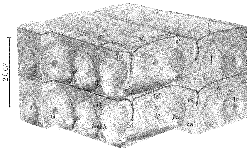
Text-Fig. 8. Diagram of inside of chamberlets. t : true thickness of keriotheca. t' , t'' : wrong measurement of the thickness of keriotheca. d_1 : distance between the adjacent transverse septula. d_2 : distance between the adjacent septa. d_1 and d_2 make chamberlet." Ts : Transverse septula. ts' : axial septula. fm : foramina. lp : lateral passage. ch : parachomata. Those signs are also used in Text-Fig. 6.
