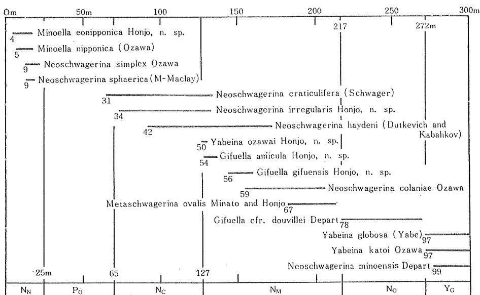
Text-Fig. 3. Ranges of Neoschwagerinids from the Akasaka Limestone, route r-r'.
