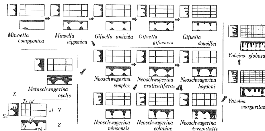
Text-Fig. 6. Sepular patterns of neoschwagerinids. Allow marks show the course of evolution. See Text-Fig. 8, p. 123.
