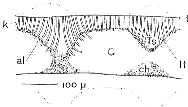
Text-Fig. 7. Diagram of a part of an axial section of a volution in Bident replica, Neoschwagerina simplex . Each alveolus (al, slightly larger than natural) stands separately from others, some lower part of the alveoli sticks out of the lower tectorium (lt). Lower tectorium does not seen inside of an alveolus. C: chamberlet cavity; t: tectum. As is seen in text-fig. 2, alveoli bend in both axial and sagittal planes. Alveolar divergency only in an axial plane is expressed in this diagram.
