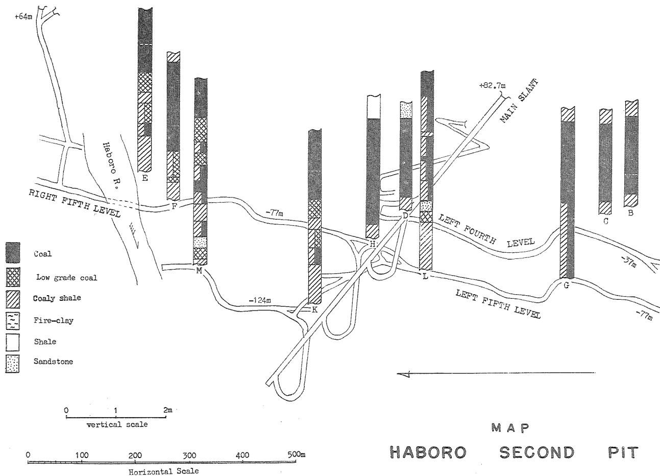
Fig. 3. Showing sampling localities and columnar sections.
