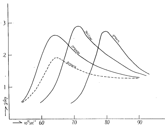
Fig. 6. Absorption curve of sphalerite from Hosokura mine.
