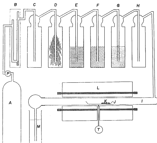
Fig. 3. Apparatus of sulphur analyses.
