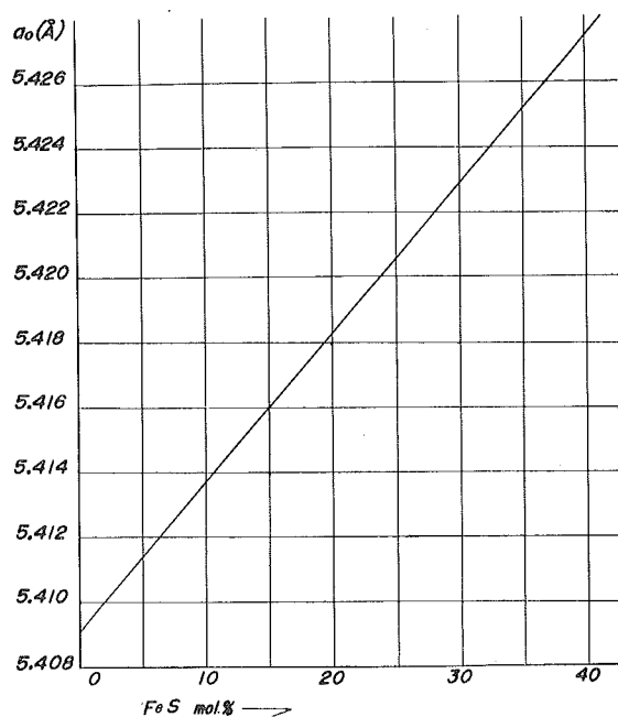
Fig. 4b. Relation between FeS content and lattice constant.
