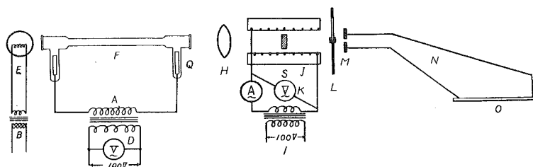
Fig. 5. Photographing apparatus of absorption curve.
