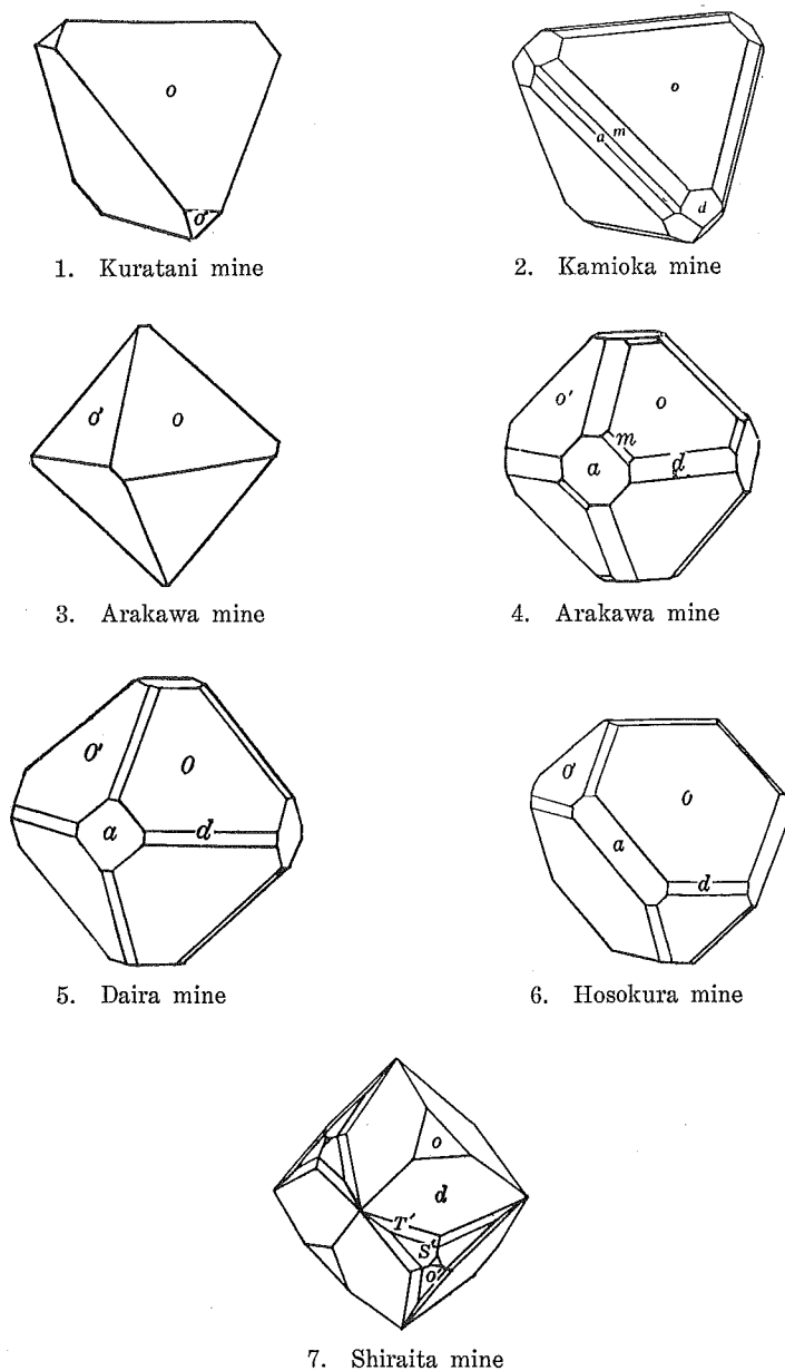
Fig. 1. Crystal forms of Japanese sphalerites. 2, 3—after Katayama N. (1933) 1, 4, 7—after Ito T. (1937) 5, 6—after Ito T. (1947)
