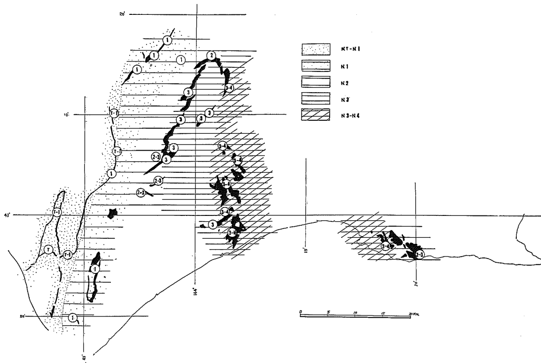
Fig. 11. Biofacies map of the middle part of the Shitakara formation.
