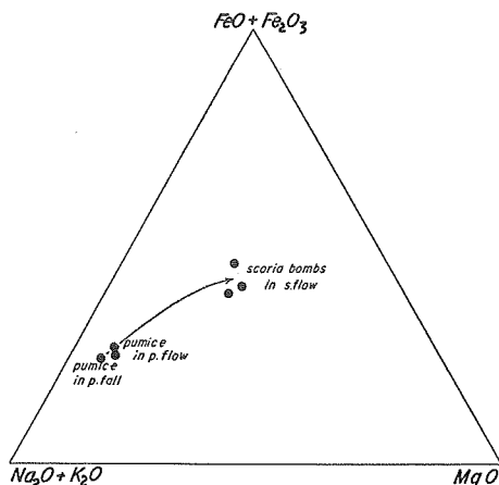
Fig. 10. Change in composition of the successive ejecta in the culminating eruptions of Mt. Mazama. (after WILLIAMS, 1942)
