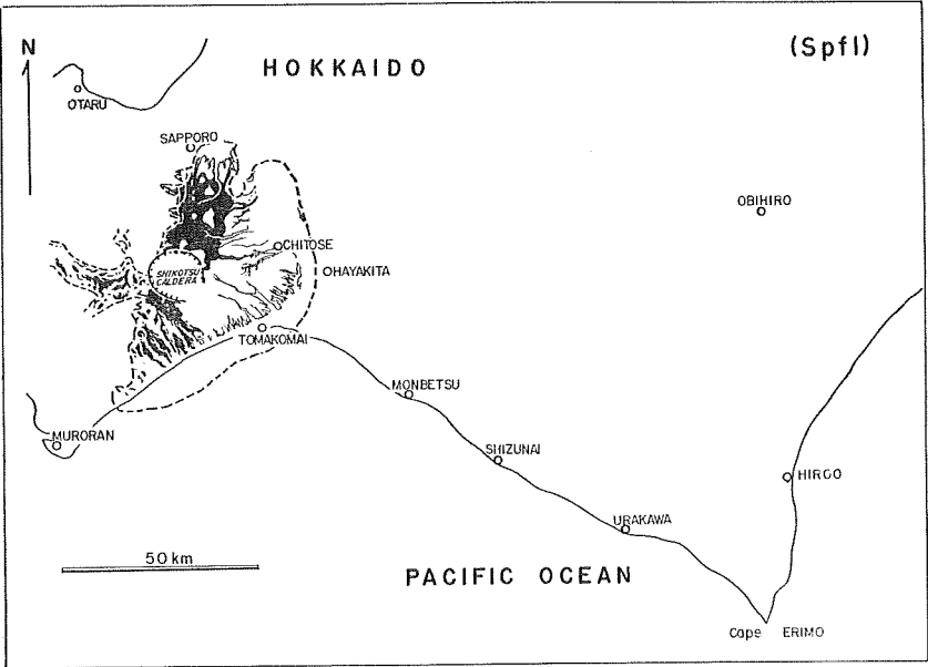
Fig. 4. Distribution of the Shikotsu pumice-flow deposit (Spfl-1 and 2). after DOI and OSANAI (1956)
