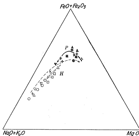
Fig. 15. MgO-FeO+Fe 2 O 3 -Na 2 O+K 2 O diagram for the volcanic products in strato-cone building stage (solid or thick marks) and caldera building stage (open or thin marks) of some Krakatoan calderas in north Japan. (Symbols same as Fig. 14)
