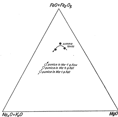
Fig. 9. Variation in composition of the somma lavas and pumice of the culminating eruption of the Mashû volcano.
