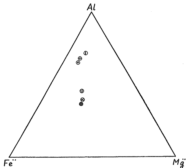
Fig. 13. Al-Fe-Mg diagram of biotites and of the bulk composition of the rocks containing them. ①: biotite of banded biotite gneiss (①), ●: biotite of biotite migmatite (●), ⊗: biotite of granitic migmatite (⊗)
