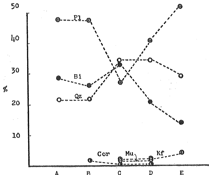
Fig. 12. Variation diagram of mode. A: biotite hornfels, B: schistose biotite spotted hornfels, C: banded biotite gneiss, D: biotite migmatite, E: granitic migmatite.
