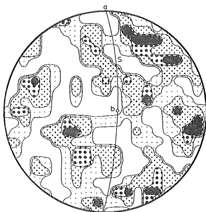
Fig. 13-i Specimen 9 , 300 quartz [0001] axes from banded gneiss Contours 2.5-2-1.5-1%
