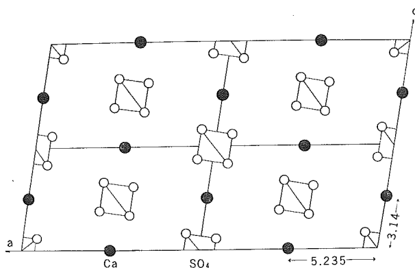
Fig. 2 Arrangements of Ca and \text{SO}_4 ions in the layer parallel to the (010).
