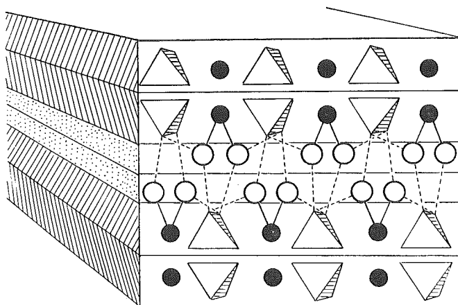
Fig. 1 Schematic illustration of the layer structure of gypsum, showing a section parallel to the (001). The solid circles denote the positions of Ca, the open circles those of water molecules, and the tetrahedrons \text{SO}_4 .
