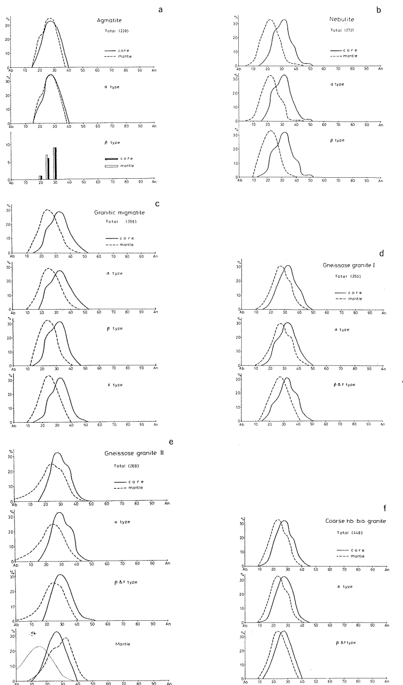
Fig. 3. An frequency curves based on unit range \pm 2.5\% \text{An} of each lithofacies. "α type" means plagioclases of 0.5 mm x 0.5 mm in maximum size. "β type" means those of 0.5–1.5 mm x 0.5–1.0 mm in size. "γ type" means those of 1.5 mm x 1.0 mm in minimum size.
