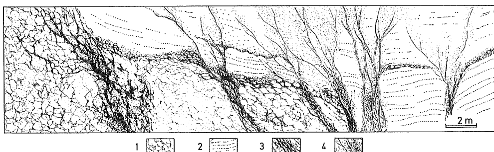
Fig. 3 Sketch of the representative outcrop in celadonitized zone. 1 ; network celadonitized seams 2 ; tuffaceous member intercalated between massive lavas 3 ; strongly celadonitized vein formed part 4 ; mordenite-cristobalite vein
