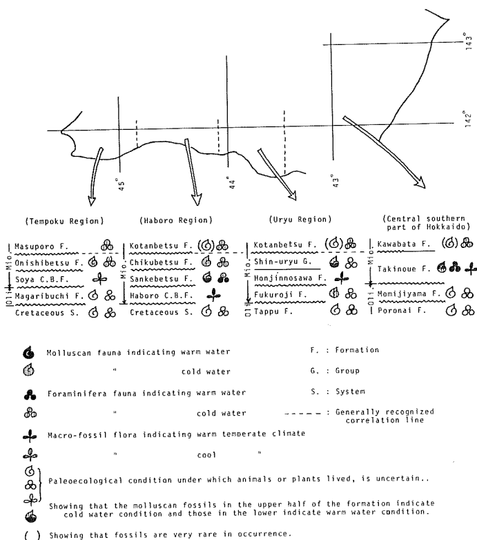
Fig. 1 General stratigraphic sequence of lower-middle Miocene sediments in Central Hokkaido
