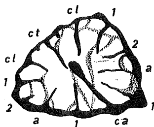
Fig. 7. Transverse section of a young corallite of Lithostrotionella kitakamiensis MINATO. X10
