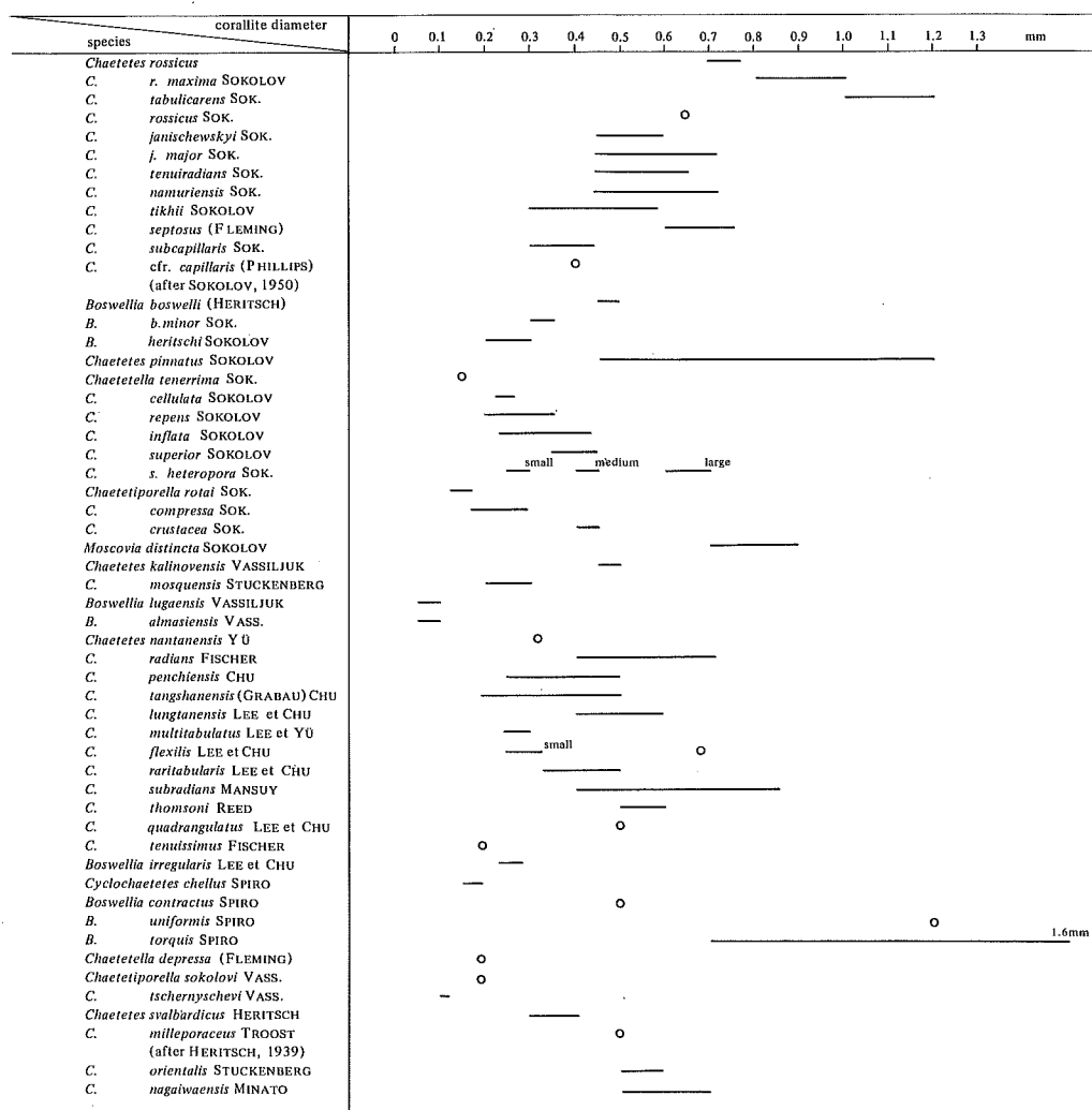
Fig. 4 Range of the size of corallite in some cerioid forms of Carboniferous Chaetetids.
