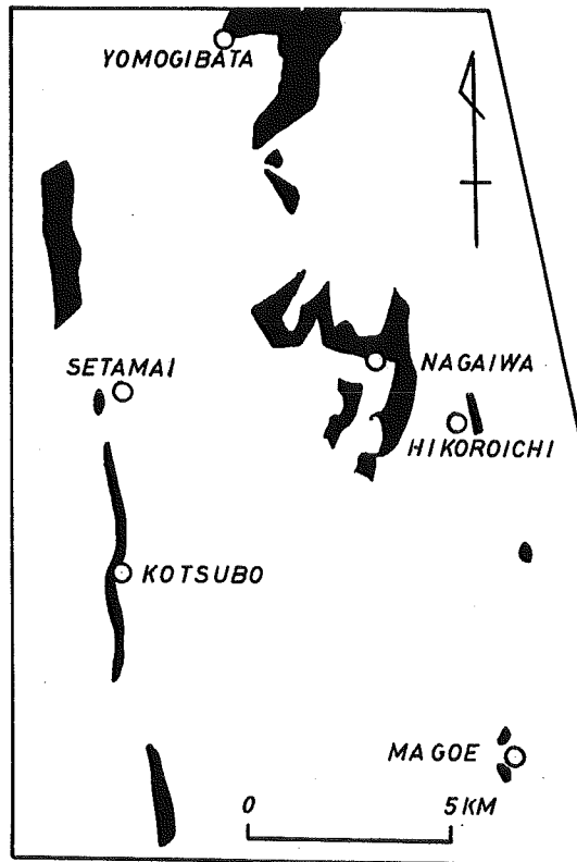
Fig. 3. Sketch map showing the known distribution of the Nagaiwa series in and around the Setamai - Hikoroichi region, Iwate Prefecture.
