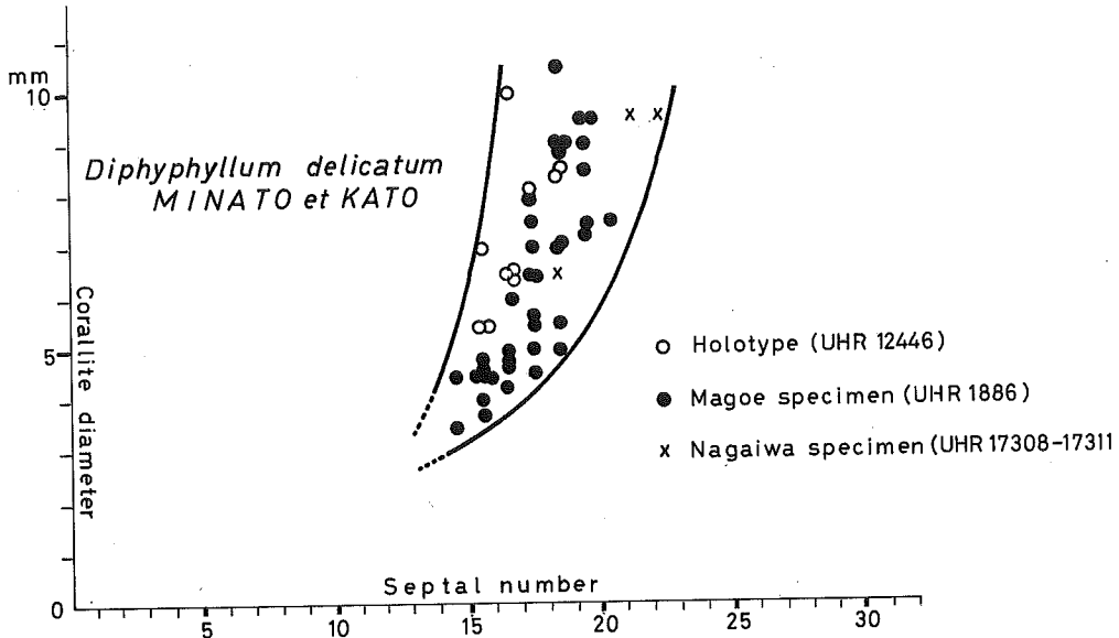
Fig. 5. Scatter diagram showing relation between diameter of corallite and number of major septa in Diphyphyllum delicatum MINATO et KATO.
