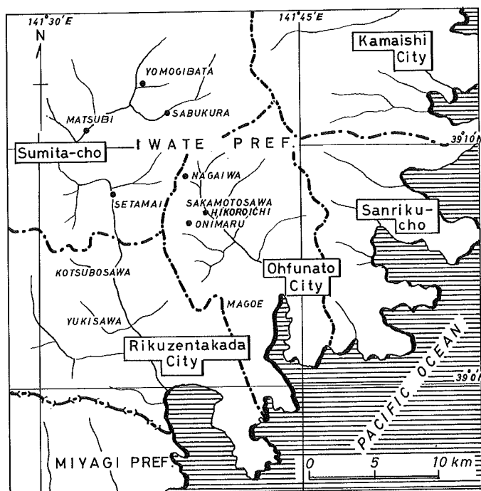
Fig. 1. The Southern Kitakami Mountains, showing chief localities wherein coral-bearing Nagaiwa series occurs.
