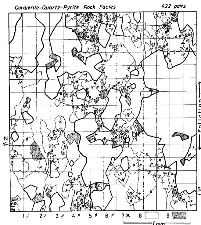
Fig. 24 Distribution Map of c -axis coordination on each concentration angle of the squared area in Fig. 6.
