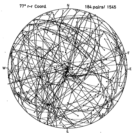
Fig. 23c Peak girdle at 77^\circ peak in cordierite-quartz-pyrite rock facies
