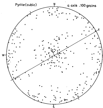
Fig. 32-(4) Pyrite fabric pattern of anthophyllite-cordierite-quartz-pyrite rock facies.
