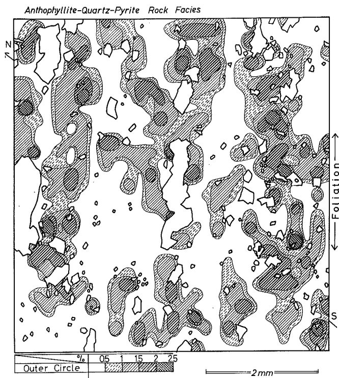
Fig. 12b A.V.A. Contour map belonging to outer circle of Fig. 9, which is maintained by making the statistical contour lines of concentration grade in respective group.
