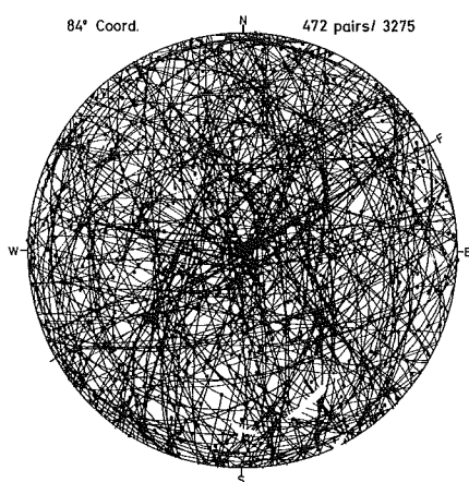
Fig. 26a Peak girdle at 84° peak in anthophyllite-cordierite-quartz-pyrite rock facies
