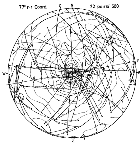
Fig. 19c Peak girdle at 77^\circ peak.
