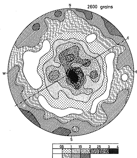
Fig. 13 A representative quartz fabric pattern of anthophyllite-cordierite-quartz-pyrite rock facies. The upper column is the concentration degree of the inner circle, the lower is one of the outer circle.
