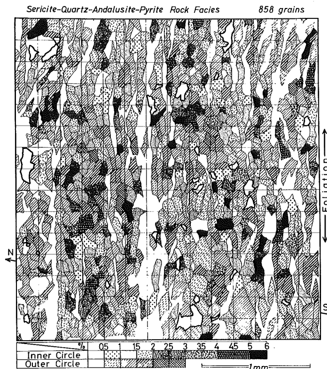
Fig. 3 A.V.A. detailed map of the squared area in Fig. 2.
