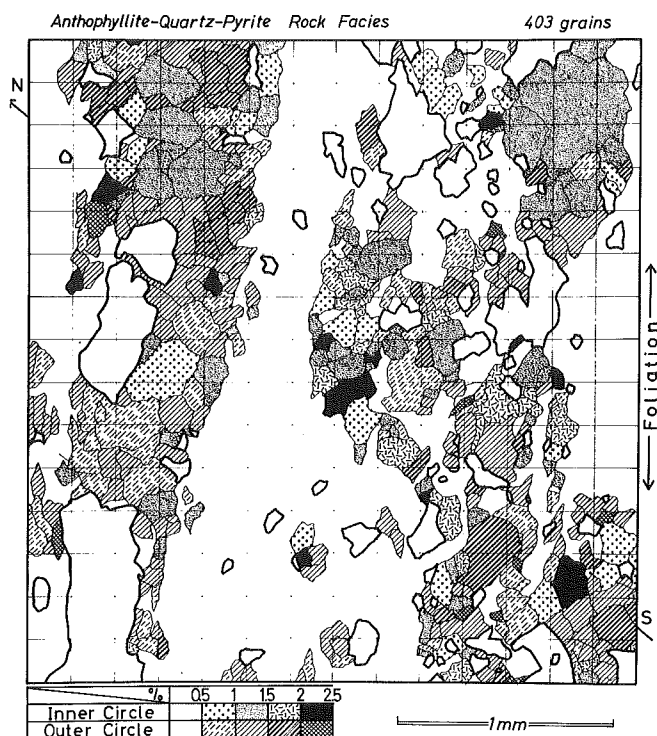
Fig. 11 A.V.A. detailed map of the squared area in Fig. 10.
