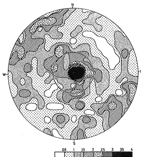
Fig. 37 An actual pattern which is statistically obtained from Fig. 36.
