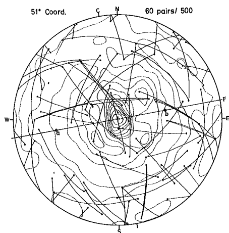
Fig. 19e Peak girdle at 51° peak.
