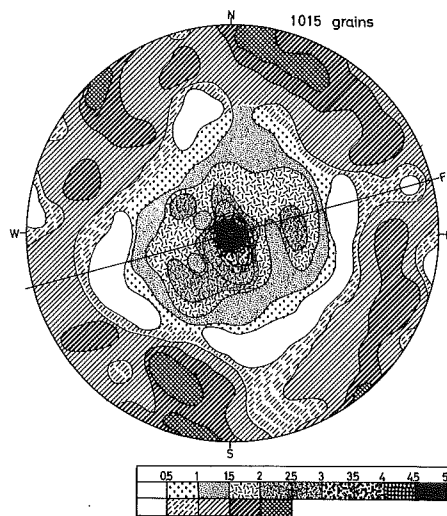
Fig. 5 A representative quartz fabric pattern of cordierite-quartz-pyrite rock facies. The upper column is the concentration degree of the inner circle, the lower is one of the outer circle.
