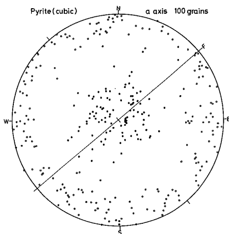
Fig. 32-(3) Pyrite fabric pattern of anthophyllite-quartz-pyrite rock facies.
