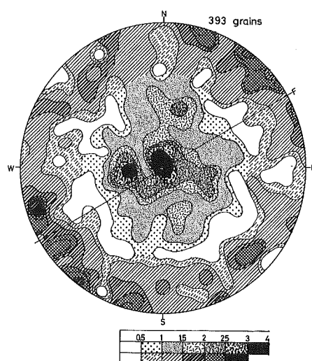
Fig. 17b Fabric pattern for fine-grained quartz facies with sulphide ore minerals in Fig. 13.
