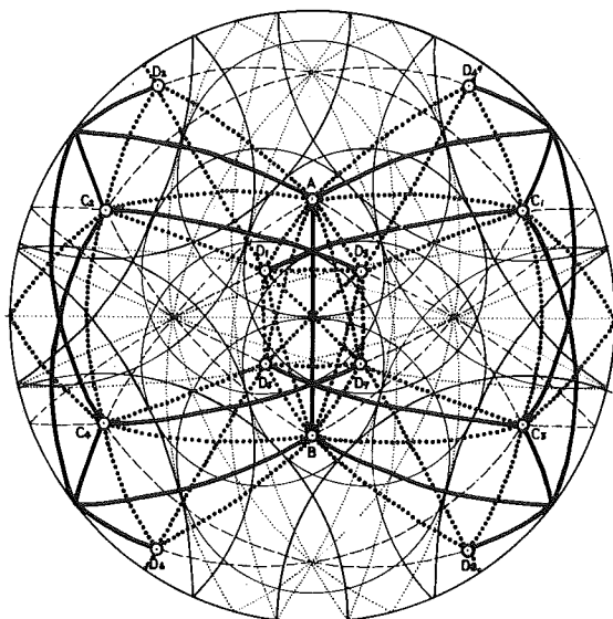
Fig. 28 Crystallographical relation of coordination after Japanese twin law for grains A, B, C and D.
