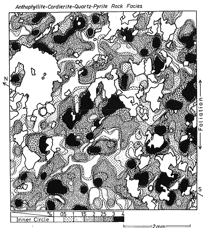
Fig. 16a A.V.A. Contour Map belonging to inner circle of Fig. 13, which is maintained by making the statistical contour lines of concentration grade in respective group.
