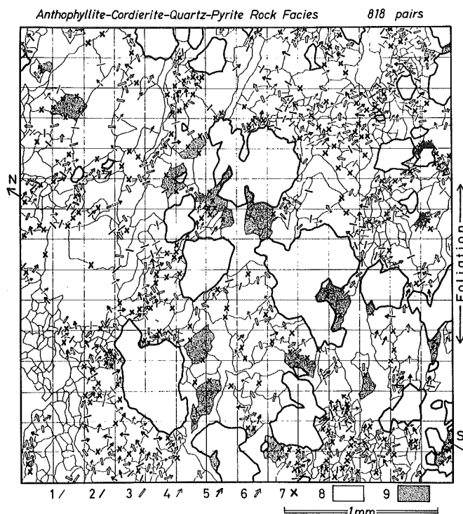
Fig. 27 Distribution Map of c -axis coordination on each concentration angle of the squared area in Fig. 14.
