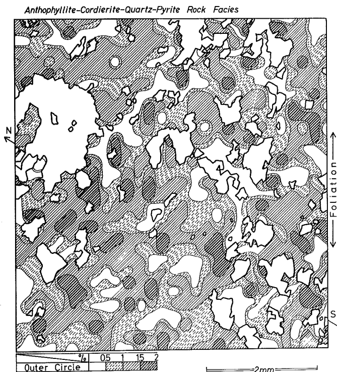
Fig. 16b A.V.A. Contour Map belonging to outer circle of Fig. 13, which is maintained by making the statistical contour lines of concentration grade in respective group.
