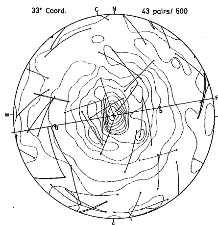
Fig. 19f Peak girdle at 33° peak.
