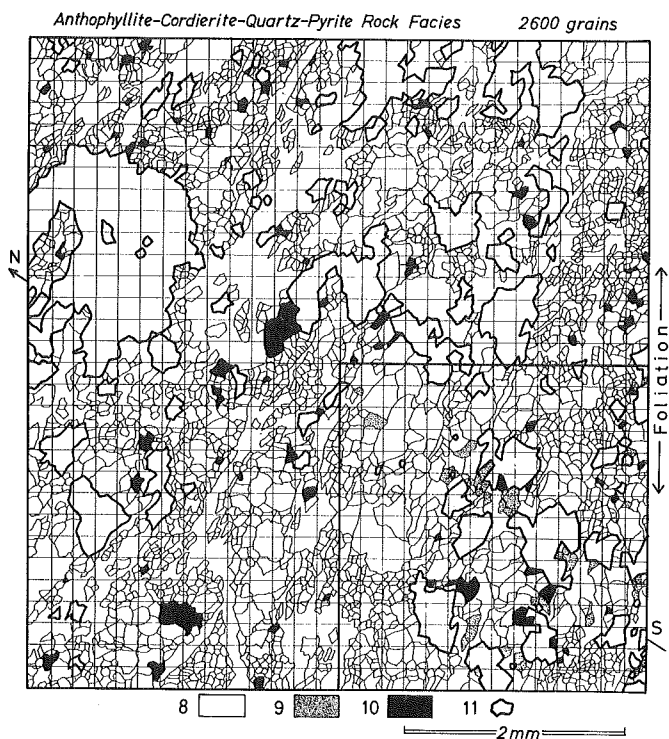
Fig. 14 A measured area in a thin section of anthophyllite-cordierite-quartz-pyrite rock facies for quartz fabric analysis. Furthermore, within a small squared area, the more detailed analyses as shown in Fig. 15 and Fig. 27 are carried out. The vacant matrix consists of plagioclase, biotite, sillimanite, perthite, chlorite and a small amount of corundum. 8: measured quartz grains with the definite coordination relation. 9: measured quartz grains without the definite coordination relation. 10: particularly, measured quartz grains plotted to the most concentrated central point of Fig. 13. 11: pyrite grains.
