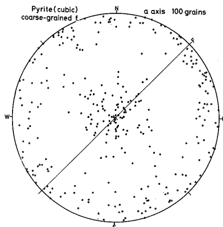
Fig. 33-(2) Pyrite fabric pattern for coarse-grained facies of pyrite ore bodies at 450 ML of the Fudotaki ore bodies.
