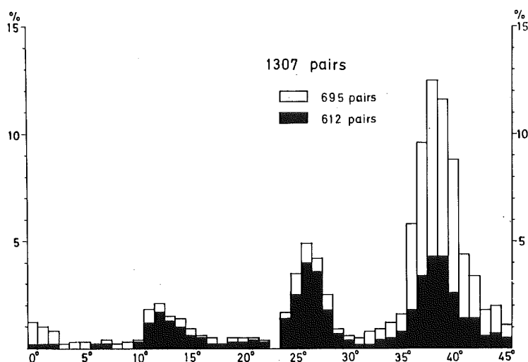
Fig. 34 A histogram of registered angles between c -axis of quartz and the pole of pyritohedral face ( c^e : framed line), or a -axis ( c^a : solid line) of pyrite in adjoining grains.
