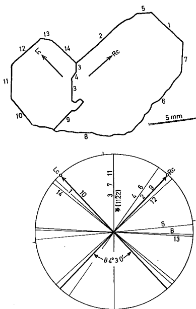
Fig. 21 Natural crystal showing the Japanese twin relation, from Narushima, Nagasaki Pref., Japan and its measured stereographic projection. The denominating numbers mean the natural crystal faces respectively. Rc and Lc denote respectively c-axis of right and left half parts of crystal.
