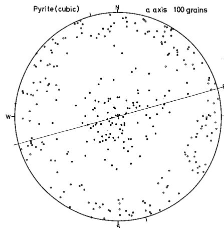
Fig. 32-(2) Pyrite fabric pattern of cordierite-quartz-pyrite rock facies.
