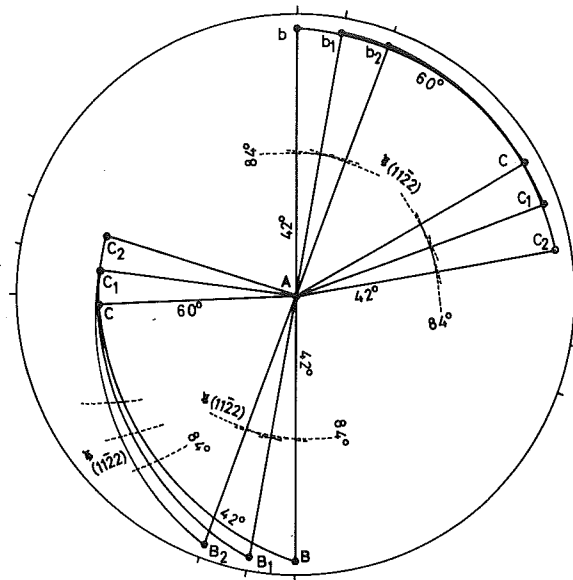
Fig. 30 A diagrammatical projection of three grains coordination after Japanese twin relation in these alteration rocks.
