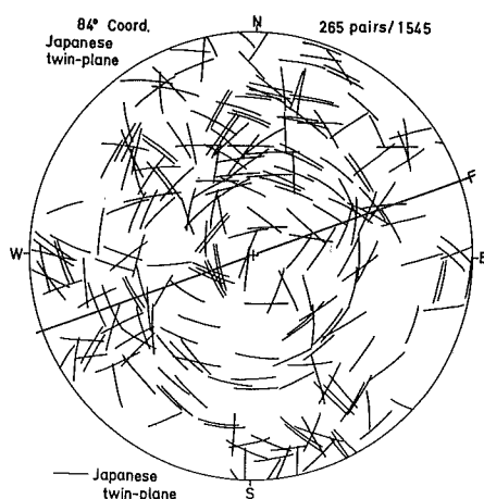
Fig. 23b A. diagram demonstrated dispositions of Japanese twin-planes from Fig. 23a.
