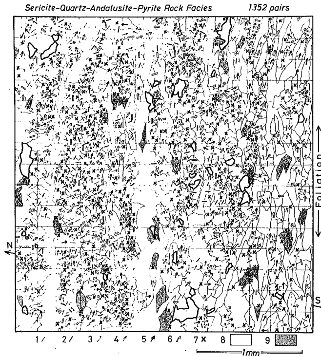
Fig. 22 Distribution Map of c -axis coordination on each concentration angle in sericite-quartz-andalusite-pyrite rock facies.
