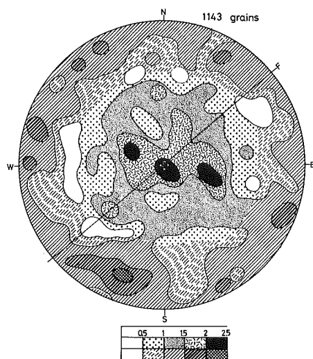
Fig. 9 A representative quartz fabric pattern of anthophyllite-quartz-pyrite rock facies. The upper column is the concentration degree of the inner circle, the lower is one of the outer circle.
