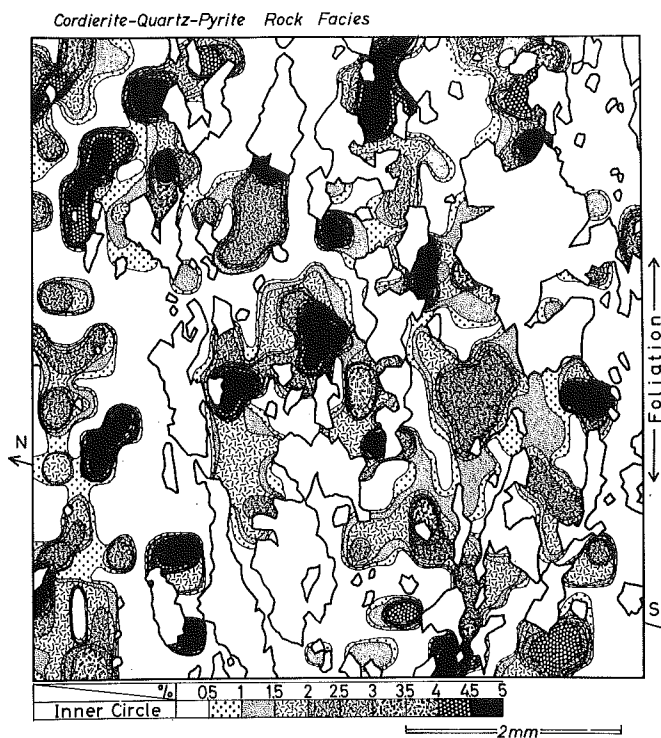
Fig. 8a A.V.A. Contour Map belonging to inner circle of Fig. 5, which is maintained by making the statistical contour lines of concentration grade in respective group.
