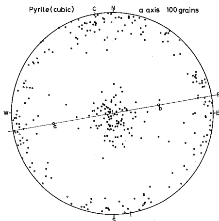
Fig. 32-(1) Pyrite fabric pattern of sericite-quartz-andalusite-pyrite rock facies.
