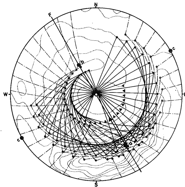
Fig. 31 Theoretical projection of three grains coordination after Japanese twin relation in the case of the Nishidohira gneiss complex (J. WATANABE, 1971).
