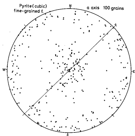
Fig. 33-(1) Pyrite fabric pattern for fine-grained facies of pyrite ore bodies at 450 ML of the Fudotaki ore bodies.
