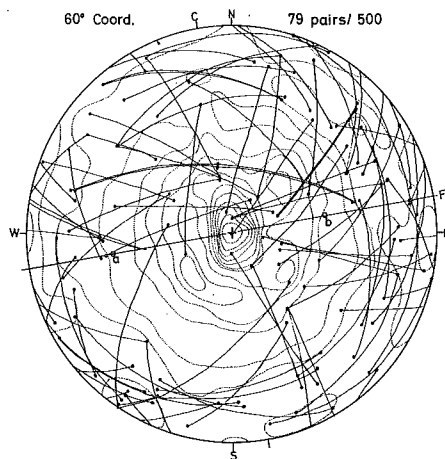
Fig. 19d Peak girdle at 60^\circ peak.
