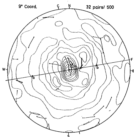
Fig. 19g Peak girdle at 9° peak.
