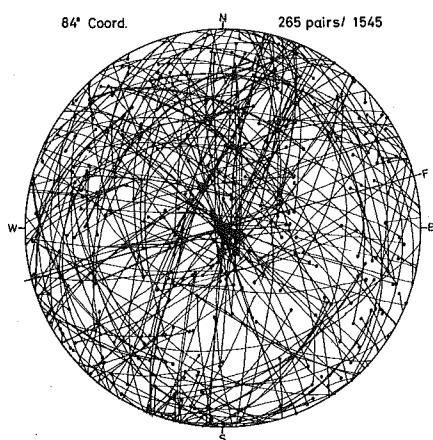
Fig. 23a Peak girdle at 84^\circ peak in cordierite-quartz-pyrite rock facies
