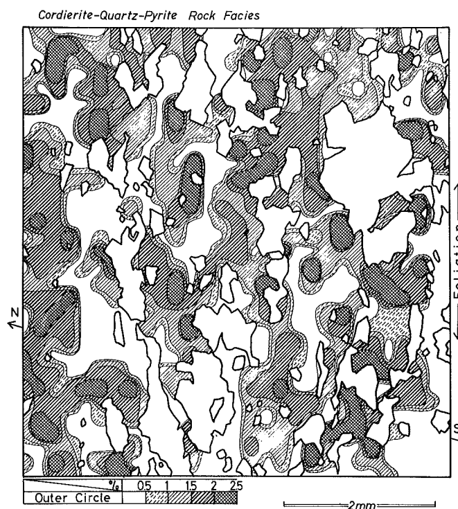
Fig. 8b A.V.A. Contour Map belonging to outer circle of Fig. 5, which is maintained by making the statistical contour lines of concentration grade in respective group.
