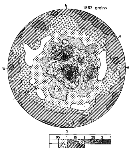
Fig. 17a Fabric pattern for fine-grained quartz facies without sulphide ore minerals in Fig. 13. The symbol marks correspond to those of Figs. 13, 16a and 16b.
