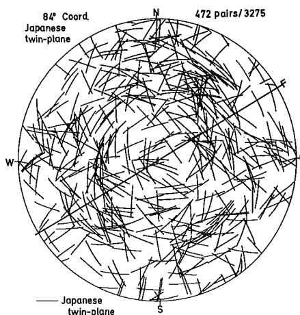
Fig. 26b A diagram demonstrated dispositions of Japanese twin-planes from Fig. 26a.
