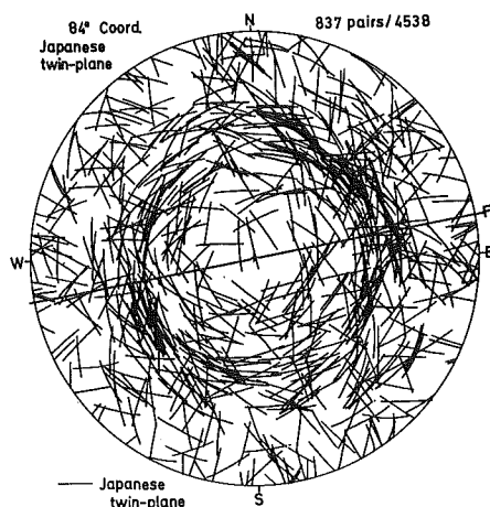
Fig. 20 A representative diagram demonstrated dispositions of Japanese twin-planes in sericite-quartz-andalusite-pyrite rock facies.
