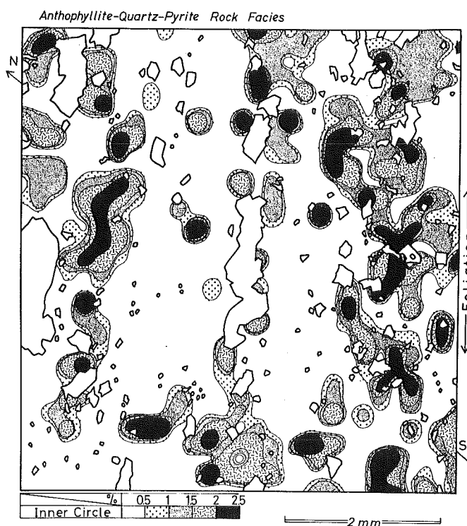
Fig. 12a A.V.A. Contour map belonging to inner circle of Fig. 9, which is maintained by making the statistical contour lines of concentration grade in respective group.
