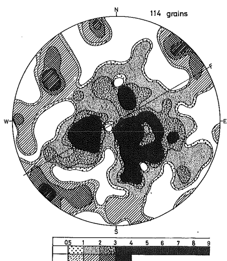
Fig. 17c Fabric pattern for coarse-grained quartz facies with sulphide ore minerals in Fig. 13.
