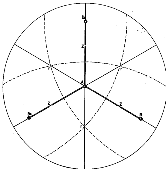
Fig. 29 Crystallographical relation of coordination by r(10\bar{1}1) .
