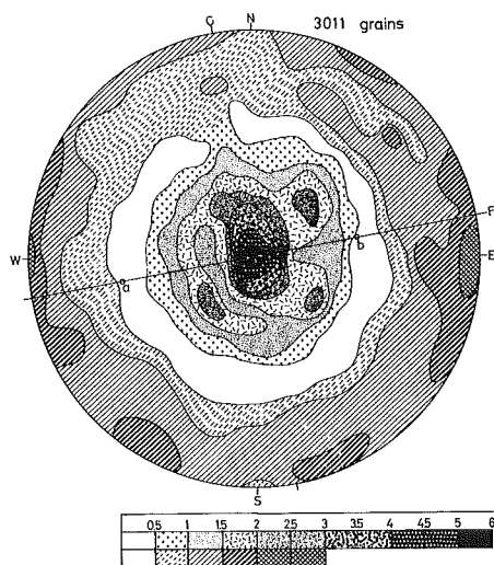
Fig. 1 A representative quartz fabric pattern of sericite-quartz-andalusite-pyrite rock facies. F is the foliation plane, a, b and c are of fabric axis. The upper column is the concentration degree of the inner circle, the lower is one of the outer circle.
