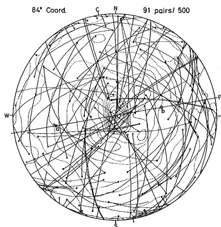
Fig. 19b Peak girdle at 84^\circ peak.
