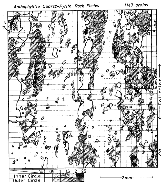
Fig. 10 A measured area in a thin section of anthophyllite-quartz-pyrite rock facies for quartz fabric analysis and A.V.A. detailed map. Furthermore, within a small squared area, the more detailed analyses as shown in Fig. 11 and Fig. 25 are carried out. The vacant matrix consists of anthophyllite, plagioclase, biotite, chlorite, a small amount of cordierite and sillimanite.
