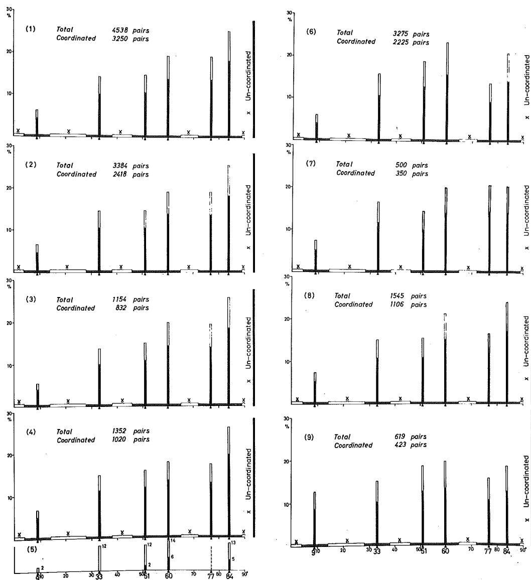
Fig. 18 Distribution and frequency diagrams for c -axis angle of the adjoining quartz grains in each rock facies.
