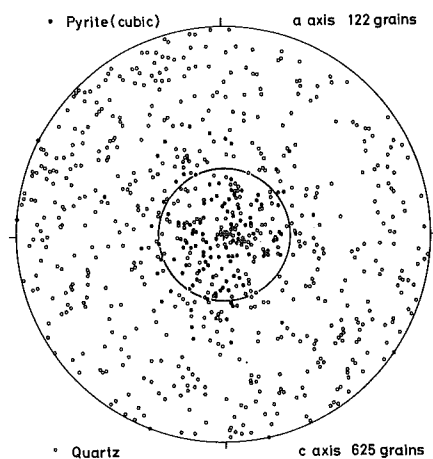
Fig. 36 An actual pattern obtained from the measured pyrite and quartz, based on Fig. 35. On Schmidt net. Small circle implies a locus of pyritohedral face around cube a(001) of the central position theoretically.
