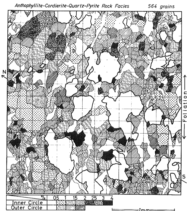
Fig. 15 A.V.A. detailed map of the squared area in Fig. 14.
