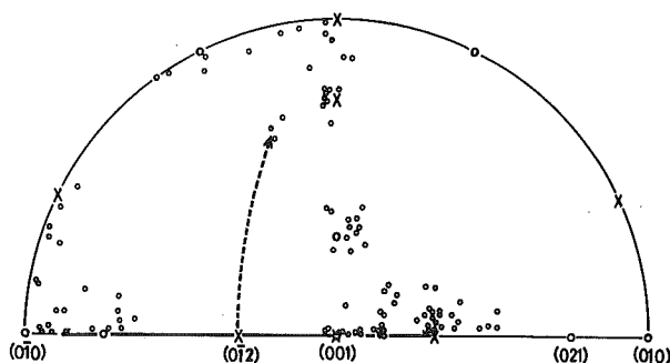
Fig. 38 An actual diagram which one hundred examples of quartz grains from Fig. 36 are exactly rearranged on cube a(001) or pyritohedral face e(012) of Fig. 35. On the northern hemisphere of Schmidt net.
