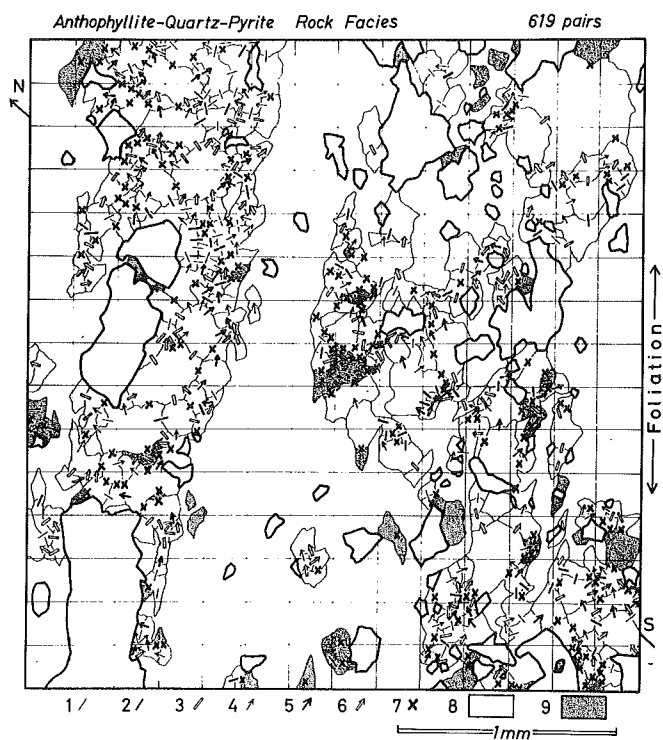
Fig. 25 Distribution Map of c -axis coordination on each concentration angle of the squared area in Fig. 10.
