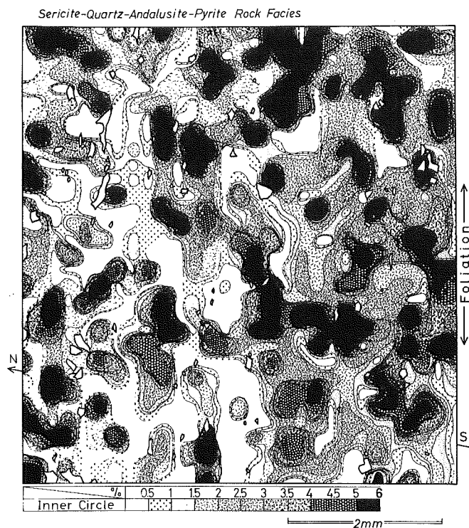
Fig. 4a A.V.A. Contour Map belonging to inner circle of Fig. 1, which is maintained by making the statistical contour lines of concentration grade in respective group.
