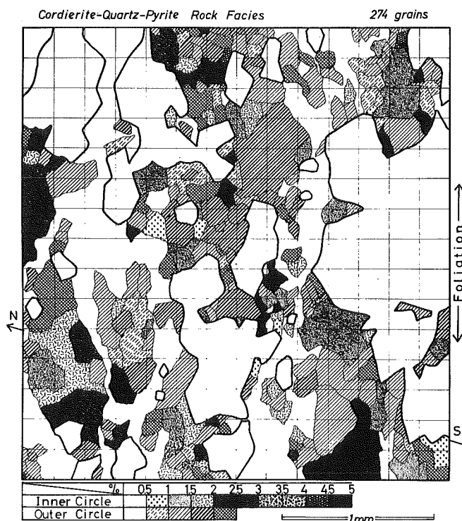
Fig. 7 A.V.A. detailed map of the squared area in Fig. 6.
