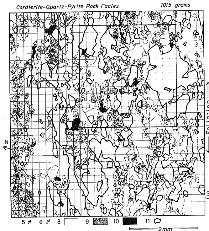
Fig. 6 A measured area in a thin section of cordierite-quartz-pyrite rock facies for quartz fabric analysis. Furthermore, within a small squared area, the more detailed analyses as shown in Fig. 7 and Fig. 24 are carried out. The vacant matrix consists of plagioclase, chlorite and a small amount of anthophyllite. 5: coordination relation at 77^\circ . 6: coordination relation at 84^\circ . 8: measured quartz grains with the definite coordination relation. 9: measured quartz grains without the definite coordination relation. 10: measured quartz grains disposed at the most concentrated central point in Fig. 5. 11: pyrite grains.
