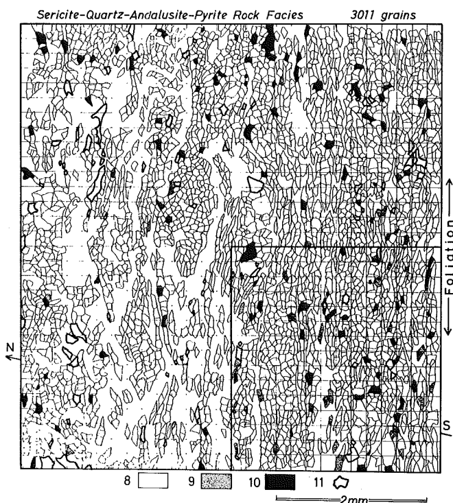
Fig. 2 A measured area in a thin section of sericite-quartz-andalusite-pyrite rock facies for quartz fabric analysis. Furthermore, within a small squared area the more detailed analyses as shown in Fig. 3 and Fig. 22 are carried out. The vacant matrix consists of sericite, plagioclase, and andalusite. 8: measured quartz grains with the definite coordination relation. 9: measured quartz grains without the definite coordination relation. 10: particularly, measured quartz grains plotted to the most concentrated central point of Fig. 1. 11: pyrite grains.
