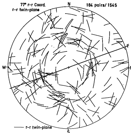
Fig. 23d A diagram demonstrated dispositions of Estérel twin-planes from Fig. 23c.
