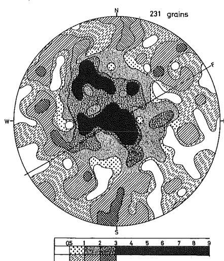
Fig. 17d Fabric pattern for coarse-grained quartz facies without sulphide ore minerals in Fig. 13.
