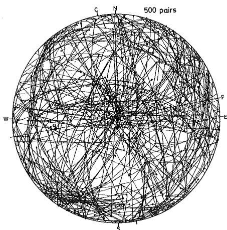
Fig. 19a Peak girdle of 500 pairs of c -axis angles of the adjoining quartz grains of sericite-quartz-andalusite-pyrite rock facies.
