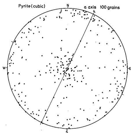
Fig. 33-(3) Pyrite fabric pattern of another pyrite ore bodies at 450 ML of the Fudotaki ore bodies.
