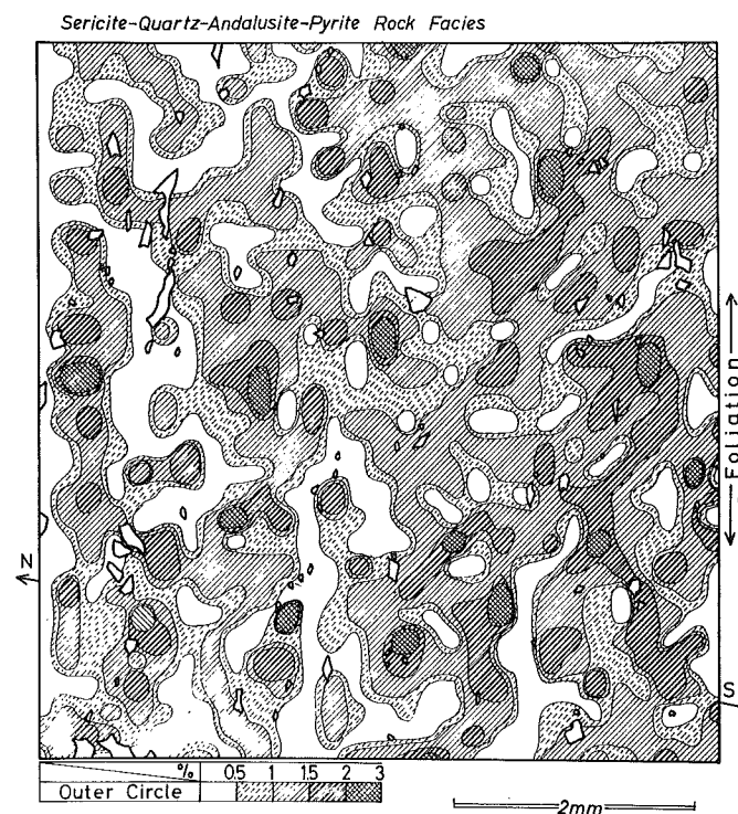
Fig. 4b A.V.A. Contour Map belonging to outer circle of Fig. 1, which is maintained by making the statistical contour lines of concentration grade in respective group.
