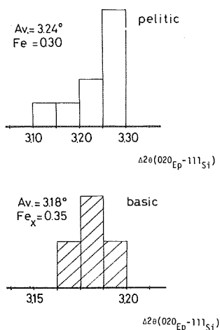
Fig. 6. \Delta 2\theta(020_{Ep}-111_{Si}) values for epidote in basic and pelitic rocks of Zone III.
