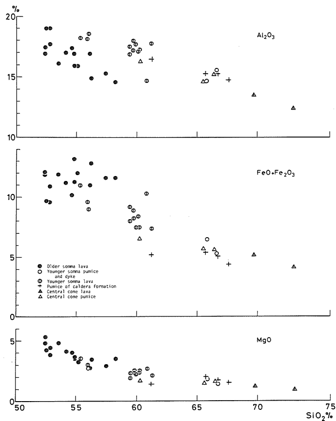
Fig. 7 \text{Al}_2\text{O}_3 , \text{FeO} + \text{Fe}_2\text{O}_3 , and \text{MgO} versus \text{SiO}_2 for the Mashu rocks.
