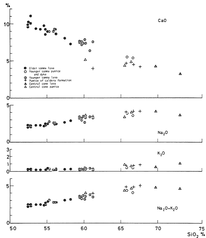
Fig. 8 \text{CaO} , \text{Na}_2\text{O} , \text{K}_2\text{O} and \text{Na}_2\text{O} + \text{K}_2\text{O} versus \text{SiO}_2 for the Mashu rocks.
