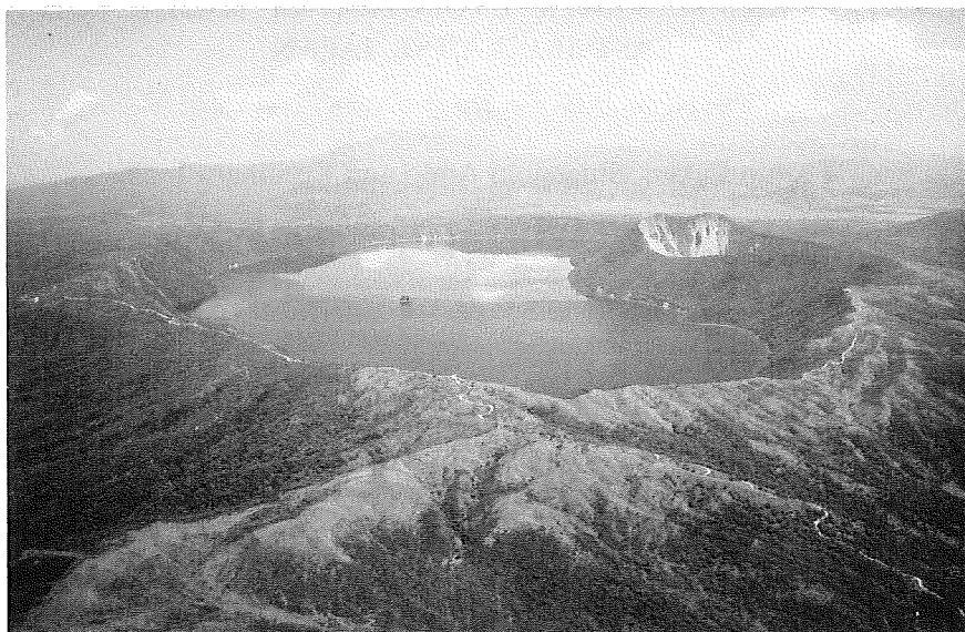
Fig. 1 The Mashu caldera, east Hokkaido, viewed from southwest. Two post-caldera volcanoes are seen; the Kamuishu lava dome at the center, and the Kamuinupuri cone with a large crater on the right.
