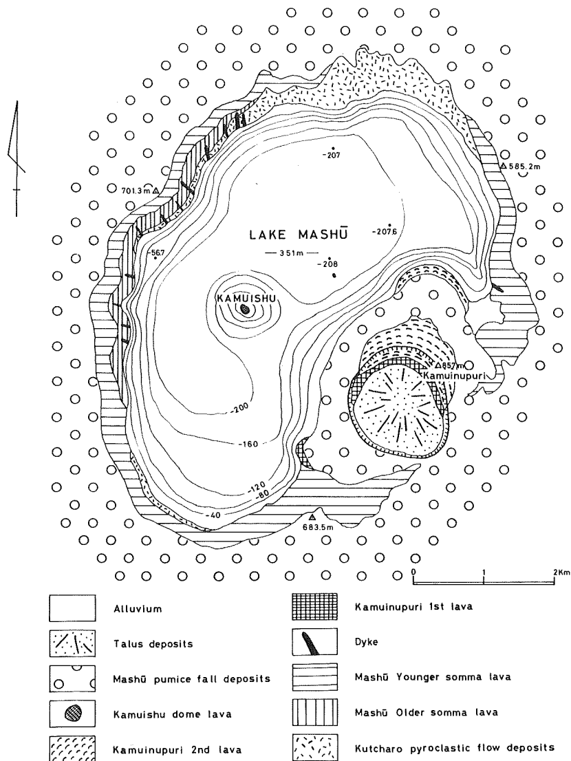
Fig. 4 Geologic map of Mashu volcano, east Hokkaido.
