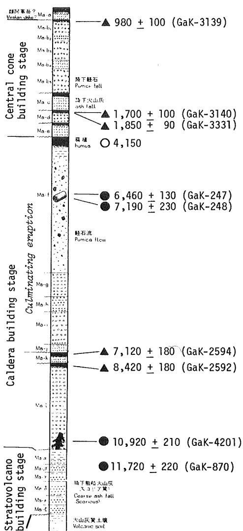
Fig. 6 Standard columnar section and radiocarbon dates of the Mashu pyroclastic deposits. Materials for radiocarbon age determination: solid circles — charcoal, and solid triangles — humic acid. An obsidian hydration date of stone implements is shown by open circle. Source of data: Katsui, 1963; Katsui and Kondo, 1965; Satoh, 1969; Sasaki et al, 1971; Shoji and Masui, 1974.
