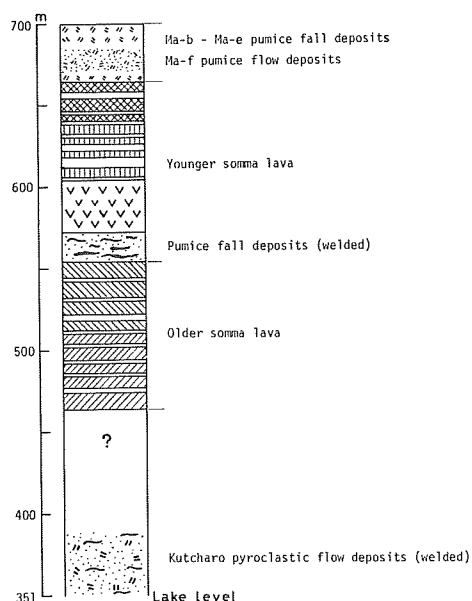
Fig. 5 A columnar section at the northwestern part of the Mashu caldera.
