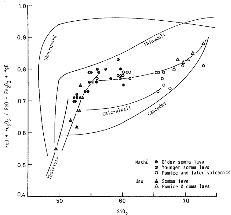
Fig. 11 \text{FeO}+\text{Fe}_2\text{O}_3 / \text{FeO}+\text{Fe}_2\text{O}_3+\text{MgO} – silica diagram for the rocks of Mashu and Usu. Data of Usu given by Oba (1966) and the trends of other rock suites by Carmichael (1964).
