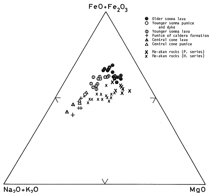
Fig. 9 Triangular variation diagram for \text{MgO} - \text{FeO} + \text{Fe}_2\text{O}_3 - \text{Na}_2\text{O} + \text{K}_2\text{O} . The data of the Me-akan rocks are mainly given by S. Ando (unpublished).
