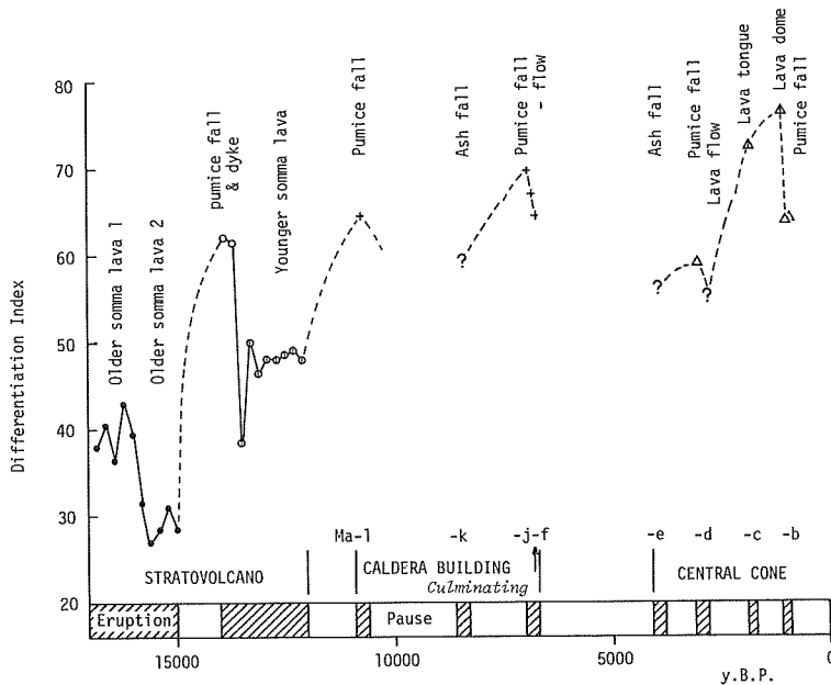
Fig. 10 Chronological arrangement of the Mashu volcanic products plotted against their differentiation index (D.I.). Data for the stratovolcano building stage are based on the samples which were systematically collected from the northwestern part of the Mashu caldera wall.
