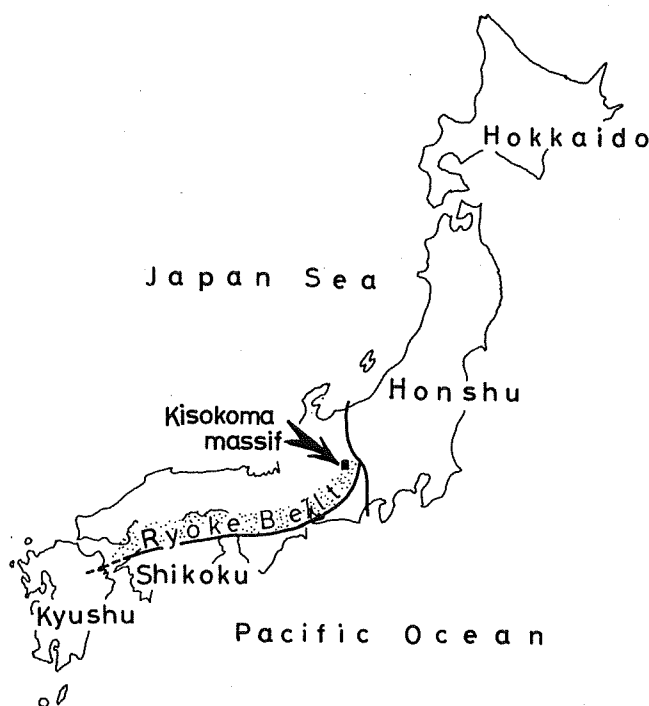
Fig. 1. Index map of the Kisokoma massif.
