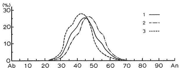
Fig. 15. An-frequency curves based on unit range \pm 2.5\text{An}\% of the biotite plagioclase porphyritic enclaves. 1. Total 2. Core 3. Mantle
