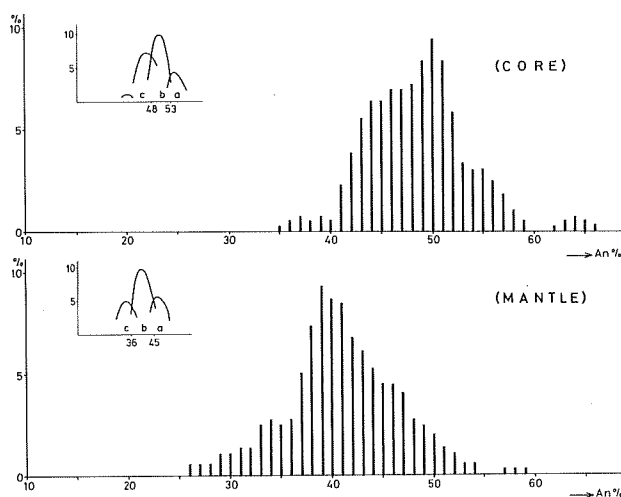
Fig. 10. An-frequency histograms based on unit range \pm 1.5\text{An}\% of the melanocratic fine-grained enclaves.
