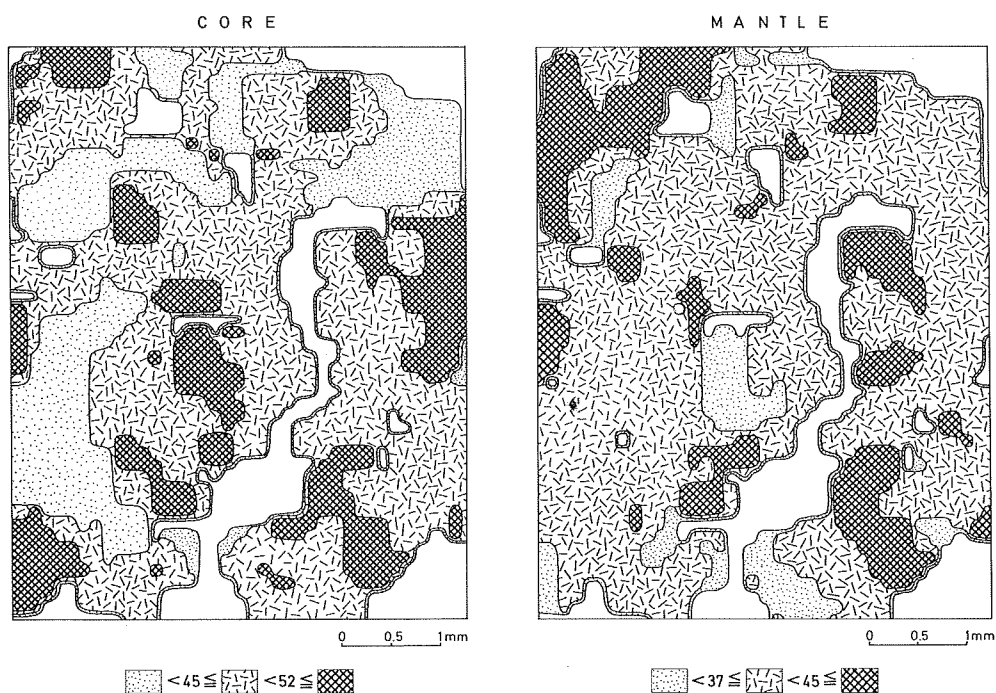
Fig. 17. Two-dimensional distribution maps of An-content of the biotite plagioclase porphyritic enclaves by statistical contouring. Unit area is 0.1 \text{ mm}^2 .
