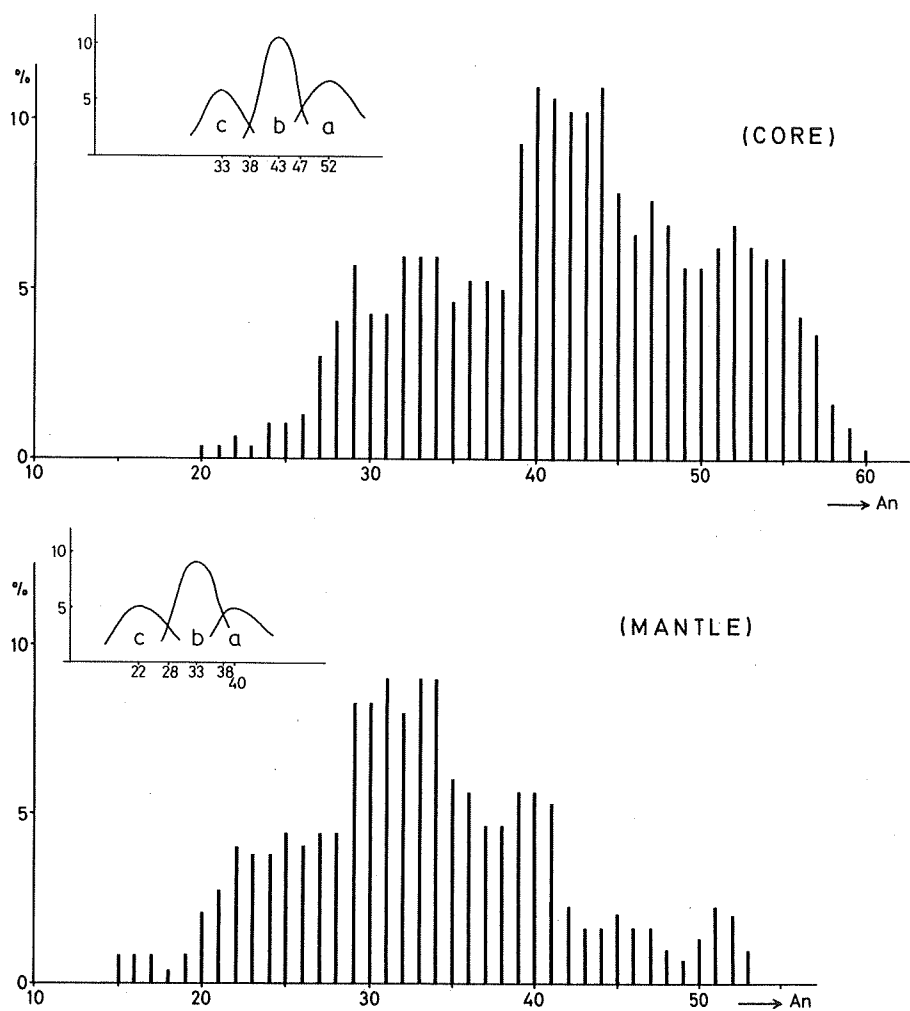
Fig. 6. An-frequency histograms based on unit range \pm 1.5\text{An}\% of the granodiorite III.
