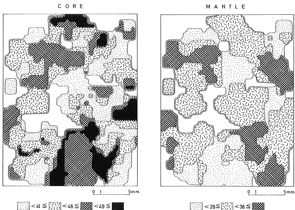
Fig. 26. Two-dimensional distribution maps of An-content of the granodiorite IV by statistical contouring. Unit area is 0.1 \text{ mm}^2 .
