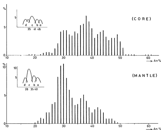
Fig. 13. An-frequency histograms based on unit range \pm 1.5\text{An}\% of the biotite porphyritic enclaves.
