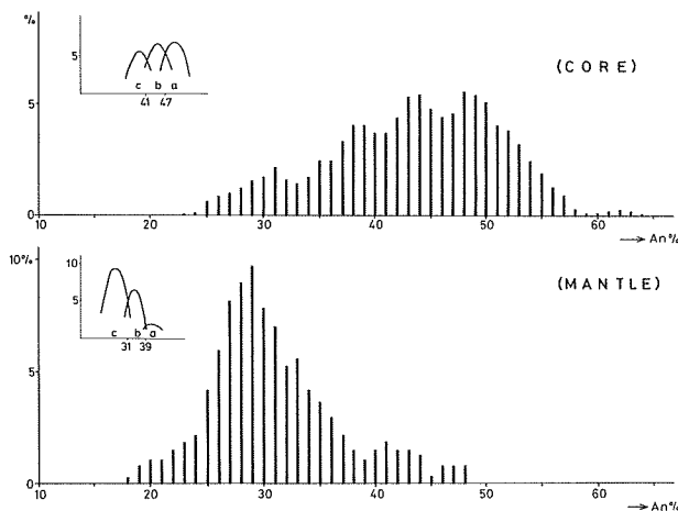
Fig. 22. An-frequency histograms based on unit range \pm 1.5\text{An}\% of the granodiorite II.
