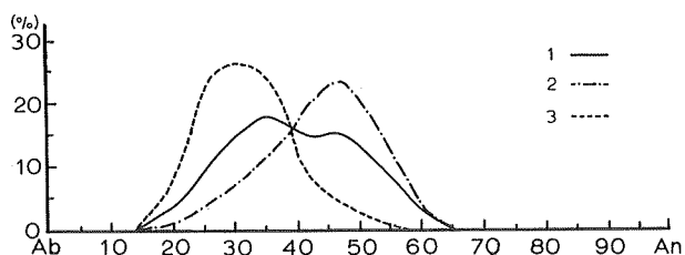
Fig. 21. An-frequency curves based on unit range \pm 2.5\text{An}\% of the granodiorite II. 1. Total 2. Core 3. Mantle
