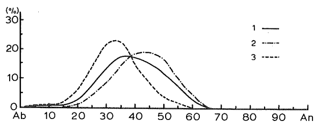
Fig. 5. An-frequency curves based on unit range \pm 2.5\text{An}\% of the granodiorite III. 1. Total 2. Core 3. Mantle
