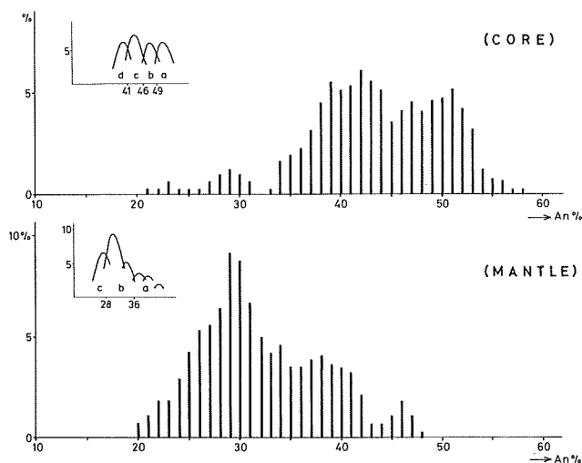
Fig. 25. An-frequency histograms based on unit range \pm 1.5\text{An}\% of the granodiorite IV.
