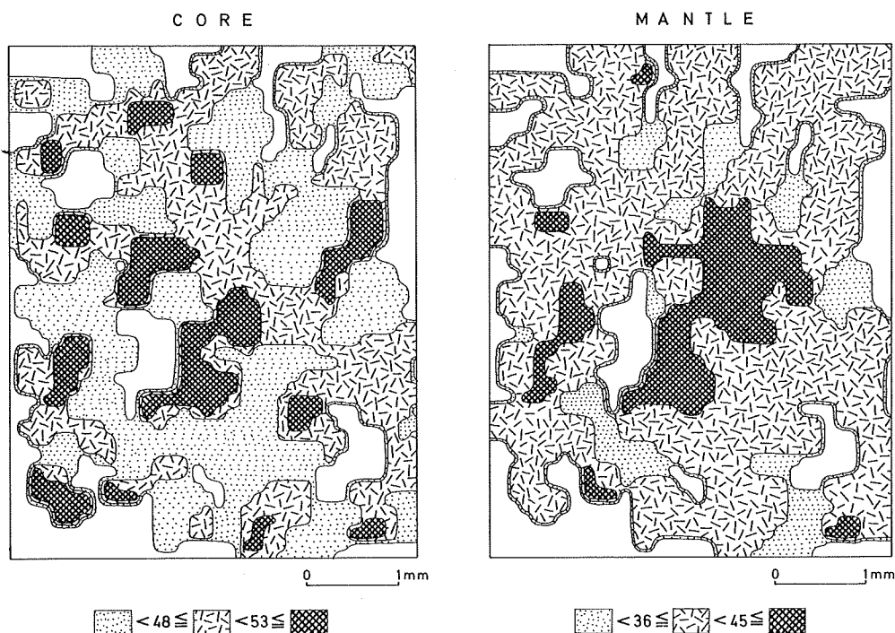
Fig. 11. Two-dimensional distribution maps of An-content of the melanocratic fine-grained enclaves by statistical contouring. Unit area is 0.1 \text{ mm}^2 .
