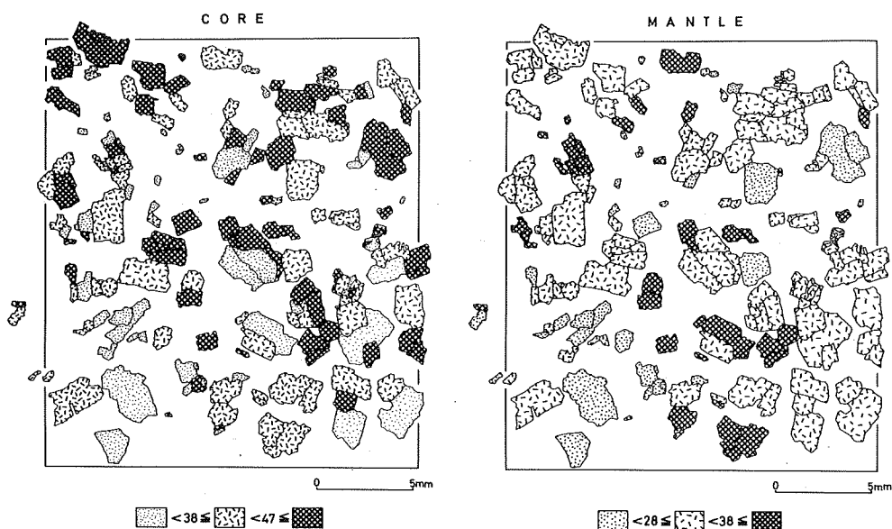
Fig. 7. Sketches of the thin section showing the plagioclases and their An-content of the granodiorite III. The vacant spaces are occupied by minerals other than plagioclase. The subdivisions correspond to the group a, b and c designated in Fig. 6.
