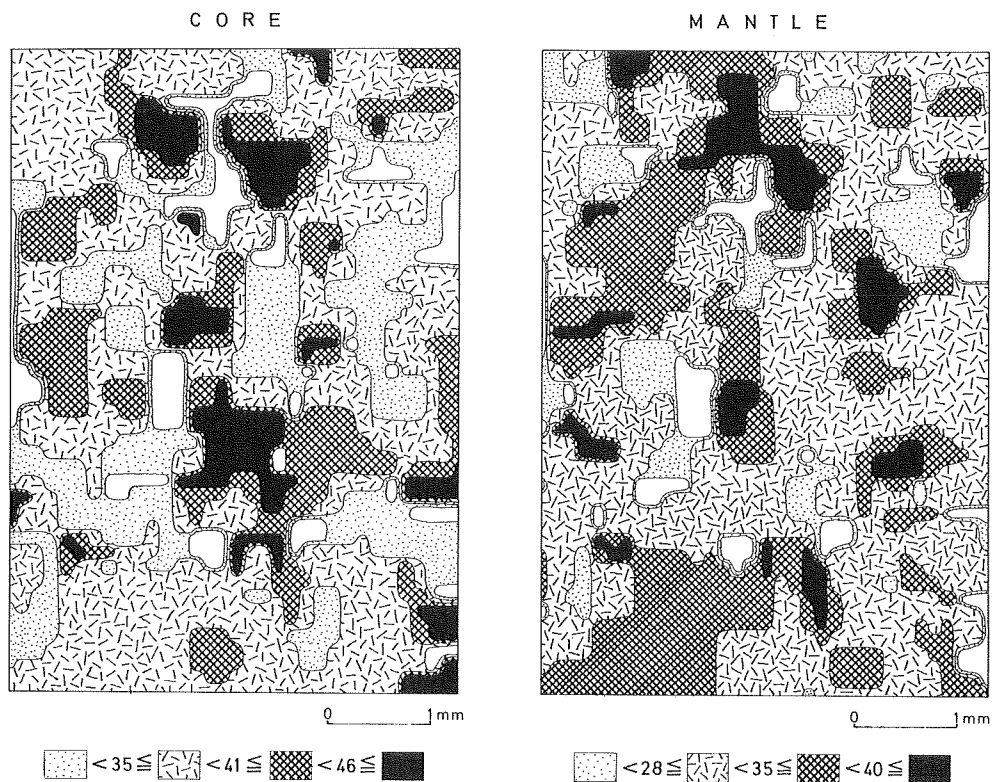
Fig. 14. Two-dimensional distribution maps of the biotite porphyritic enclaves by statistical contouring. Unit range is 0.1 \text{ mm}^2 .
