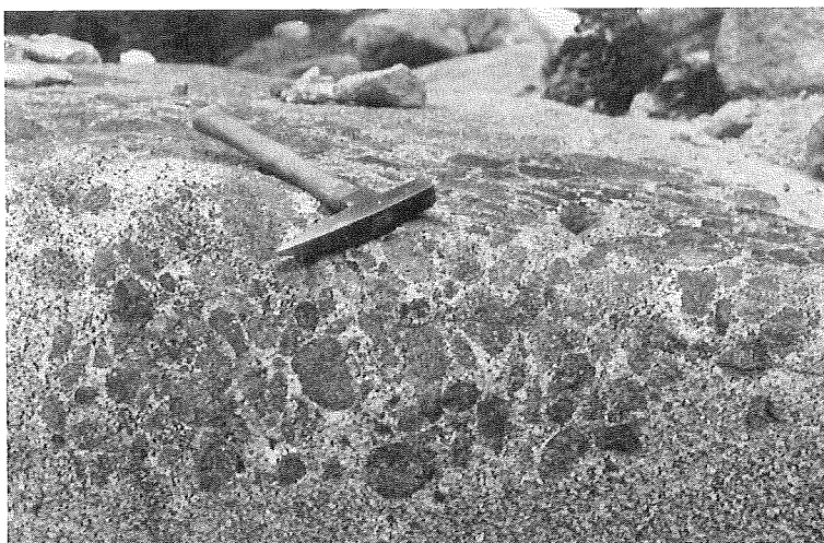
Fig. 3. An outcrop showing a layer of aggregated numerous basic enclaves. From the river Shozawa.
