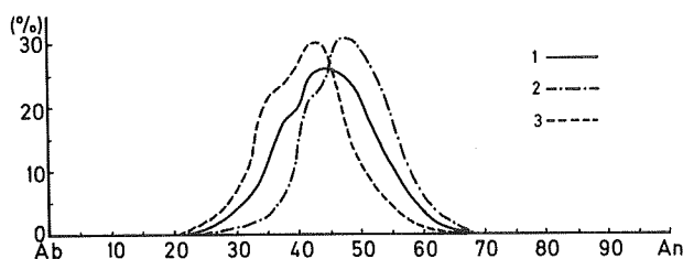
Fig. 9. An-frequency curves based on unit range \pm 2.5\text{An}\% of the melanocratic fine-grained enclaves. 1. Total 2. Core 3. Mantle
