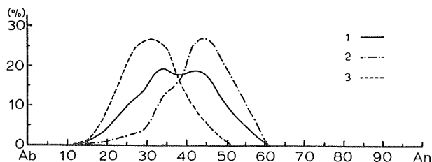
Fig. 24. An-frequency curves based on unit range \pm 2.5\text{An}\% of the granodiorite IV. 1. Total 2. Core 3. Mantle
