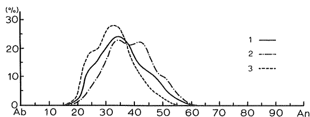
Fig 12. An-frequency curves based on unit range \pm 2.5\text{An}\% of the biotite porphyritic enclaves.
