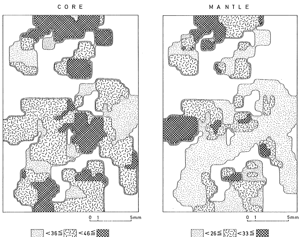
Fig. 20. Two-dimensional distribution maps of An-content of the granodiorite I by statistical contouring. Unit area is 0.1 \text{ mm}^2 .
