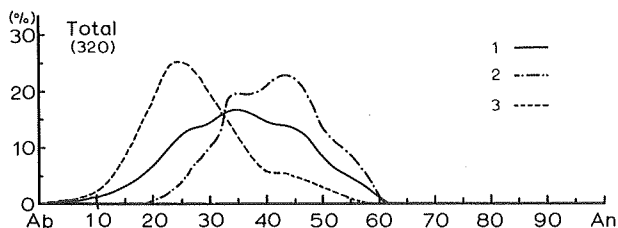
Fig. 18. An-frequency curves based on unit range \pm 2.5 \text{ An\%} of the granodiorite I. 1. Total 2. Core 3. Mantle
