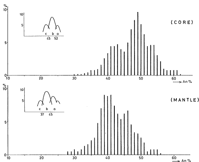
Fig. 16. An-frequency histograms based on unit range \pm 1.5\text{An}\% of the biotite plagioclase porphyritic enclaves.
