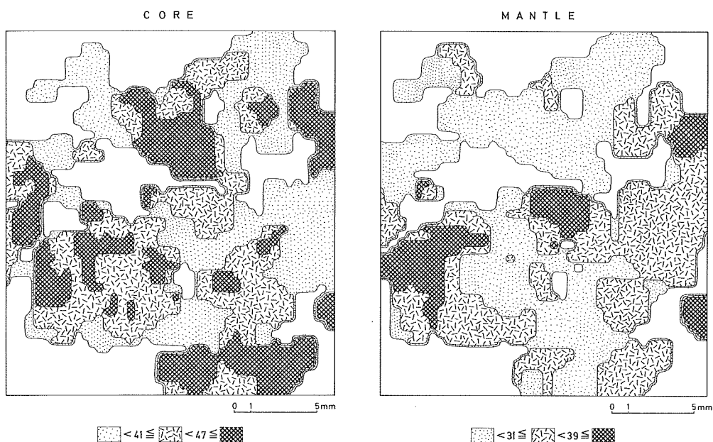
Fig. 23. Two-dimensional distribution maps of An-content of the granodiorite II by statistical contouring. Unit area is 0.1 \text{ mm}^2 .
