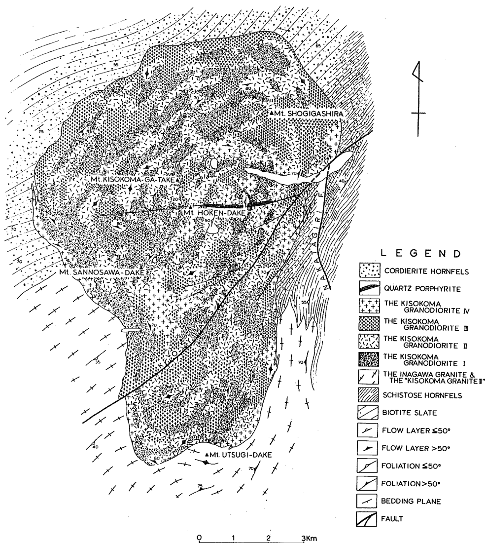
Fig. 2. Lithofacies map of the Kisokoma massif.
