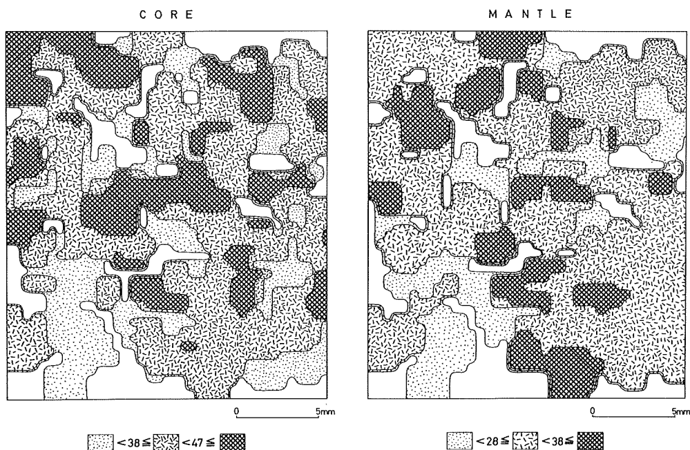
Fig. 8. Two-dimensional distribution maps of An-content of the granodiorite III by statistical contouring. Unit area is 0.1\text{mm}^2 .
