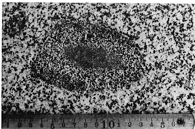
Fig 4. Zoned basic enclave showing the sequence of metasomatic process. The core represents the melanocratic fine-grained lithofacies and the mantle shows the biotite plagioclase porphyritic lithofacies.
