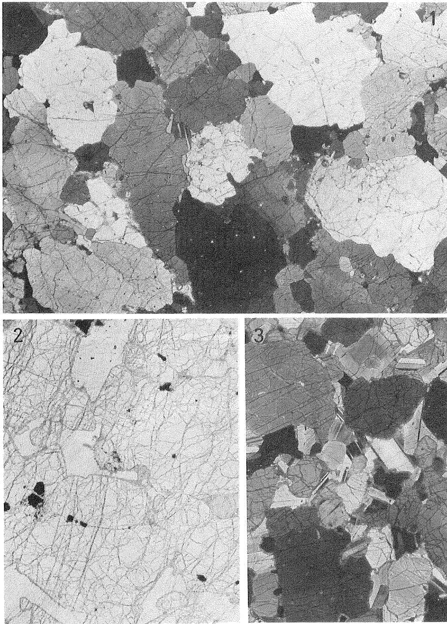
Plate 8: Fig. 1. Olivine mesocumulate of olivine-rich layers of the Lower Zone. The amount of intercumulus plagioclase is very small. X 10.
