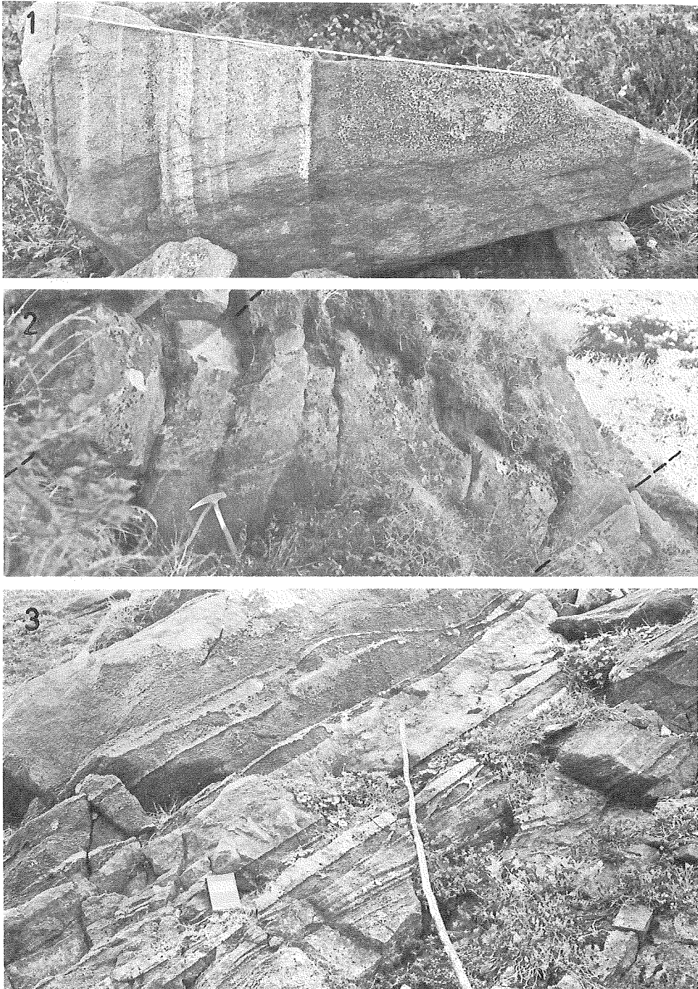
Plate 3: Fig. 1. Well developed example of finely stratified layering from the Lower Zone of the Poroshiri part.
