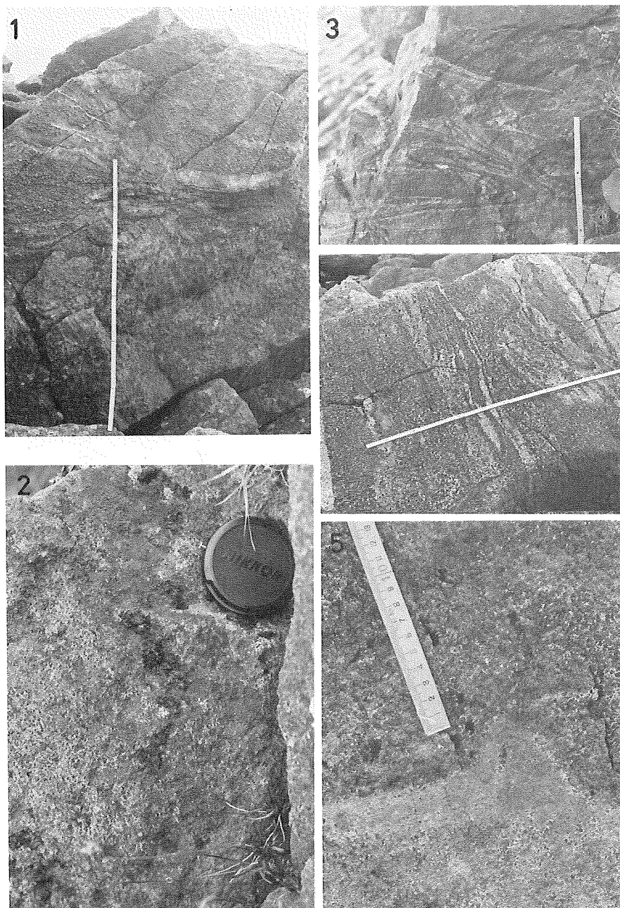
Plate 4: Fig. 1. Disturbed structure in plagioclase-rich macro layer of the Lower Zone of the Poroshiri part. Scale is 1m.
