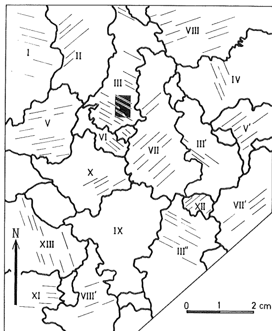
Fig. 2 Domain structure with closely packed porphyroblasts. (Analogues to Fig. 1). Schematic shading within the domains indicates the direction of edges common to two intersecting surfaces; the polished surface of the material and the natural crystal surface bounding "pits" equivalent to an e-face. The rectangle in domain "III" is the area of the photomicrograph (Fig. 4a).
