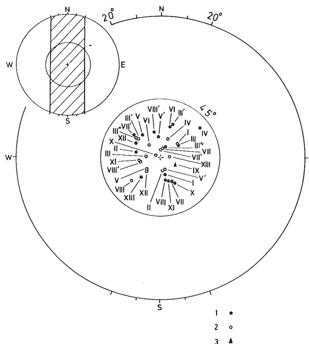
Fig. 6 A diagram showing orientation of boundary "pits" of pyrite in each domain. Roman numerals are comparable to those in Fig. 2. 1: measured e(210) pole, 2: calculated a-axis, 3: measured a-axis.
