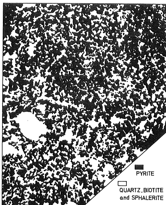
Fig. 1 A typical sample of pyrite ores forming porphyroblastic domains. Carefully oriented samples have been used to make the polished sections. (Loc. 2F 850ML)
