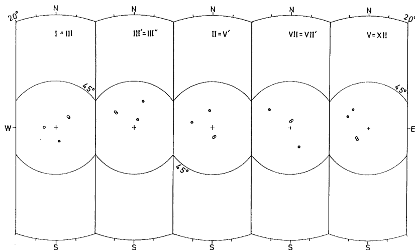
Fig. 7 Nearly parallel disposition of domains, represented by the orientation of measured e-face poles (solid circle) and calculated a-axes (open circle). Roman letters are the number of domain in Fig. 2.
