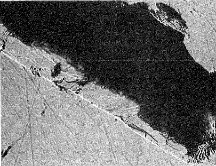
Fig. 4d Even greater enlargement of the same area of Fig. 4c, showing layering-growth hillocks (Interference contrast by Nomarski method). X 710
