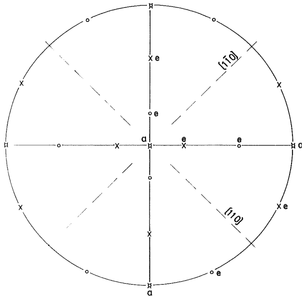
Fig. 5 Estimation of the symmetrical component of pyrite deduced from the actual measurement. e: pyritohedral face, a: cube face. [110] and [1\bar{1}0] are twin axes (broken lines) of so-called Iron Cross Twin of pyrite. This diagram includes two sets of component faces after twin disposition (open circle and cross). Solid line: a-face.
