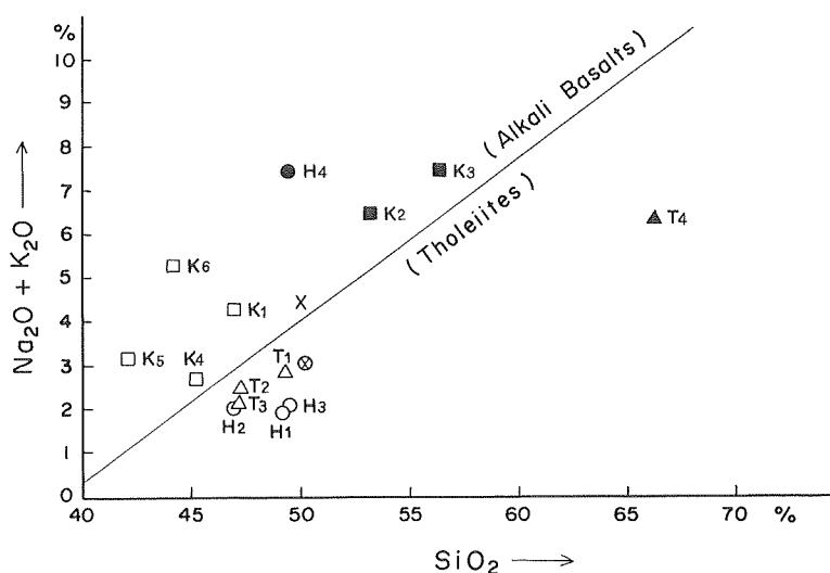
Fig. 2 Alkali-silica diagram for pillow lava rocks from the central axial zone of Hokkaido. Heavy line is Hawaii alkalic-tholeiitic division line, as defined by Macdonald and Katsura (1964)
