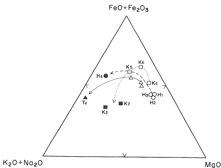
Fig. 3 FMA diagram showing pillow lavas from the Tokoro Belt, the Hidaka Belt and the Kamuikotan Belt, central axial zone of Hokkaido
