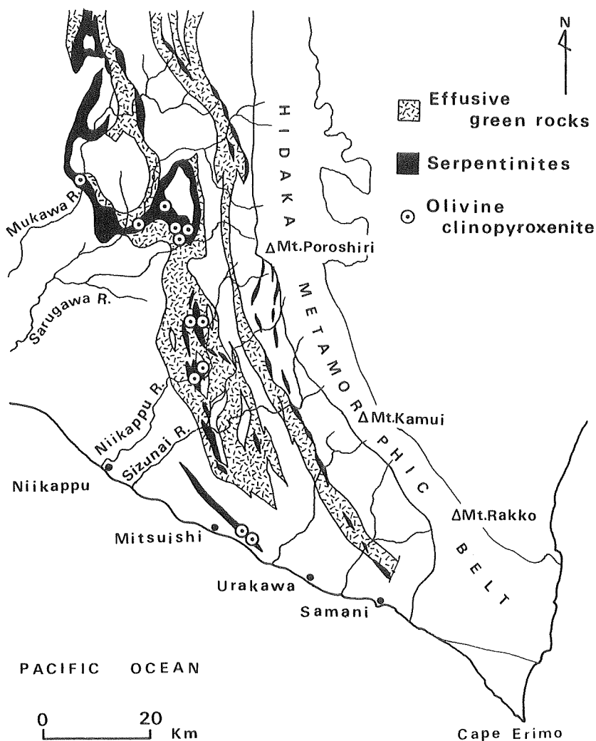
Fig. 1 Localities of olivine clinopyroxenite in serpentinite bodies of the Kamukotan Zone.
