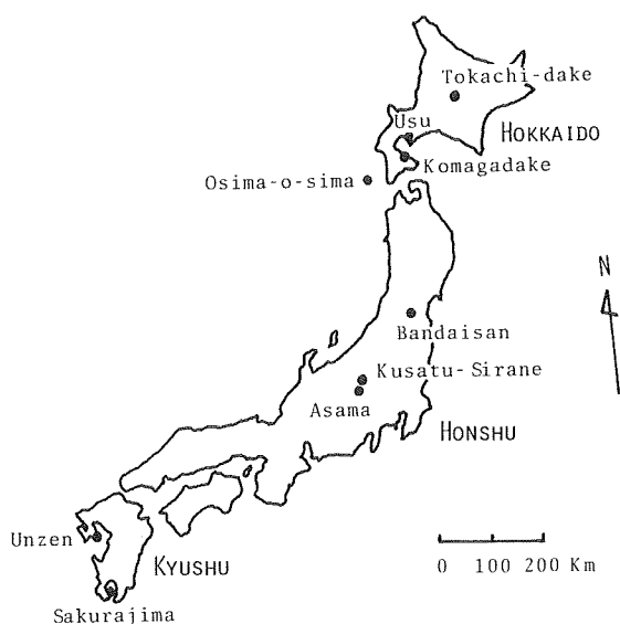
Fig. 1 Japanese Main Islands, indicating localities of volcanoes included in studies.
