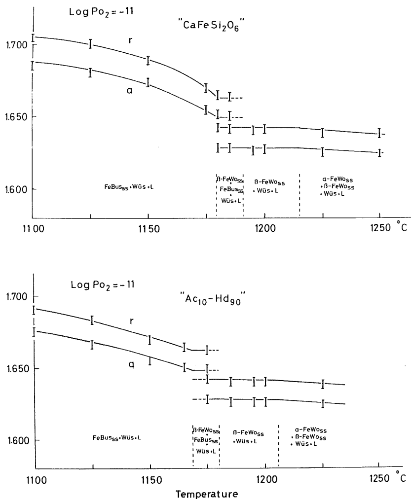
Fig. 3 Change of refractive indices of \beta\text{-Fe-wollastonite}_{\text{ss}} and \text{Fe-bustamite}_{\text{ss}} crystallized from the compositions of \text{CaFe}^{2+}\text{Si}_2\text{O}_6 and \text{Ac}_{10}\text{Hd}_{90} at 10^{-11} atm f_{\text{O}_2} . Abbreviations are same as in Fig. 1.
