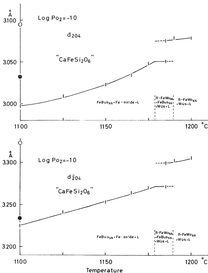
Fig. 2 Change of d-spacings of \beta -Fe-wollastonite ss and Fe-bustamite ss crystallized from the composition \text{CaFe}^{2+}\text{Si}_2\text{O}_6 at 10^{-10} atm f_{\text{O}_2} . The open circles represent d_{210} and d_{102} of \beta -wollastonite and the solid circles d_{204} and d_{204}^- of bustamite. Abbreviations are same as in Fig. 1.
