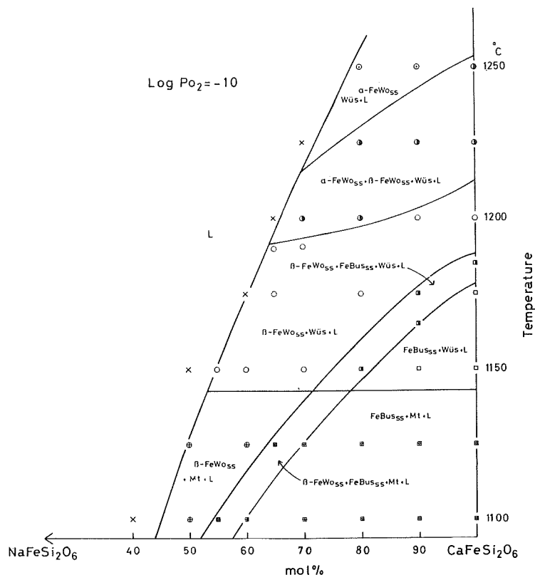
Fig. 7 Phase diagram of the system \text{NaFe}^{3+}\text{Si}_2\text{O}_6 - \text{CaFe}^{2+}\text{Si}_2\text{O}_6 at 10^{-10} atm f_{O_2} . Abbreviations are given in Fig. 1.
