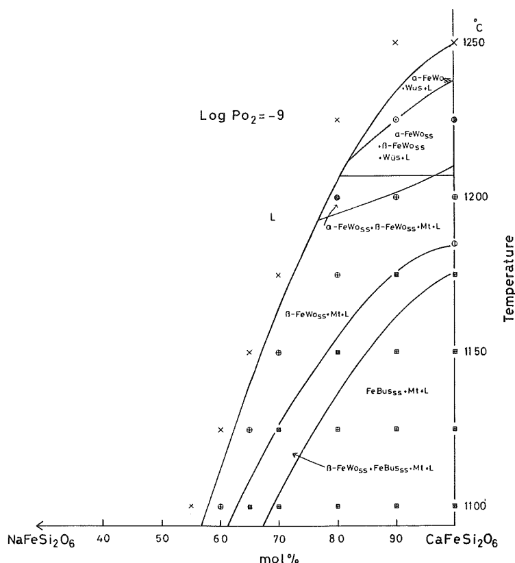
Fig. 8 Phase diagram of the system \text{NaFe}^{3+}\text{Si}_2\text{O}_6 - \text{CaFe}^{2+}\text{Si}_2\text{O}_6 at 10^{-9} atm f_{O_2} . Abbreviations are given in fig. 1.
