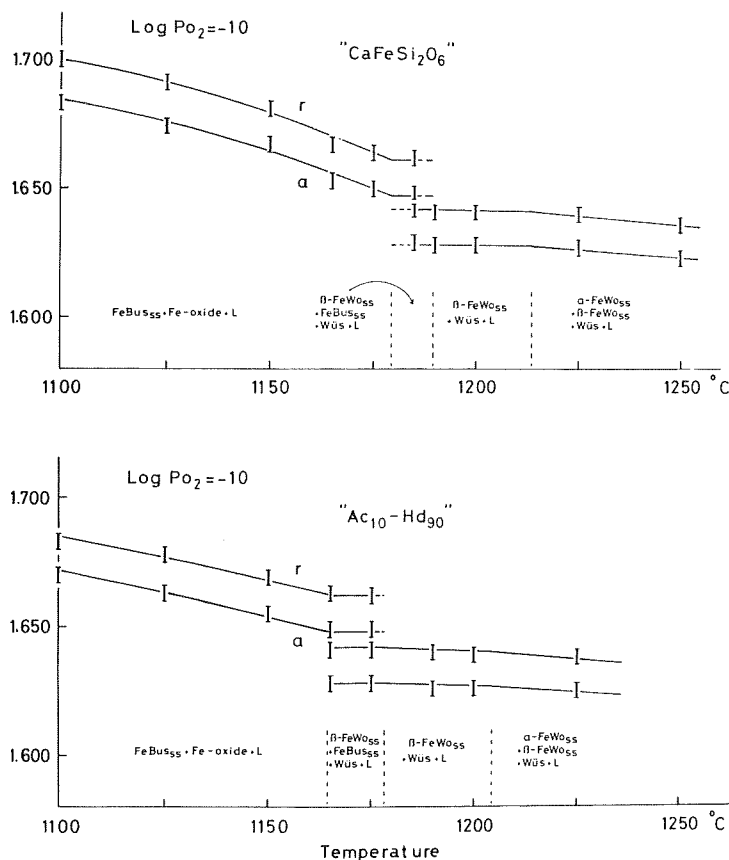
Fig. 4 Change of refractive indices of \beta\text{-Fe-wollastonite}_{\text{ss}} and \text{Fe-bustamite}_{\text{ss}} crystallized from the compositions of \text{CaFe}^{2+}\text{Si}_2\text{O}_6 and \text{Ac}_{10}\text{Hd}_{90} at 10^{-10} atm f_{\text{O}_2} . Abbreviations are same as in Fig. 1.
