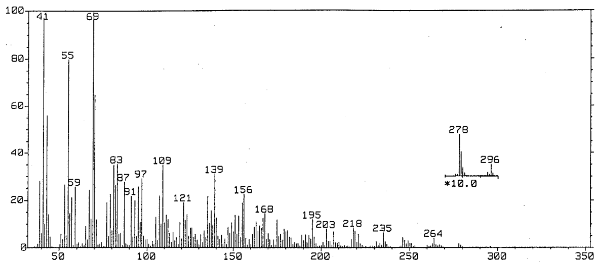
Fig. 3-84 EI-Mass Spectrum of RSA-CN
