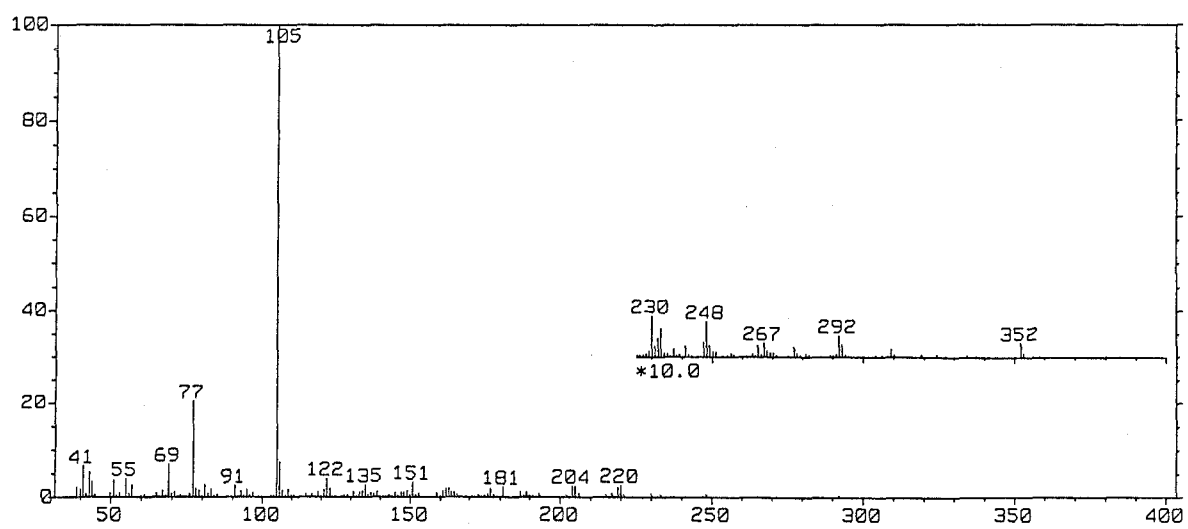
Fig. 3-91 EI-Mass Spectrum of RSA-BA
