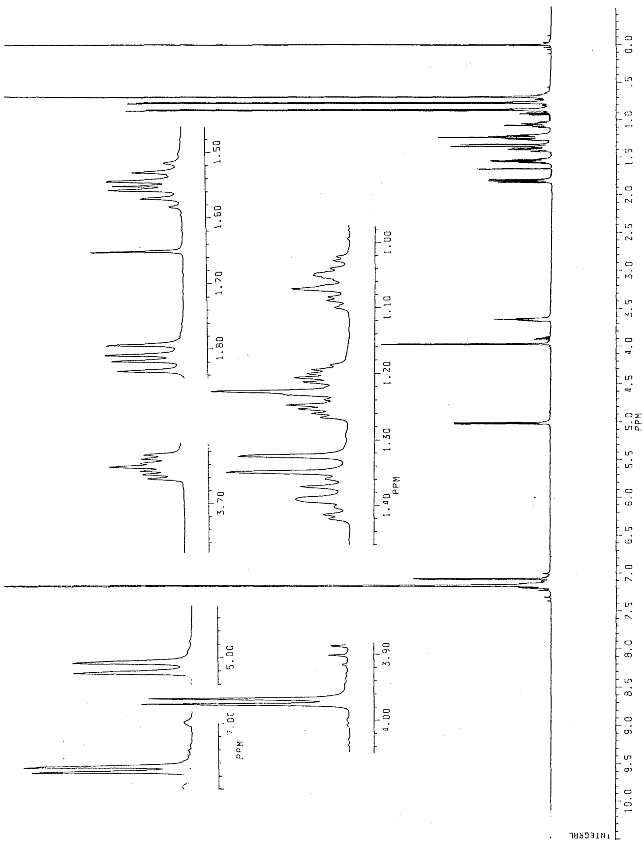
Fig. 3-133 ^1\text{H} -NMR Spectrum of RDA-FA-2 (500 MHz, in \text{C}_6\text{D}_6 )
