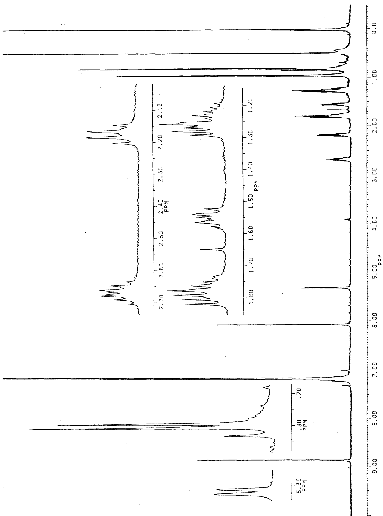
Fig. 3-81 ^1\text{H} -NMR Spectrum of RSA-PCC (500 MHz, in \text{C}_6\text{D}_6 )
