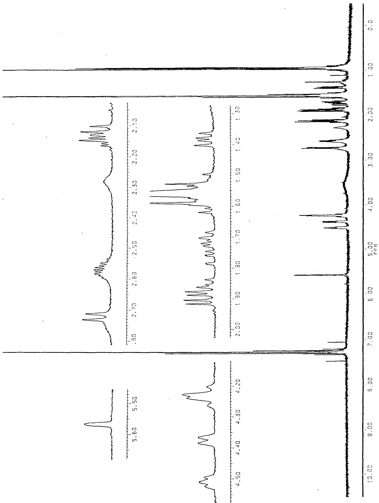
Fig. 3-57 ^1\text{H} -NMR Spectrum of RSA-NBH-TU (500 MHz, in \text{CDCl}_3 )
