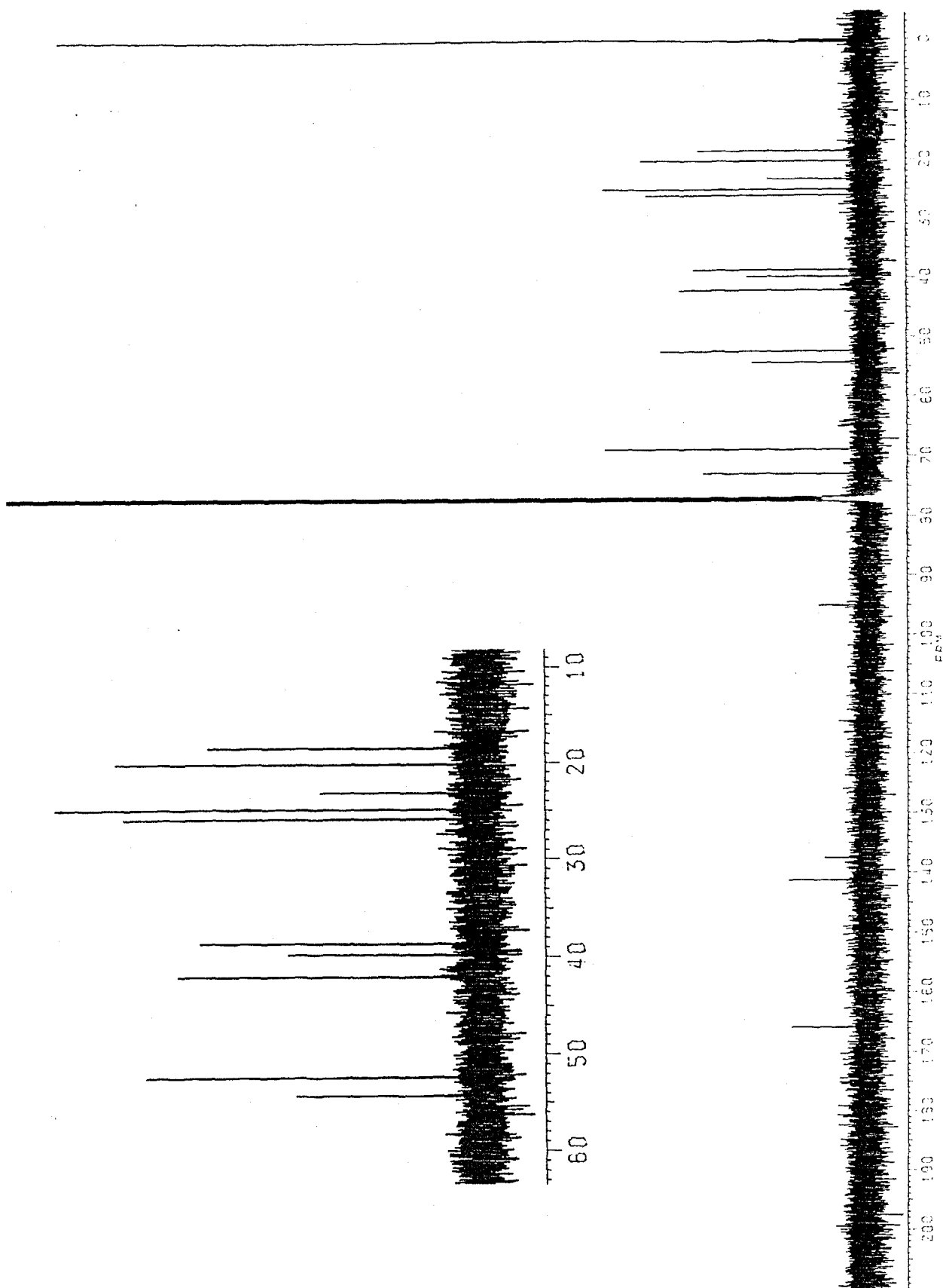
Fig. 3-87 ^{13}\text{H} -NMR Spectra of RSA-CN (125 MHz, in \text{CDCl}_3 , COM and DEPT)
