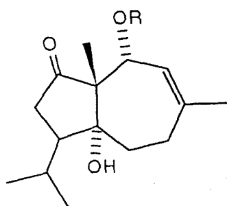
54 R=angelate [56]
