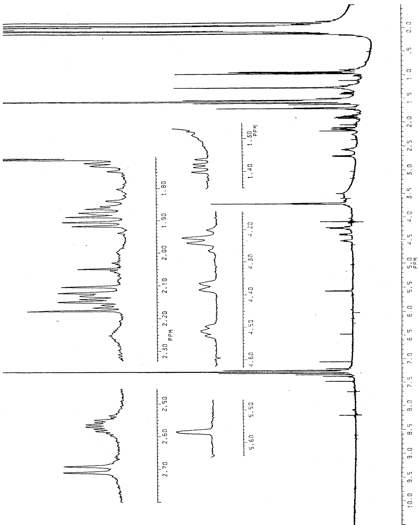
Fig. 3-53 ^1\text{H} -NMR Spectrum of RSA-LAH (500 MHz, in \text{CDCl}_3 )
