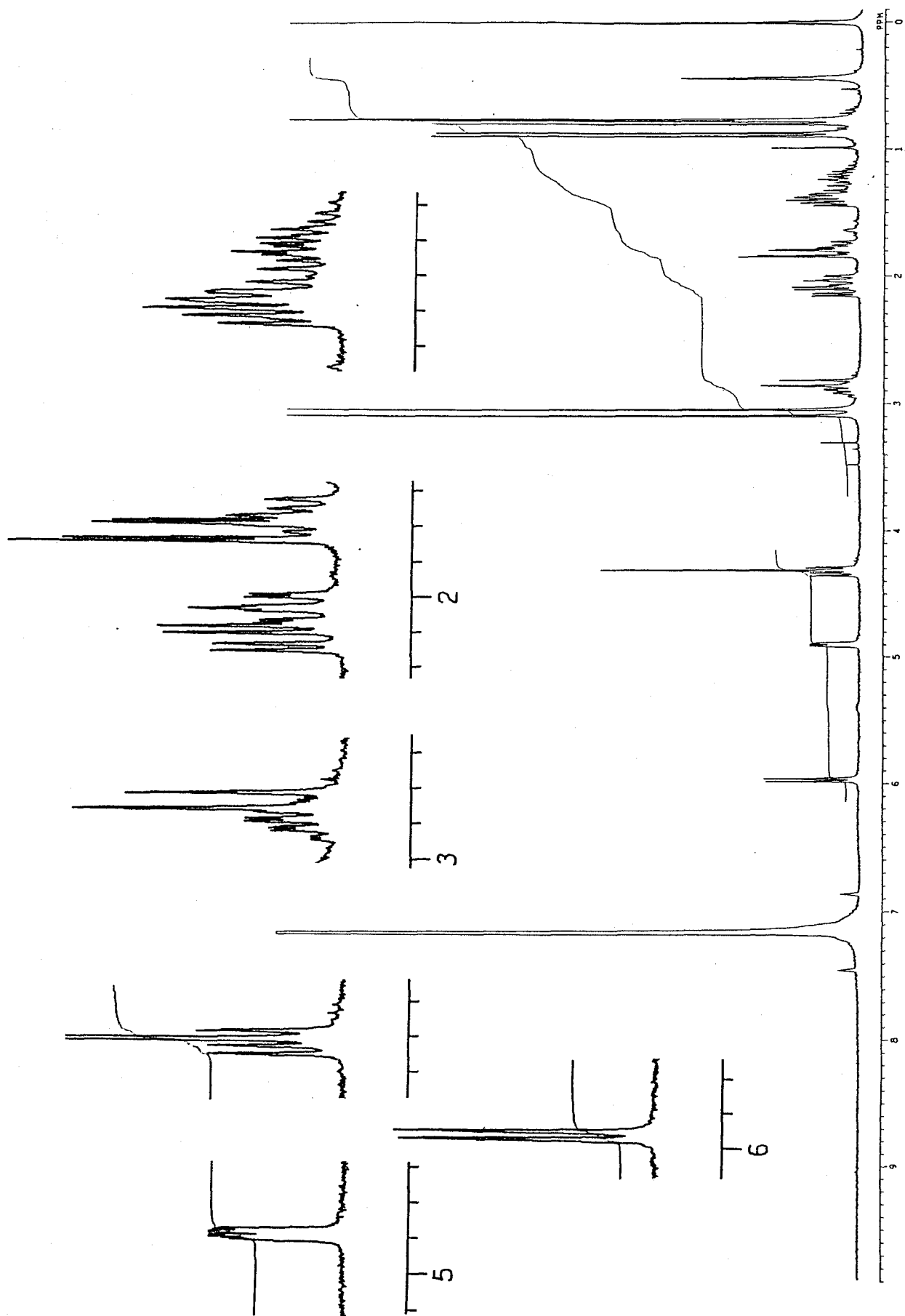
Fig. 3-67 ^1\text{H} -NMR Spectrum of RSA-HCL (270 MHz, in \text{C}_6\text{D}_6 )
