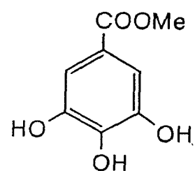
methyl gallate (76)
