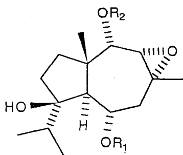
37; linkiol [43] R=angelate
