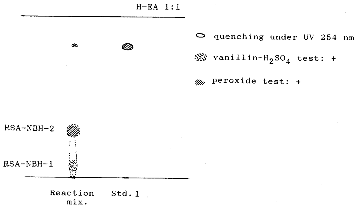
Fig. 3-37 TL Chromatogram of \text{NaBH}_4 Reduction Products of Rugosal A (1)
