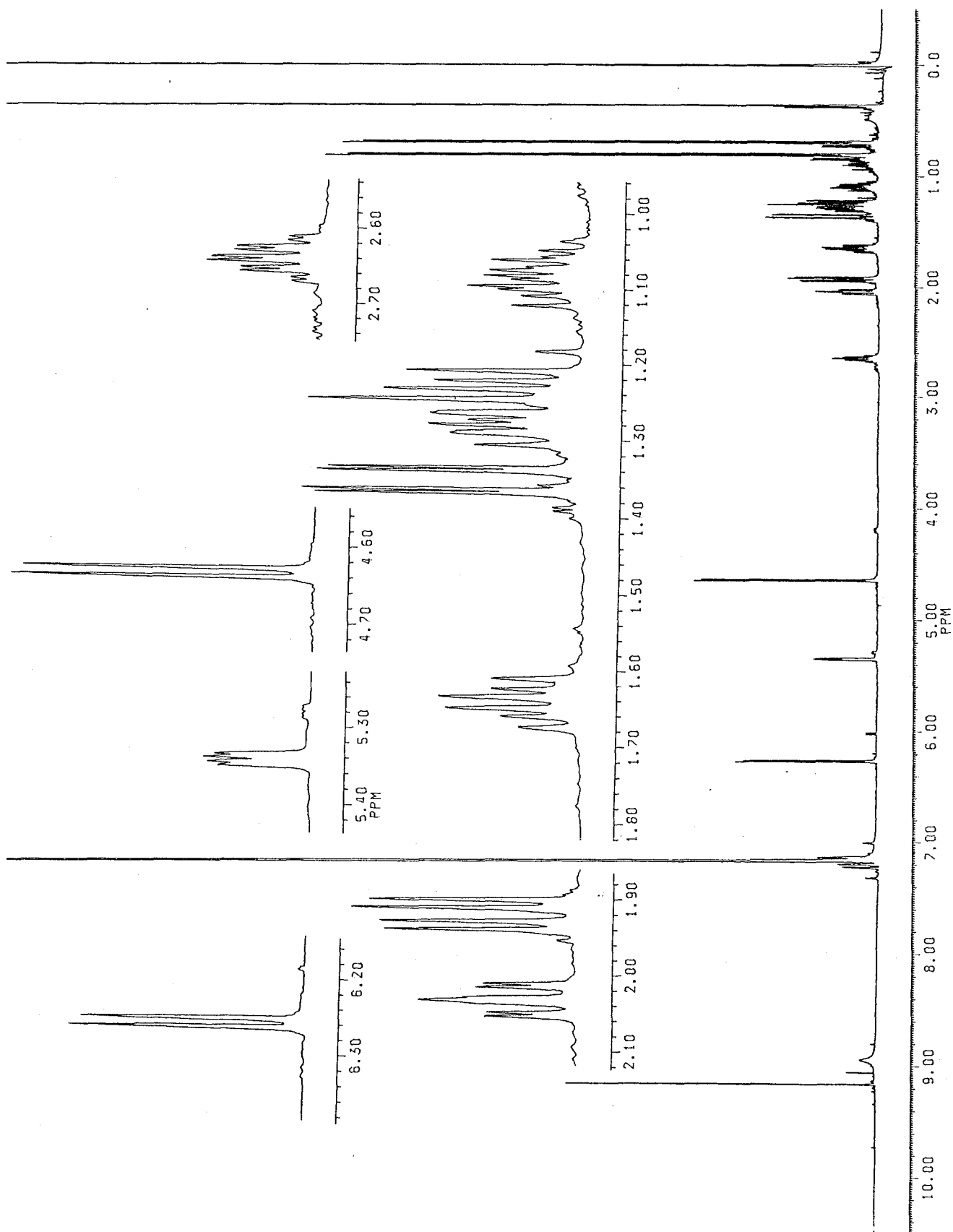
Fig. 3-202 ^1\text{H} -NMR Spectrum of RL-C-OX-A2 (500 MHz, in \text{C}_6\text{D}_6 )
