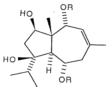
44; tingitanol [45] R=angelate
