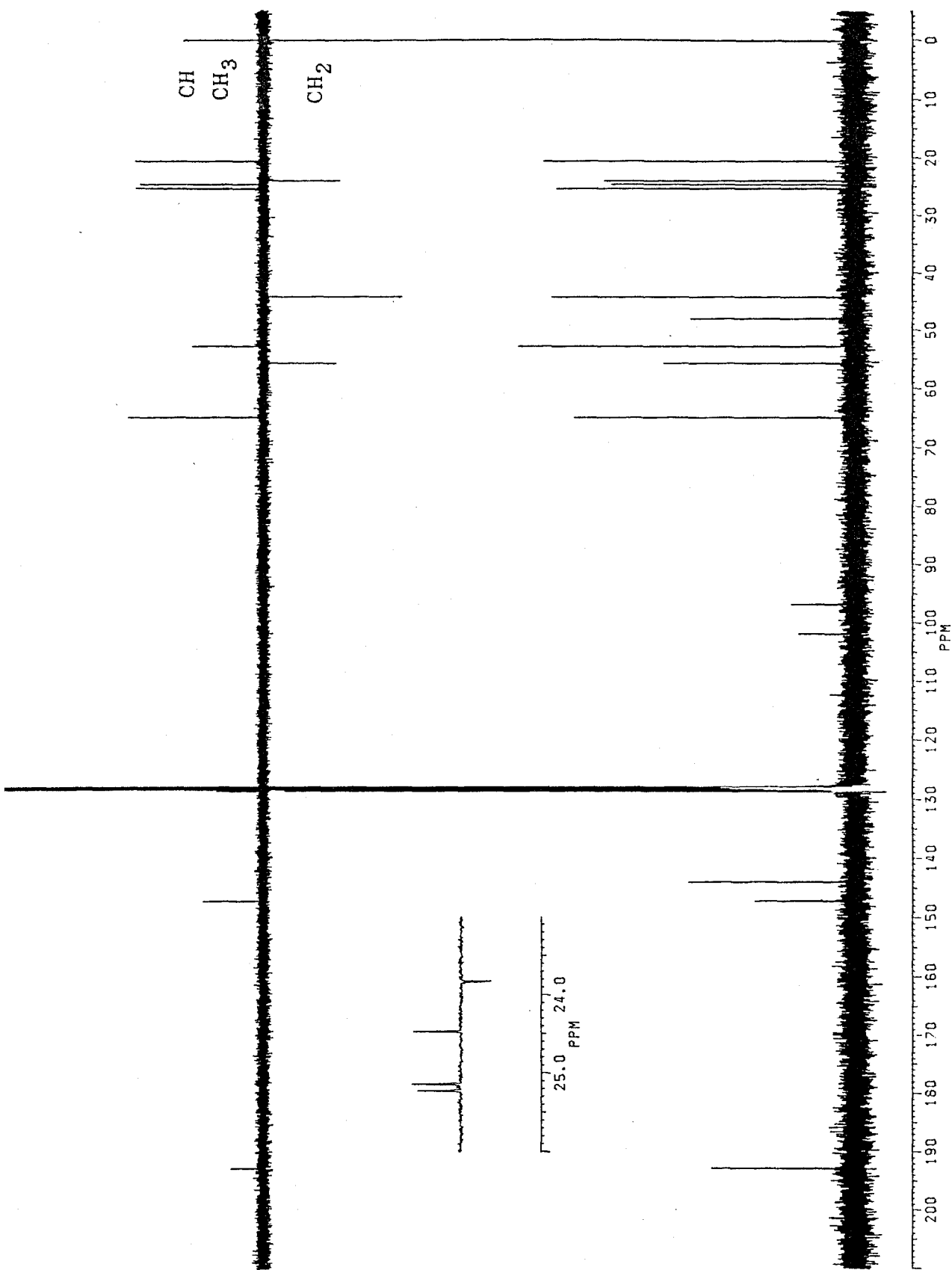
Fig. 3-62 ^{13}\text{C} -NMR Spectrum of RSA-PY (125 MHz, in \text{C}_6\text{D}_6 )
