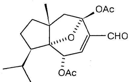
RSA-AC-2 (1b)
