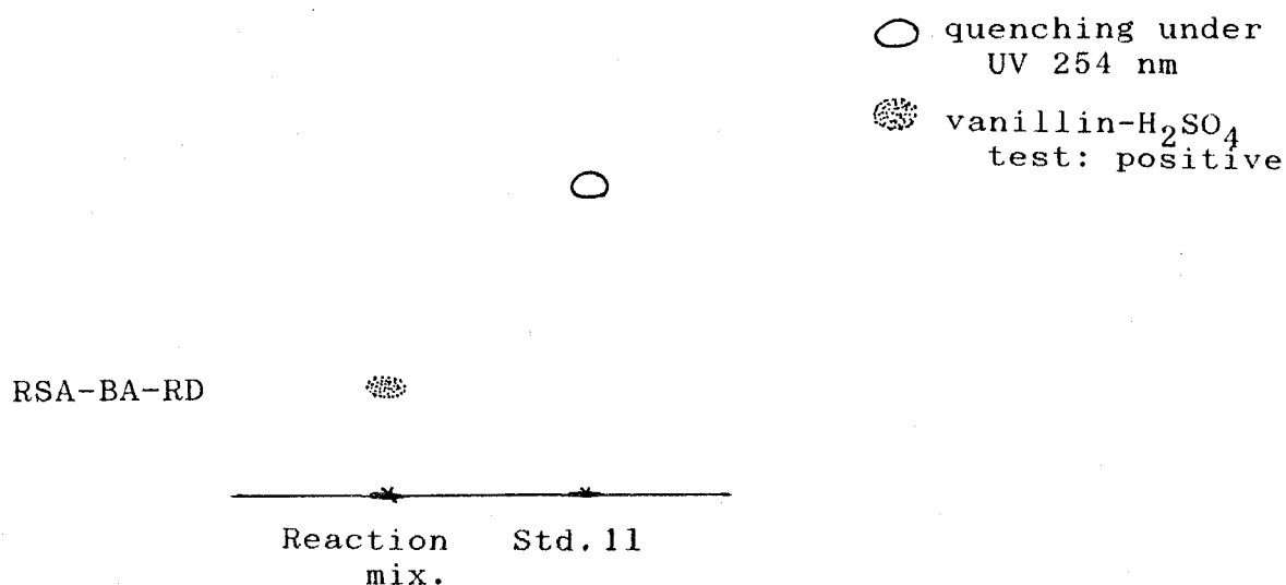
Fig. 3-97 TL Chromatogram of Reaction Product Obtained by \text{NaBH}_4 Reduction of Rugosal A (1)
