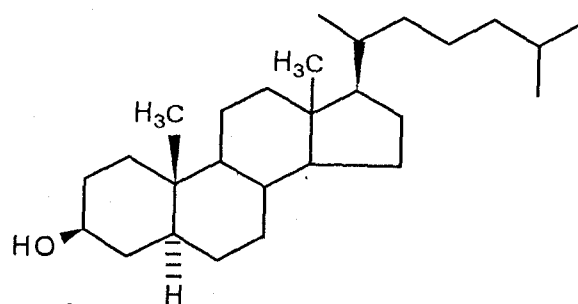
cholesterol (78) [76]
