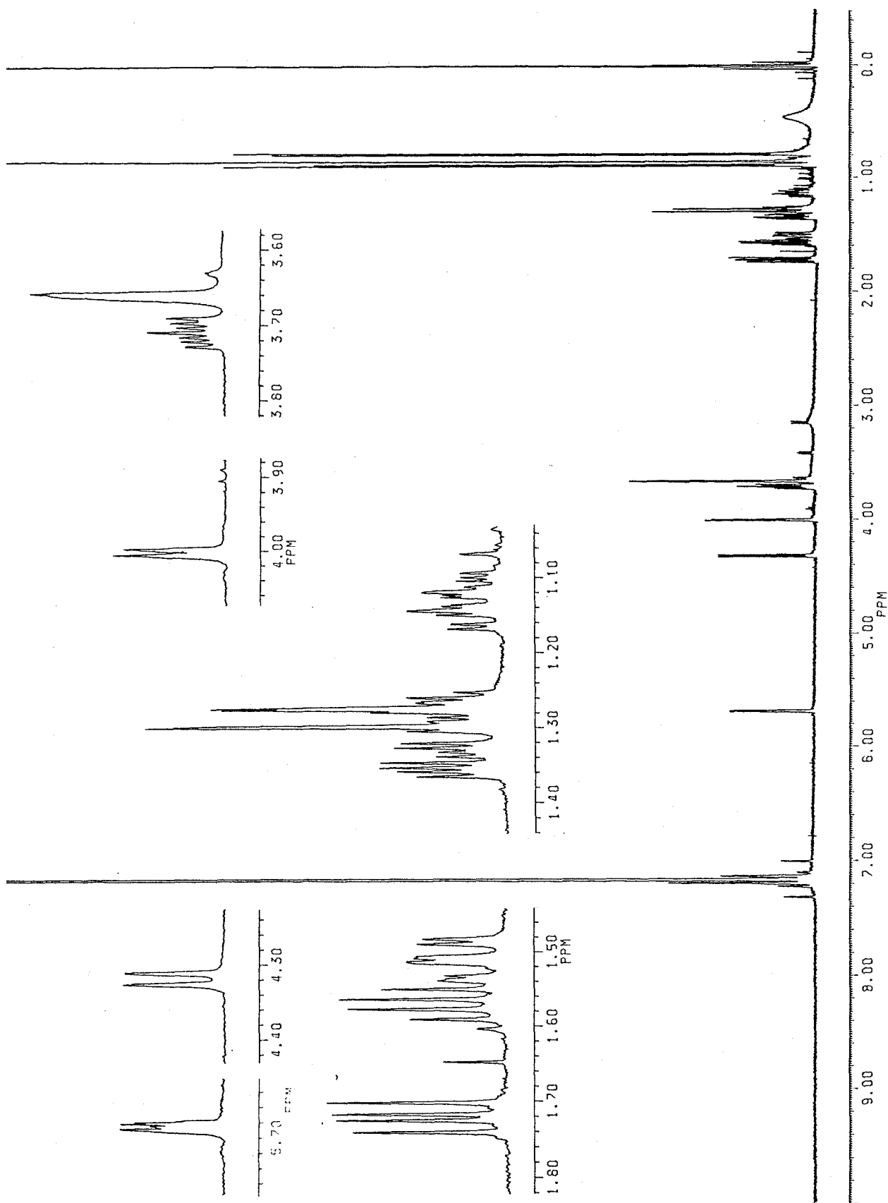
Fig. 3-146 ^1\text{H} -NMR Spectrum of RSA-NBH-TSA (500 MHz, in \text{C}_6\text{D}_6 )
