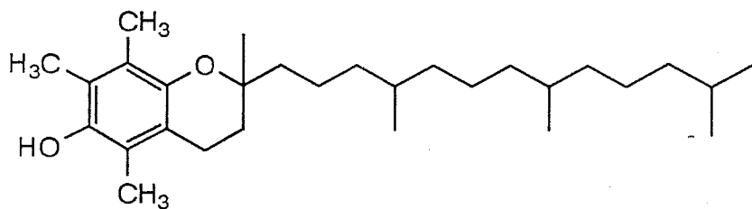
α-tocopherol (66) [79]
