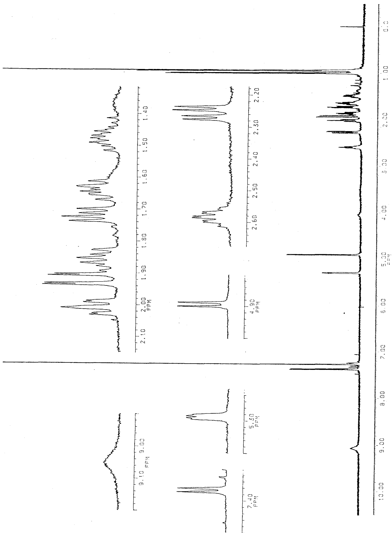
Fig. 3-229 ^1\text{H} -NMR Spectrum of RL-115M-A-OX (500 MHz, in \text{CDCl}_3 )
