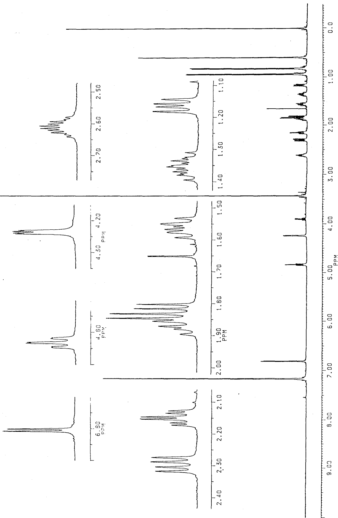
Fig. 3-128 ^1\text{H} -NMR Spectrum of RDA-TU-ME (500 MHz, in \text{C}_6\text{D}_6 )
