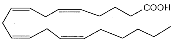
arachidonic acid (93)
