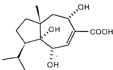
4; carota-1,4-dienoic acid (RL-115MA)
