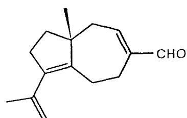
15; dehydrodaucenaldehyde (RL-D)
