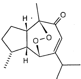
hydroperoxyhanalpinol (90)
