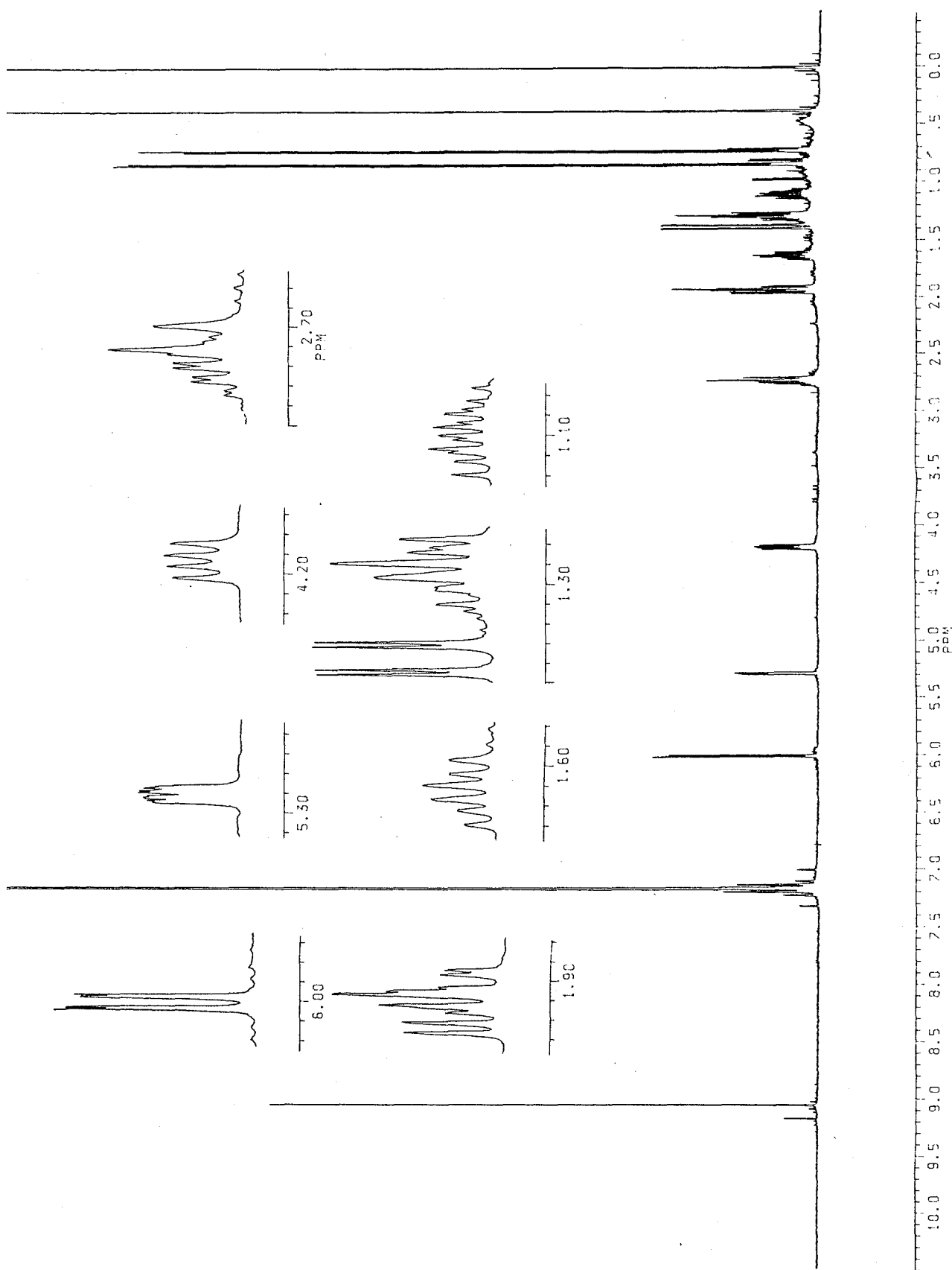
Fig. 3-196 ^1\text{H} -NMR Spectrum of RL-C-OX1 (500 MHz, in \text{C}_6\text{D}_6 )
