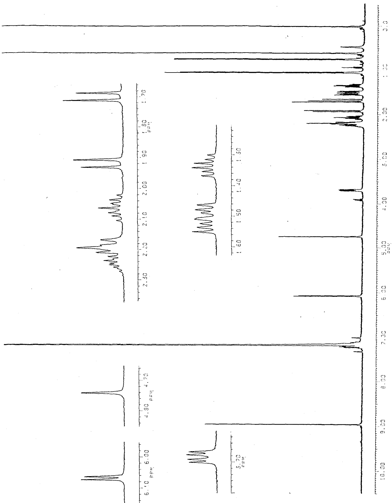
Fig. 3-61 ^1\text{H} -NMR Spectrum of RSA-PY (500 MHz, in \text{C}_6\text{D}_6 )
