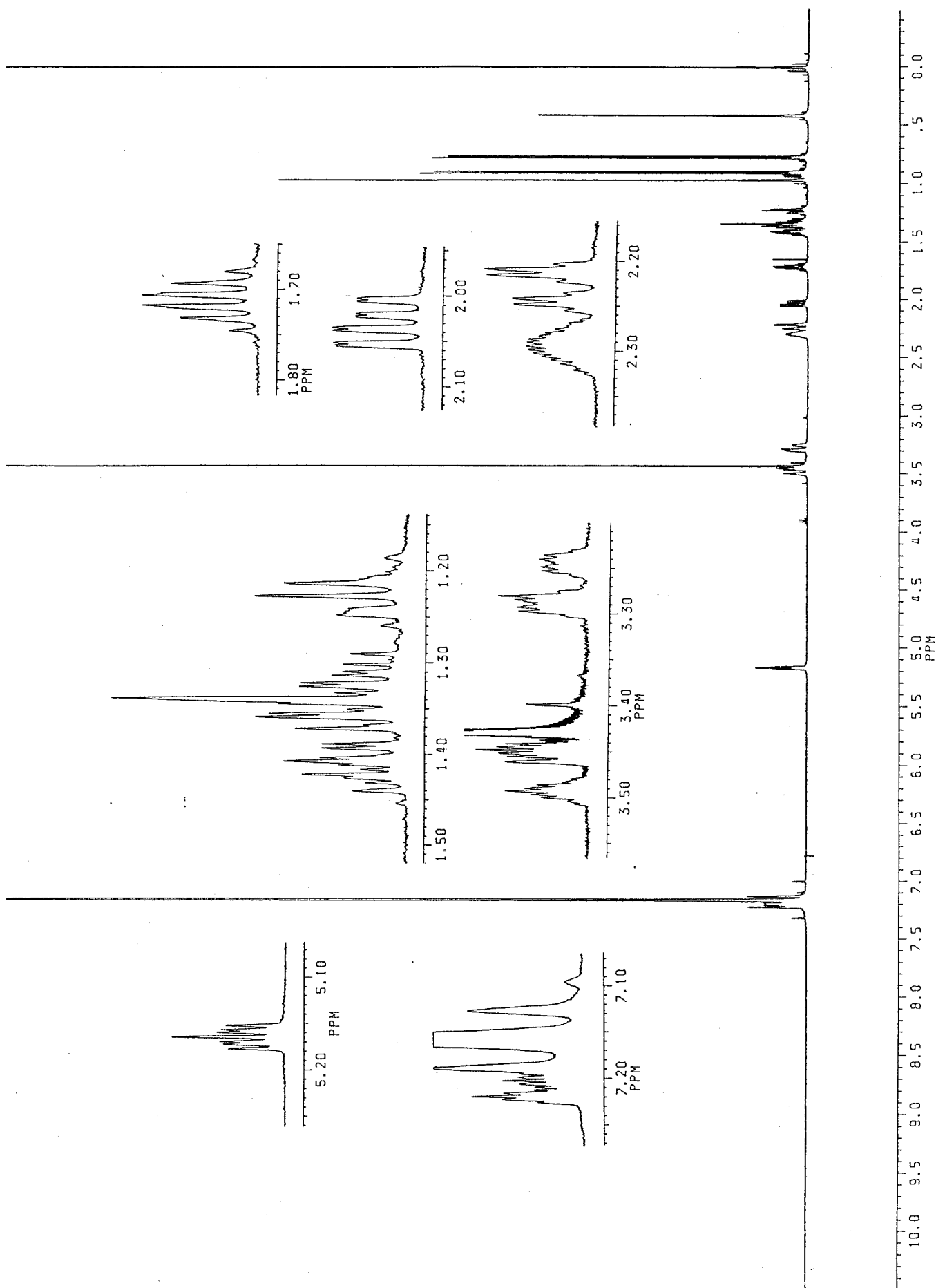
Fig. 3-178 ^1\text{H} -NMR Spectrum of RL-C-ME (500 MHz, in \text{C}_6\text{D}_6 )
