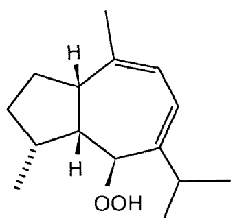
hydroperoxide intermediate (88)
