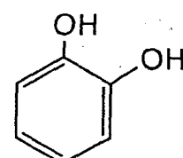
pyrocatechol (75)
