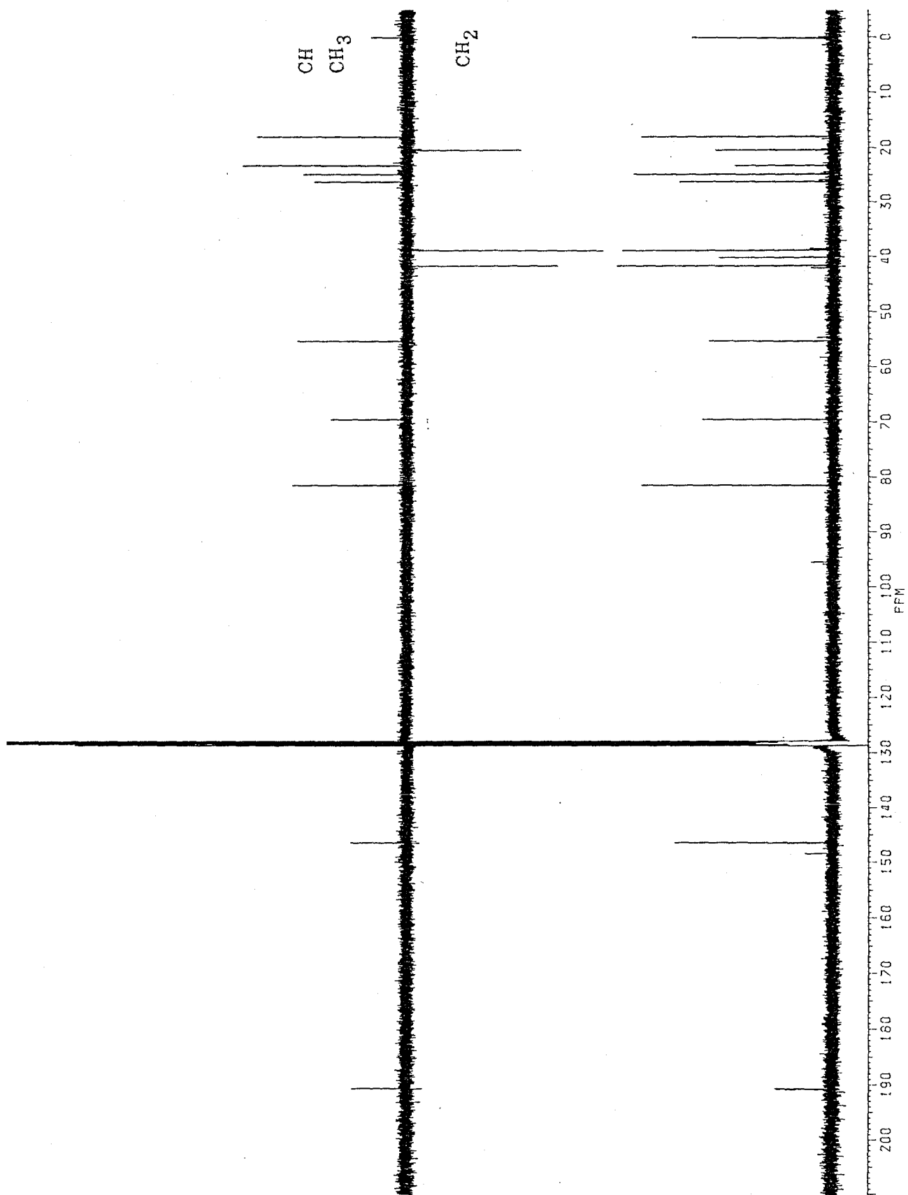
Fig. 3-204 ^{13}\text{C} -NMR Spectra of RL-C-OX-A2 (125 MHz, in \text{C}_6\text{D}_6 , COM and DEPT)
