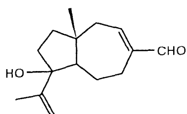
17; hydroxyisodaucenaldehyde (RL-119A)
