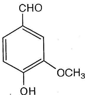
vanillin
