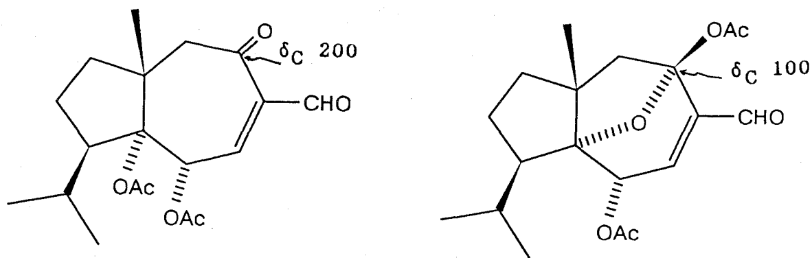
Fig. 3-35 Two Possible Structures for RSA-AC-2: In ^{13}\text{C} -NMR spectrum, H should show a ketone carbon signal around \delta_{\text{C}} 200, while I should have a ketal carbon around \delta_{\text{C}} 100.
