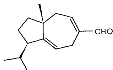
3; carota-1,4-dienaldehyde (RL-C)
