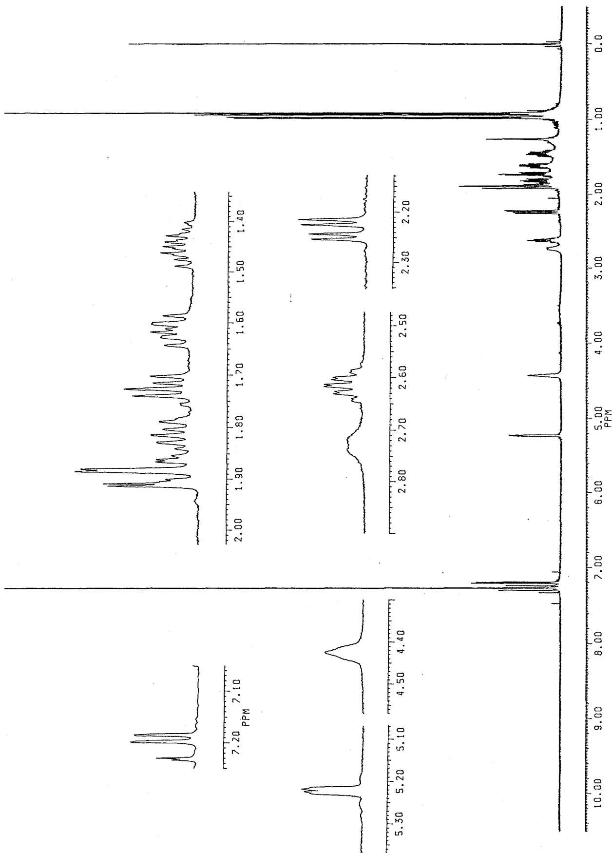
Fig. 3-197 ^1\text{H} -NMR Spectrum of RL-C-OX2 (500 MHz, in \text{C}_6\text{D}_6 )
