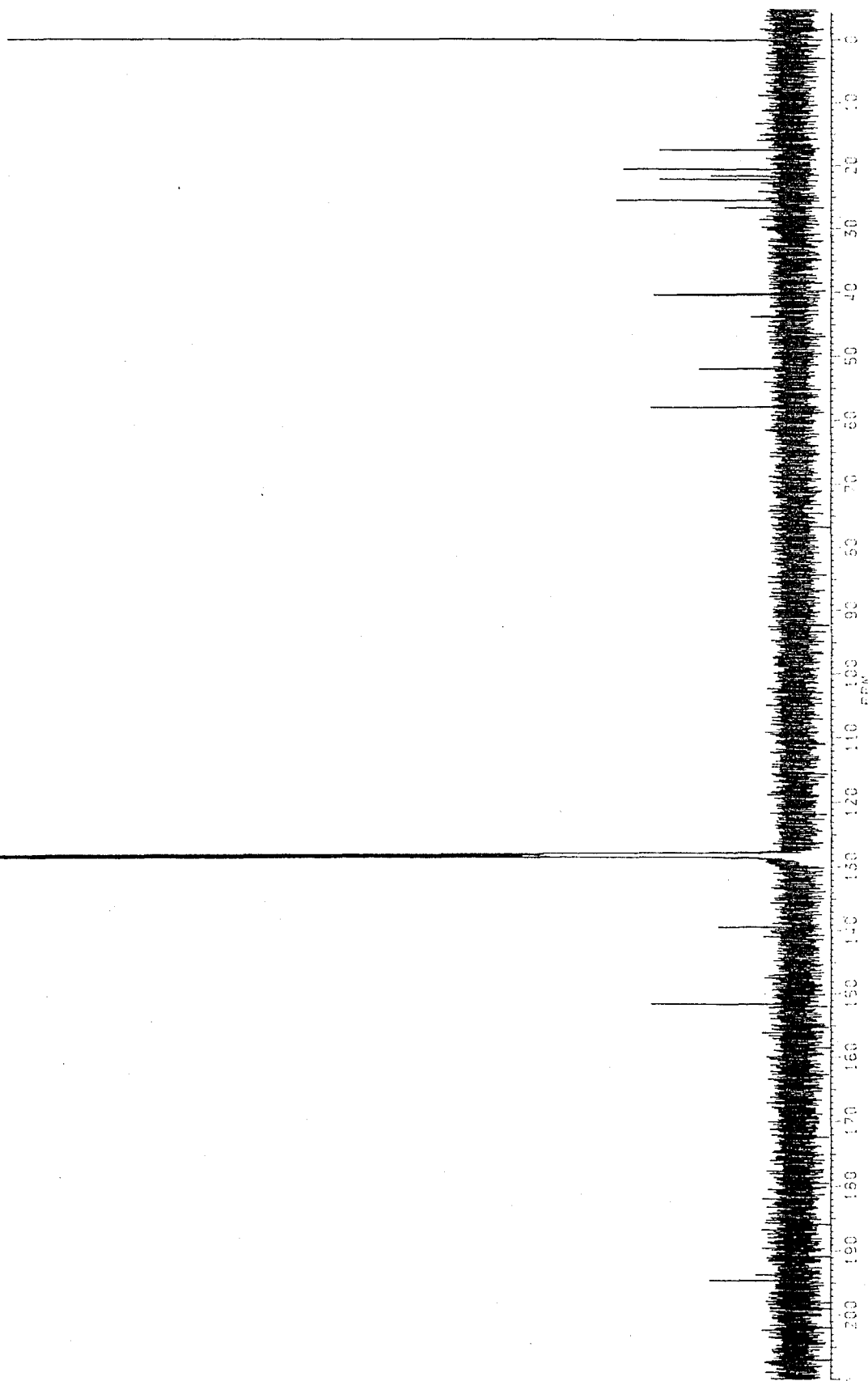
Fig. 3-213 13 C-NMR Spectrum of RL-C-OX-B1 (125 MHz, in C 6 D 6 ): The sample was further obtained from a oxgenated mixture of crude carota-1,4-dienaldehyde (3).
