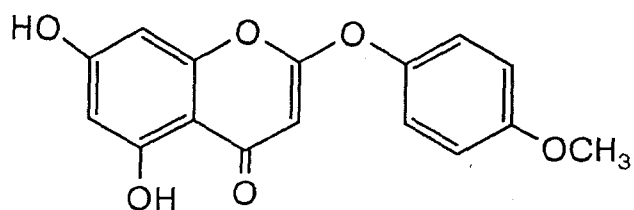
6-demethoxy-4'-methyloxyflavone (73)
