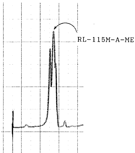
Fig. 3-189 HPLC Pattern of Methylated RL-115M Mixture Recorded on UV Detector at 230 nm (Unisil Q 100-5, 12 mm x 220 mm, 5 % EtOAc/ n -hexane)
