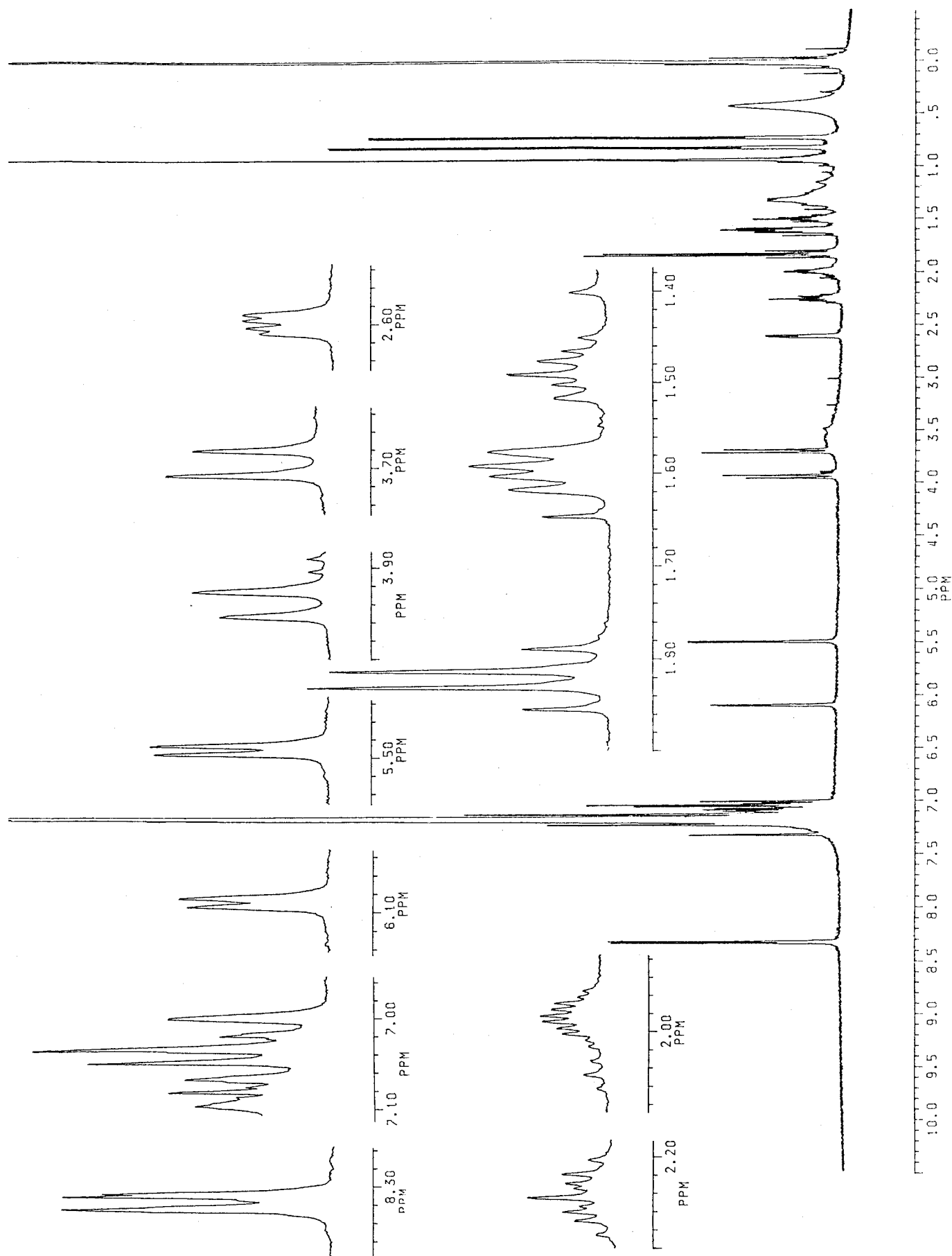
Fig. 3-100 ^1\text{H} -NMR Spectrum of RSA-BA-RD (500 MHz, in \text{C}_6\text{D}_6 )
