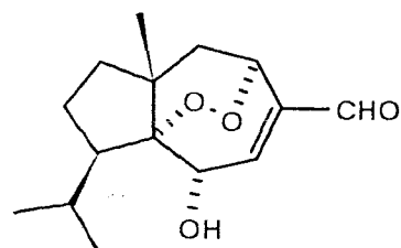
1; rugosal A
