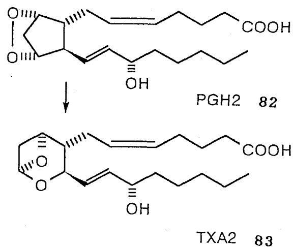
Scheme 3-9 Endoperoxide rearrangement of PGH 2 to yield TXA 2
