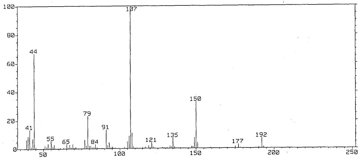
Fig. 3-222 EI-Mass Spectrum of RL-C-OX3
