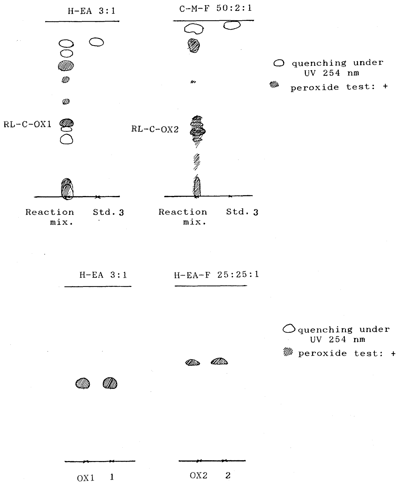
Fig. 3-193 TL Chromatograms of Autooxidation Products from Carota-1,4-dienaldehyde (3): Most of the products showed a positive response to peroxide test; however, those were quite unstable except two denoted as RL-C-OX1 and RL-C-OX2 in the chromatogram.
