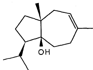
28; carotol [38,39]
