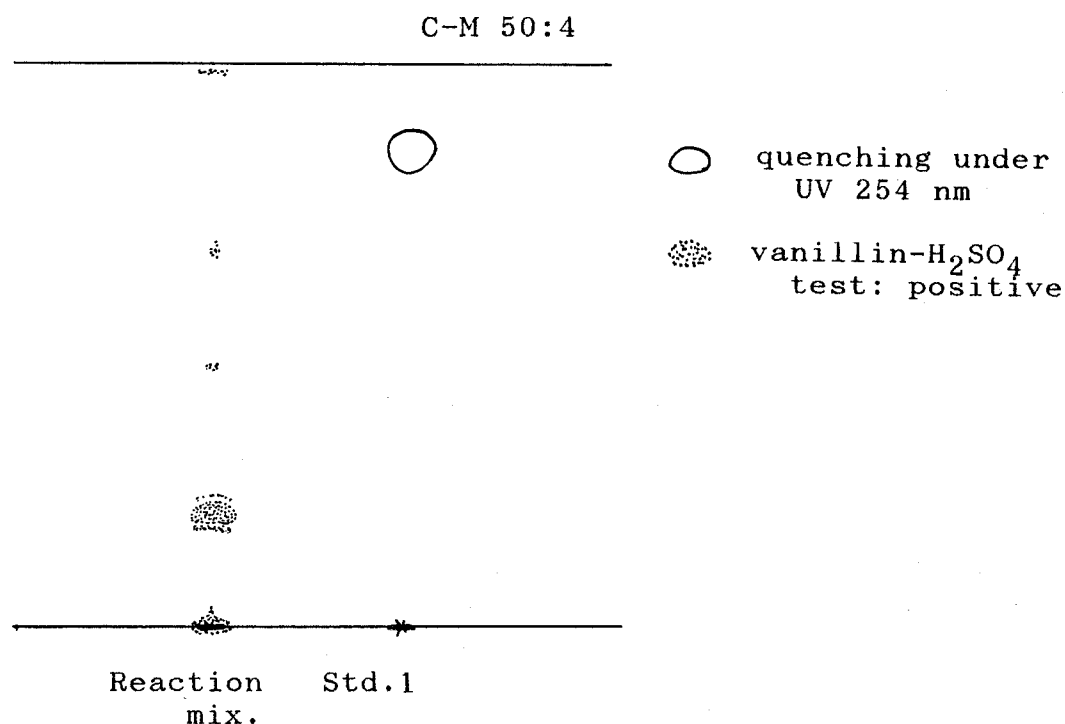
Fig. 3-50 TL-Chromatogram of Reaction Product Obtained by Reduction of Rugosal A (1) with \text{LiAlH}_4
