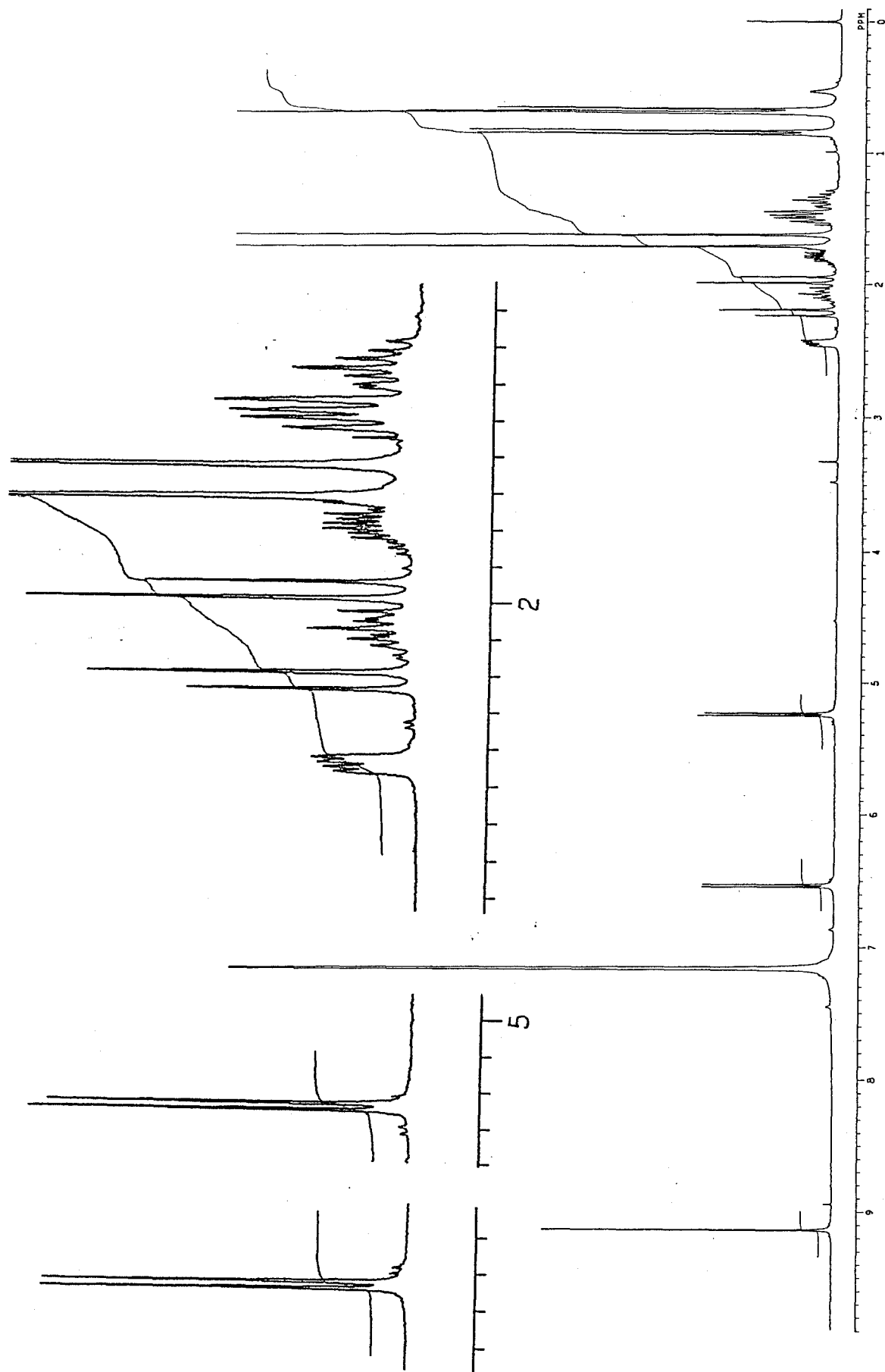
Fig. 3-34 ^1\text{H} -NMR Spectrum of RSA-AC-2 (270 MHz, in \text{C}_6\text{D}_6 )
