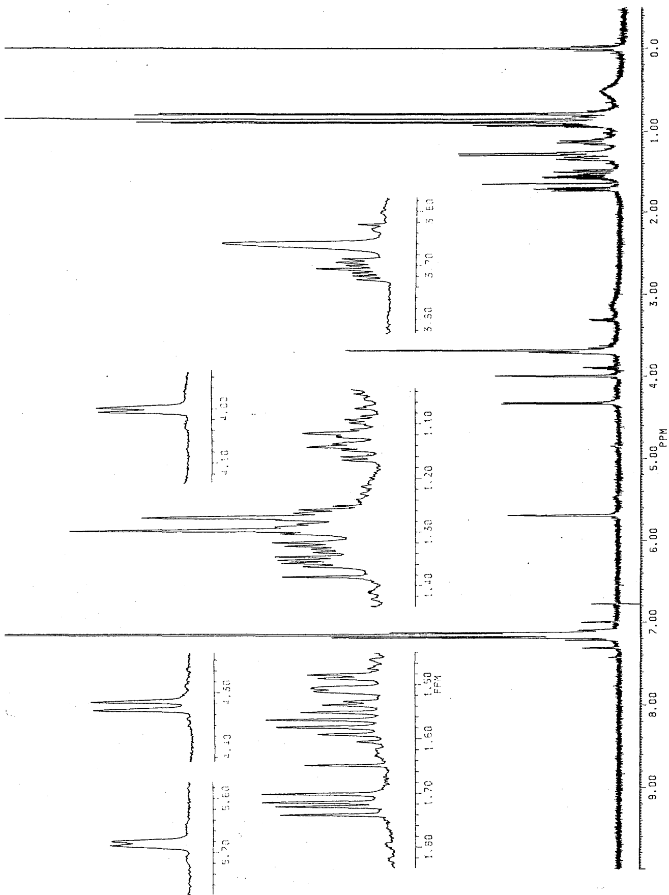
Fig. 3-143 ^1\text{H} -NMR Spectrum of RSA-NBH-TSA (500 MHz, in \text{C}_6\text{D}_6 )
