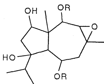
31; isolaserpitin [40] R=angelate
