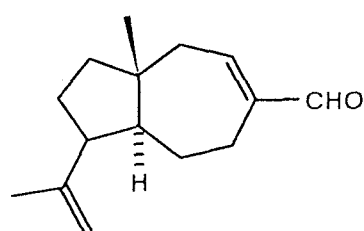
12; isodaucenaldehyde (RL-E)
