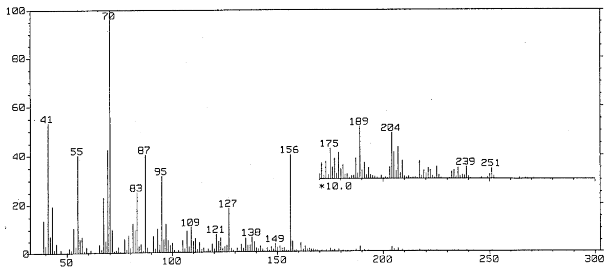
Fig. 3-142 EI-Mass Spectrum of RSA-NBH-TSA
