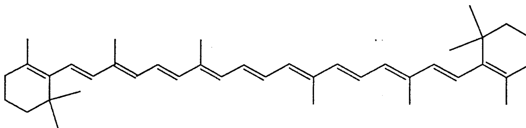
α-tocopherol (66) [79]
