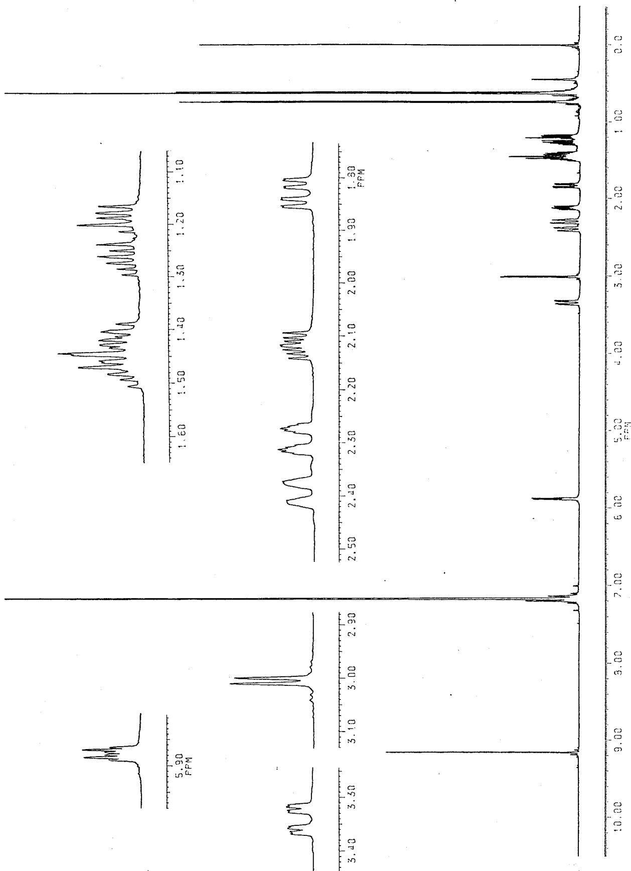
Fig. 3-181 ^1\text{H} -NMR Spectrum of RL-C-CPBA (500 MHz, in \text{C}_6\text{D}_6 )
