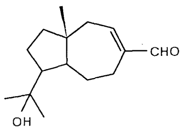
14; hydroxycarotanaldehyde (RL-117C)
