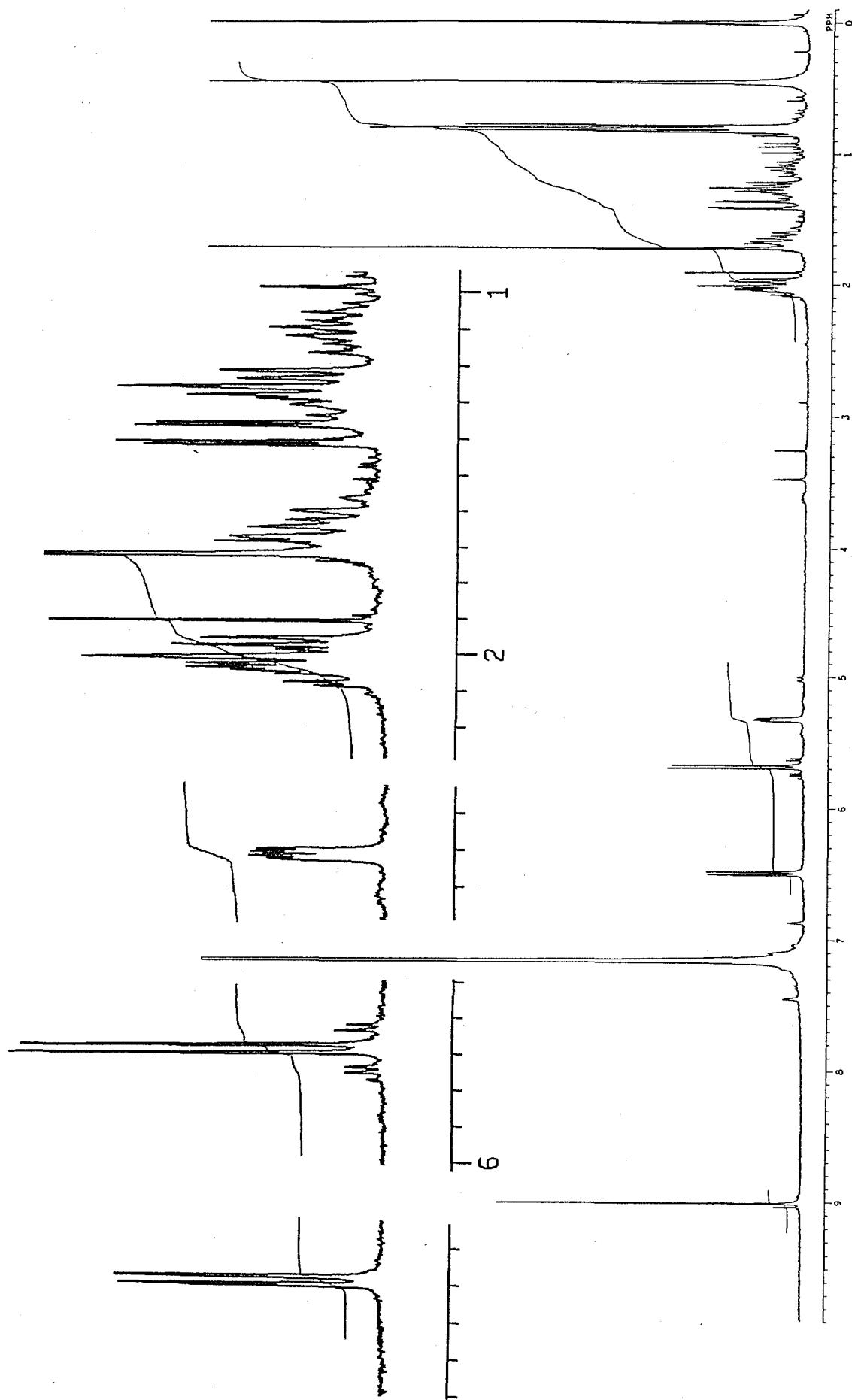
Fig. 3-31 ^1\text{H} -NMR Spectrum of RSA-AC-1 (270 MHz, in \text{C}_6\text{D}_6 )
