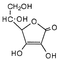
ascorbic acid (65) [79]
