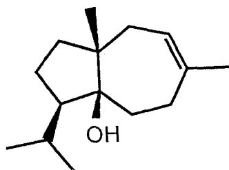
carotol (28)
