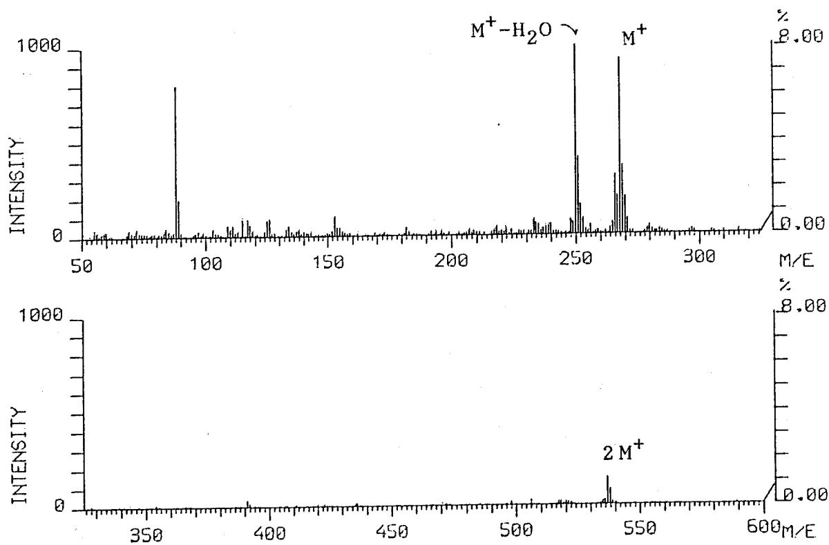
Fig. 3-38 FD-Mass Spectrum of RSA-NBH-1
