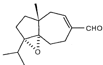
10; epoxydaucenaldehyde A (RL-109B)
