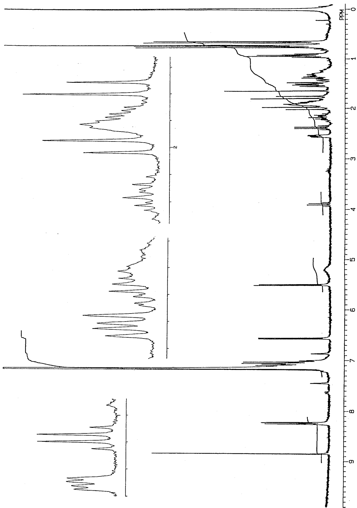
Fig. 3-92 ^1\text{H} -NMR Spectrum of RSA-BA (270 MHz, in \text{C}_6\text{D}_6 )
