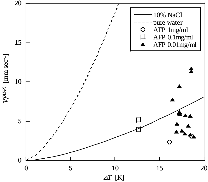
Figure 3 Lateral growth rate of CO 2 hydrate film v_f^{(AFP)} as a function of supercooling \Delta T and for various AFP concentrations. The dotted line and solid line indicate the previous data on pure water and 10 wt% NaCl solution, respectively. 14
