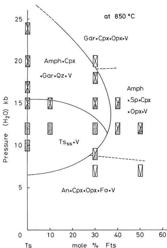
Fig. 3 Pressure-composition section at 850°C. Abbreviations are same as in Table 1.
