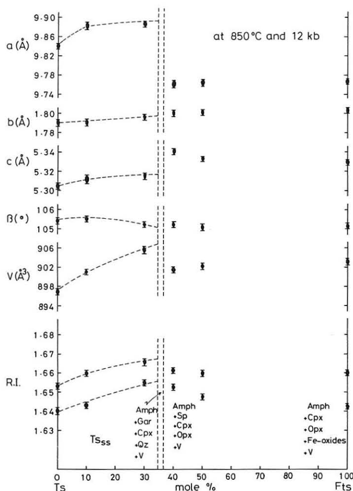
Fig. 4 Relationship between cell-dimensions or refractive indices of amphiboles with respect to chemical composition. Abbreviations are same as in Table 1.
