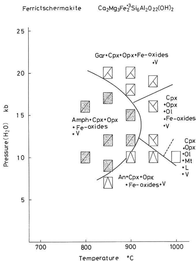
Fig. 2 Phase diagram of the composition of ferri-tschermakite at various temperatures and pressures. Abbreviations are same as in Table 1.
