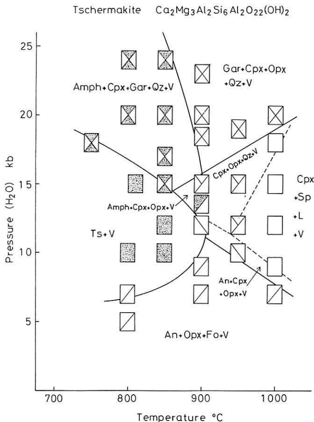
Fig. 1 Phase diagram of the composition of tschermakite at different temperatures and pressures. Abbreviations are same as in Table 1.
