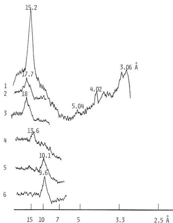
Fig. 14 X-ray diffraction patterns of a clay sample (< 0.2 μ ) from the Big I ash. 1: untreated, 2: solvated with glycerol, 3: water saturation, 4: K-saturation, 5: heated to 400°C, and 6: heated to 550°C.
