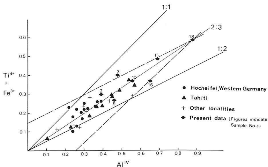
Fig. 8 Relation between \text{Ti}^{4+} + \text{Fe}^{3+} and \text{Al}^{\text{IV}} in Ti-rich clinopyroxenes from the various localities.
