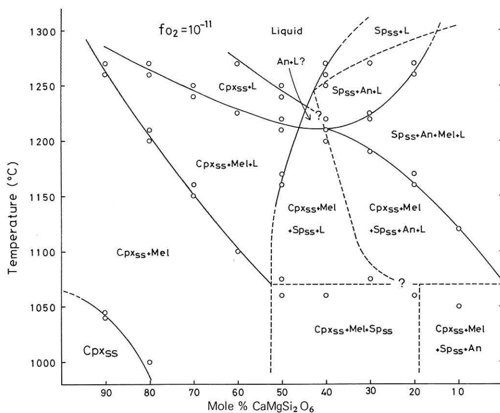
Fig. 3 Phase diagram of the join \text{CaMgSi}_2\text{O}_6 - \text{CaFe}^{3+}\text{AlSiO}_6 at 10^{-11} . Abbreviations are the same as in Table 1.
