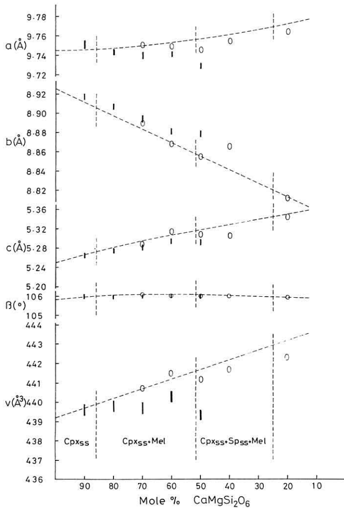
Fig. 5 Unit-cell dimensions of the clinopyroxene crystallized at 1100^\circ\text{C} and 10^{-10} atm f_{\text{O}_2} . The dashed lines: the variation of unit-cell dimensions of the clinopyroxene(ss) crystallized in air (Hijikata, 1968).
