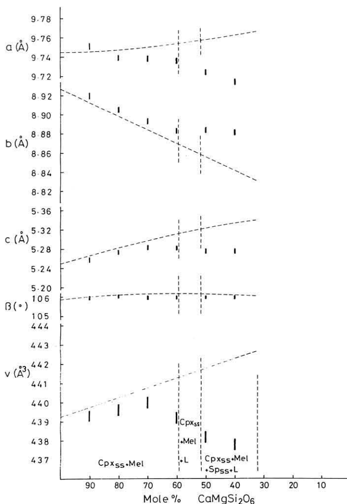
Fig. 6 Unit-cell dimensions of the clinopyroxene crystallized at 1100°C and 10^{-11} atm f_{O_2} . The dashed lines: the variation of the unit-cell dimensions of the clinopyroxene(ss) crystallized in air (Hijikata, 1968).
