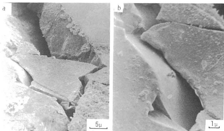
Fig. 6 Quasicleavage fracture in quartz grain (a), and its smooth and gentle swerved surface (b).
