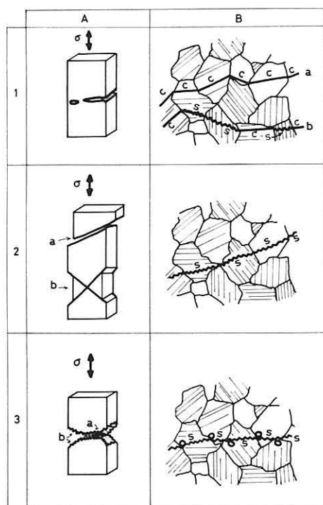
Fig. 1 Megascopic (A) and microscopic (B) fractures. 1. Cleavage fracture; a.continuous cleavage fracture, b.discontinuous cleavage fracture, 2. Shear fracture; a.slant-shear fracture, b.chisel-point fracture, 3. Normal (a) and shear (b) ruptures.
