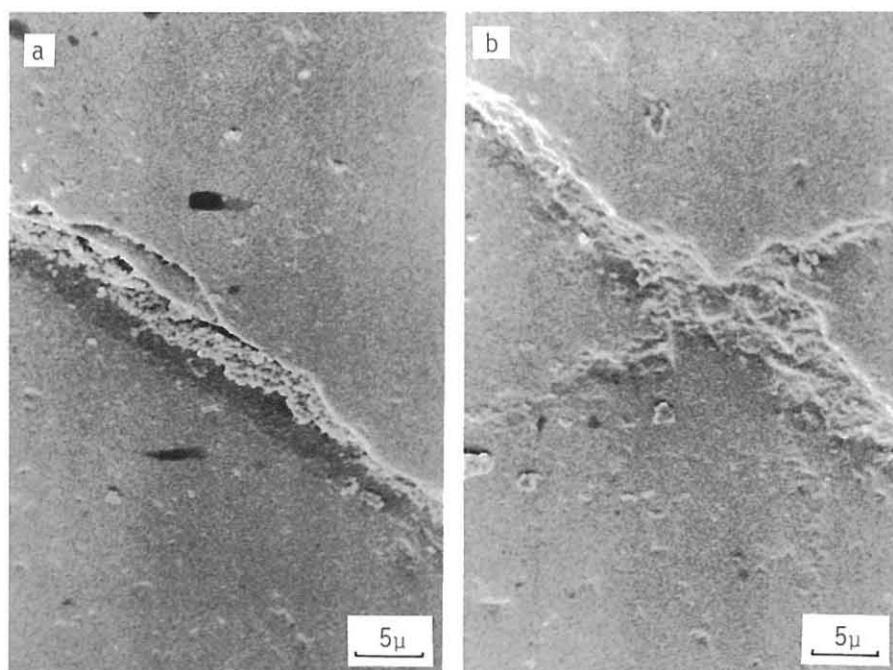
Fig. 8 The belt which consists of numerous minute fractures en échelon (a), and closed belts (b).
