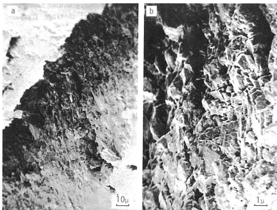
Fig. 3 Fracture surface in limestone (a), and the crystallographic from of calcite on the fracture surface (b).
