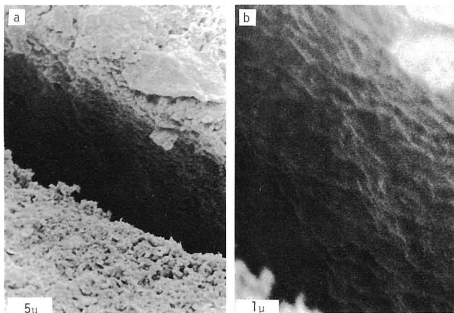
Fig. 9 A surface of normal rupture (a), and isometric dimples on the surface (b).
