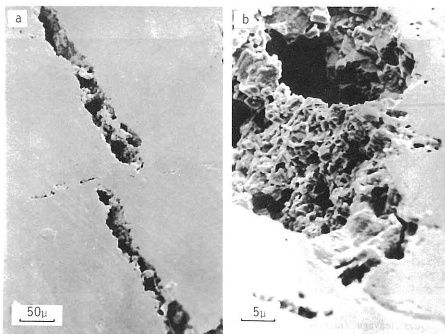
Fig. 4 Apices of fractures which do not reach the neighbour (a), and the stair-like form of apex (b).
