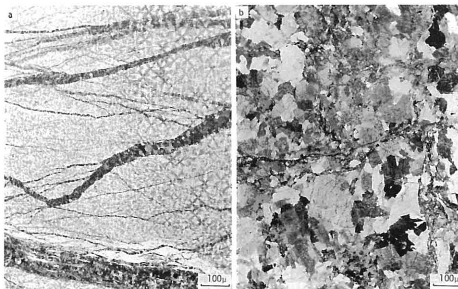
Fig. 11 Microphotograph of limestone pebble (a) and granite pebble (b).
