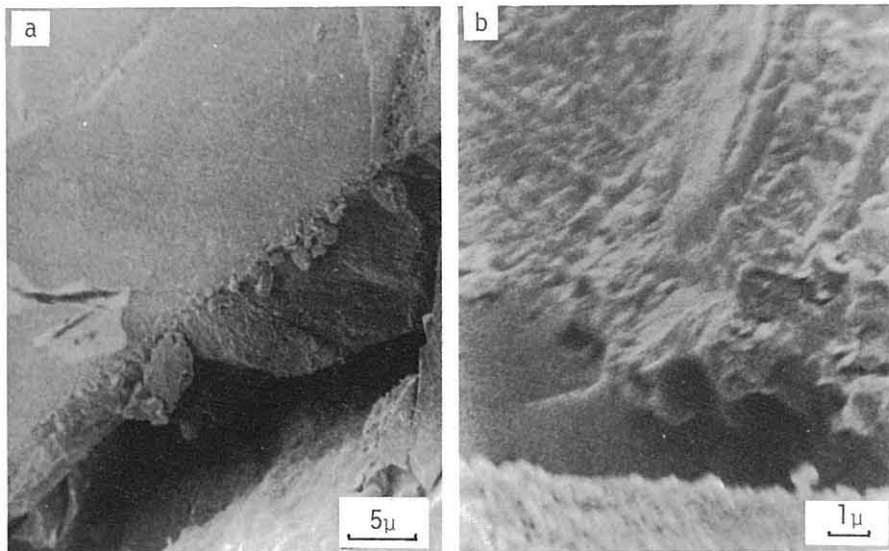
Fig. 10 A surface of shear rupture (a), and elongated dimples on the surface (b).
