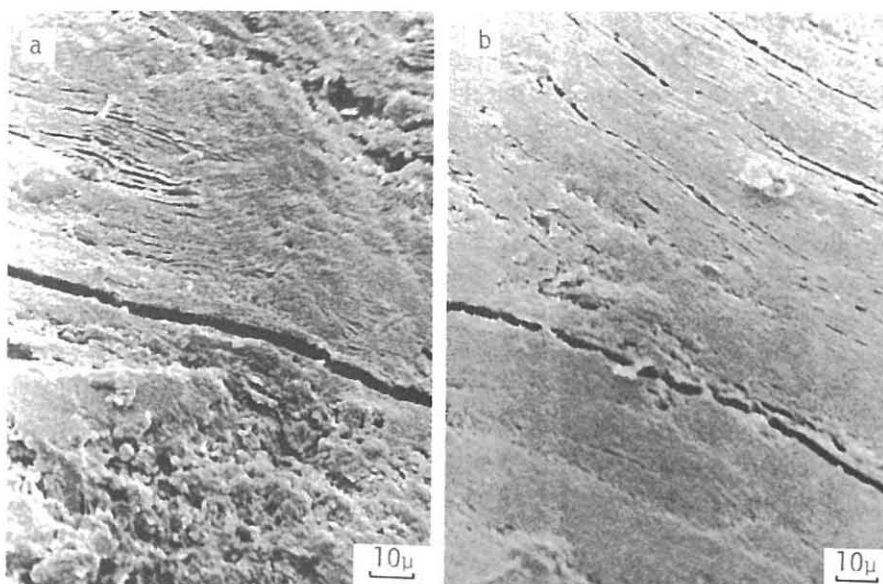
Fig. 5 Parallel cleavage fracture in feldspar grain (a), and in quartz grain (b).
