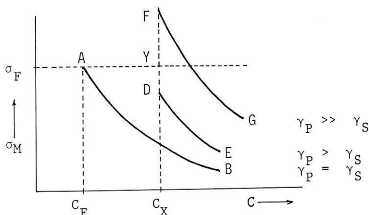
Fig. 12 An effect of plastic relaxation on plastic work, \gamma_p , according to the modification of Griffith's criterion.
