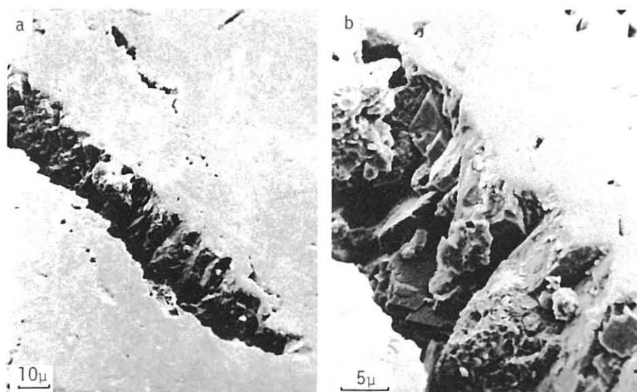
Fig. 2 Normal rupture in limestone pebble. A fracture with marked notches plane (a), and mutually crossed planes (b).
