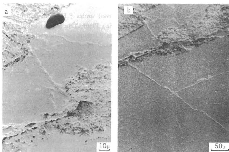
Fig. 7 shear fracture in quartz grain. The fracture with displacement along its plane (a) and a set of crossed fractures.
