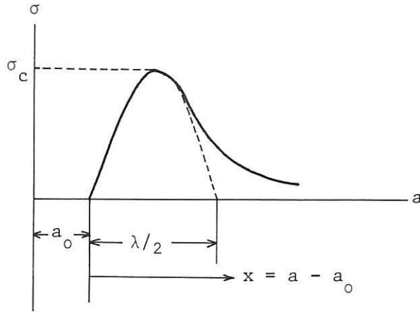
Fig. 13 The tensile stress needed to pull apart in a > a_0 distance. a_0 : the equilibrate distance between atoms at \sigma = 0 . Fracturing occurs at \sigma = \sigma_c .
