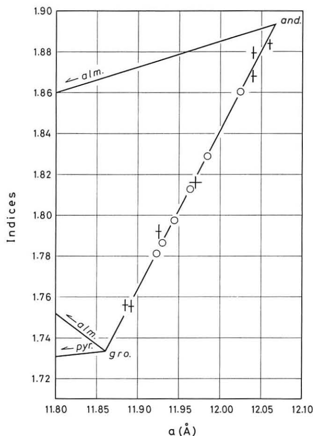
Fig. 1. Relationship between refractive indices and cell-parameters of natural (cross) and synthetic (open circle) optical anomaly garnets. and; andradite, gro; grossular, pyr; pyrope, alm; almandine
