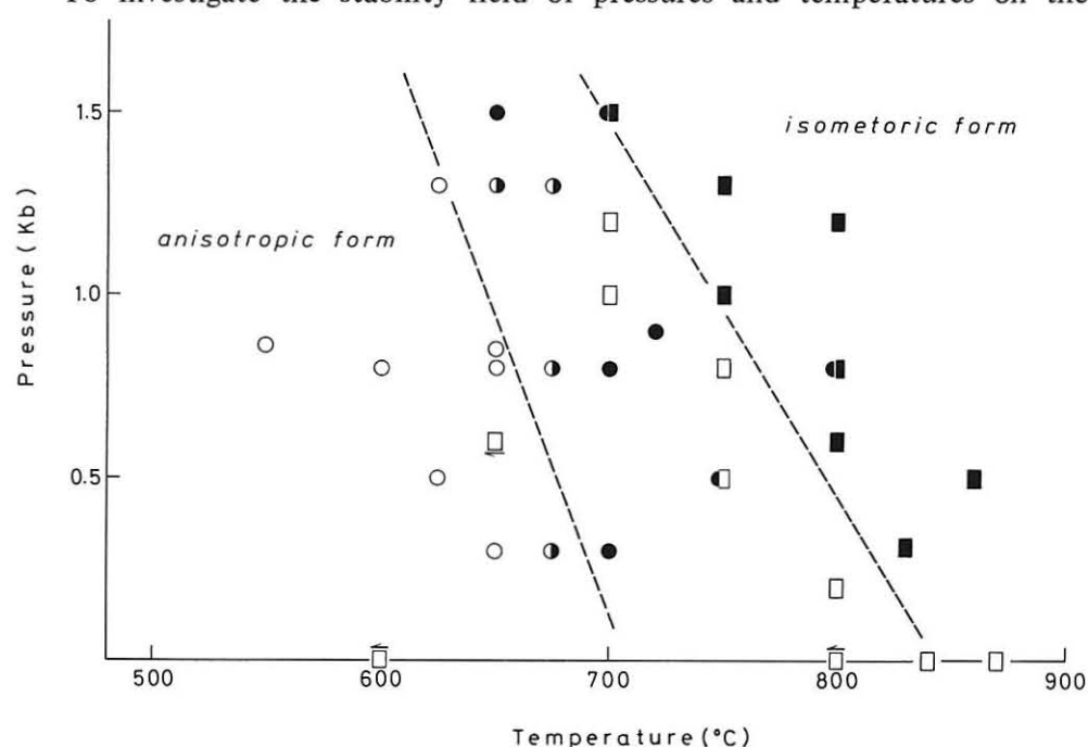
Fig. 2. Stability field of natural and synthetic optical anomaly garnets.
