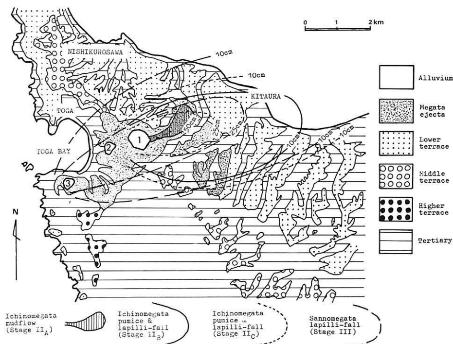
Fig. 9 Map showing the distribution of volcanic ejecta from three maars in Oga Peninsula, 1: Ichinomegata, 2: Ninomegata, and 3: Sannomegata. Tephra falls represented by thickness contour lines.
