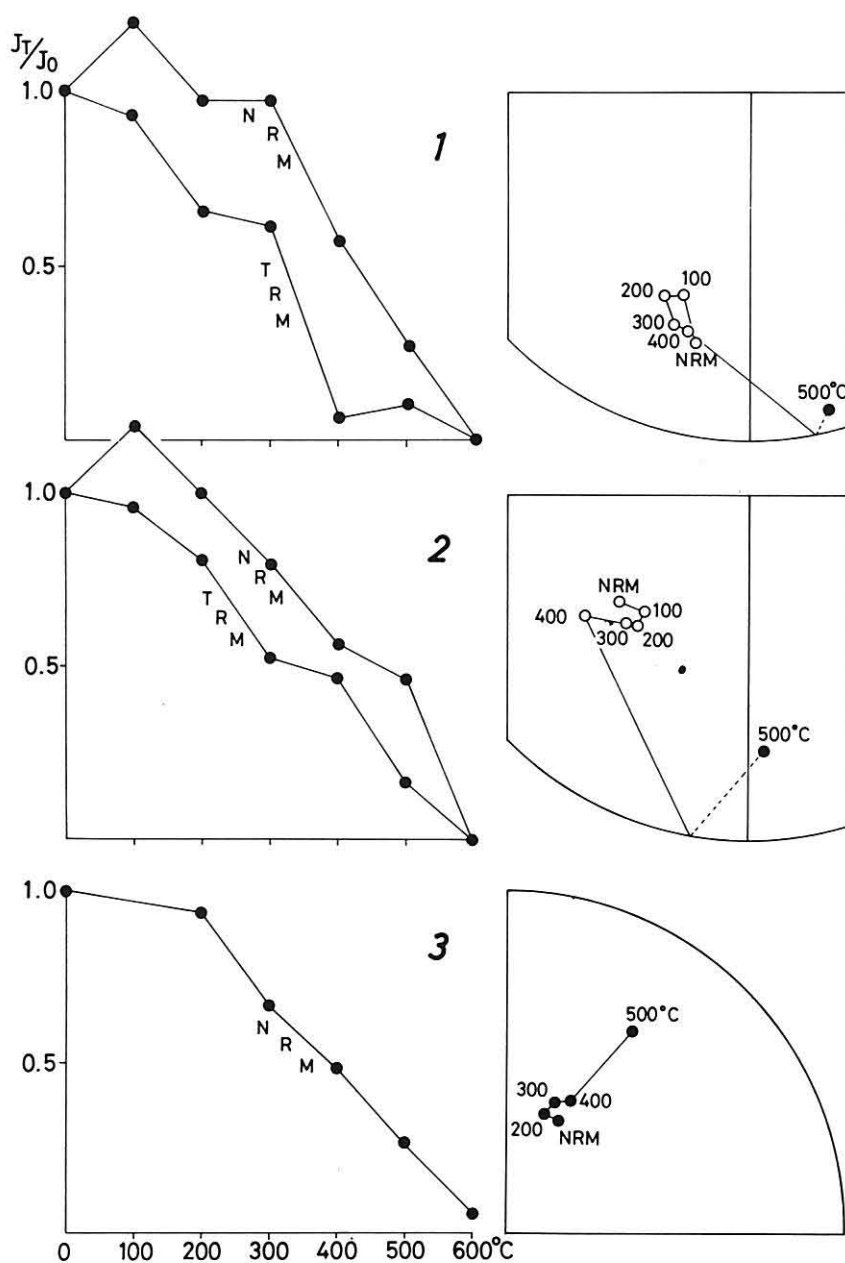
Fig. 4 Intensity decay curves for natural remanent magnetization (NRM) and also thermo remanent magnetization (TRM) and changes in the directions of NRM during demagnetization with temperature.
