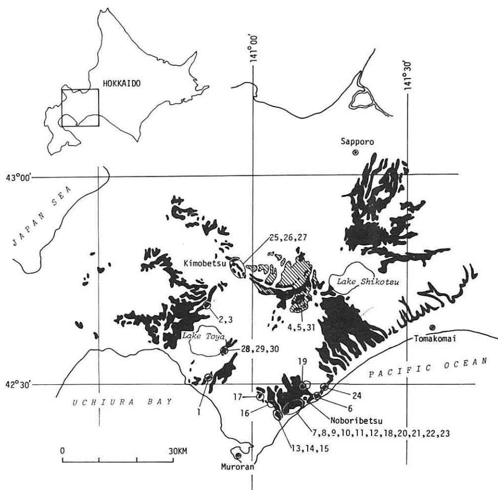
Fig. 1 Distribution of the Quaternary pyroclastic deposits and the volcanic product developed in the Shikotsu – Toya districts. Black: Pyroclastic deposits. Hatched: the Sokeishu lava. Numerals correspond with the numbers of the sampling sites shown in the Table 1.
