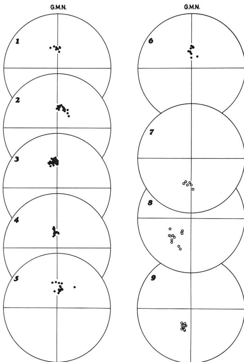
Fig. 2 Directions of natural remanent magnetization for the pyroclastic deposits distinguished. Solid circles represent lower hemisphere projections and open circles represent upper hemisphere on Schmidt's net. G.M.N.: Geomagnetic north 1: Toya pumice flow. 2: Shikotsu welded tuff. 3: Ponayoro pumice flow. 4: Noboribetsu welded tuff. 5: Ranpoge pumice flow. 6: Kimobetsu welded tuff. 7: Takinoue welded tuff. 8: Sobetsu pumice flow 9: Sokeishu lava flow.
