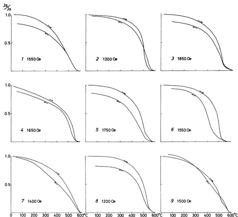
Fig. 3 Typical thermomagnetic curves for each pyroclastic deposit (1–8) and the Sokeishu lava (9). 1: Toya pumice flow. 2: Shikotsu welded tuff. 3: Ponayoro pumice flow. 4: Noboribetsu welded tuff. 5: Ranpoge pumice flow. 6: Kimobetsu welded tuff. 7: Takinoue welded tuff. 8: Sobetsu pumice flow.
