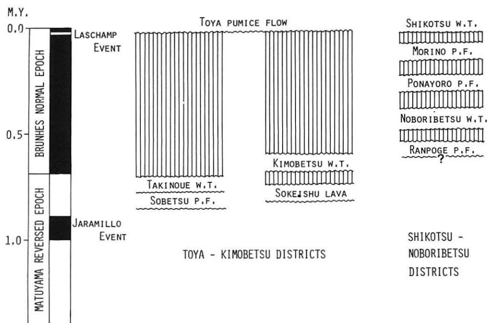
Fig. 5 Correlation diagram of pyroclastic deposits in southwestern Hokkaido as deduced from the present paleomagnetic measurements.
