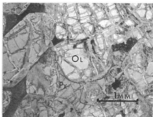
Fig. 3 Wehrlitic gabbro. Texture is ortho- to meso-cumulate.
