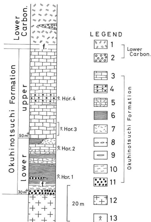
Text-fig. 4 Geological columnar section of the Okuhinotsuchi Formation.
