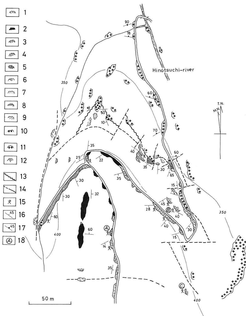
Text-fig. 3 Geological sketch map of the Okuhinotsuchi Formation in the main area of its distribution.
