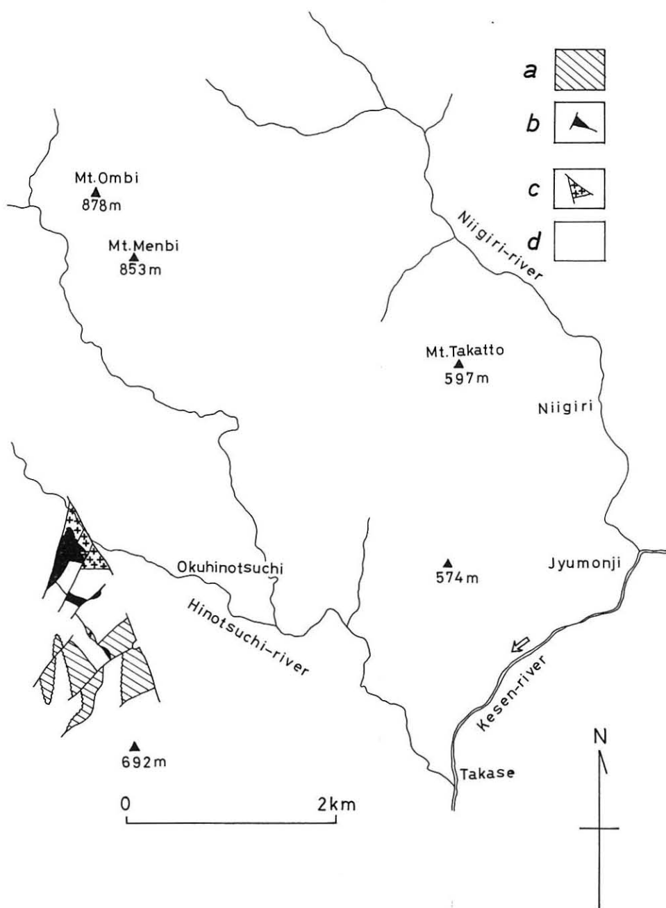
Text-fig. 2 Map showing the distribution of the Silurian Okuhinotsuchi Formation.
