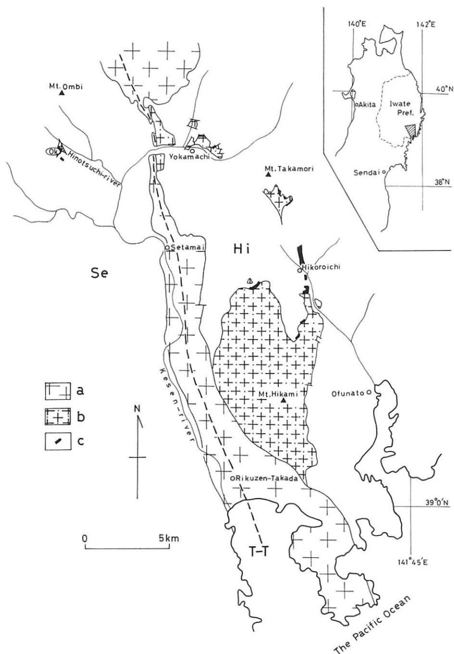
Text-fig. 1 Map showing the distribution of Silurian deposits in the southern Kitakami Mountains.
