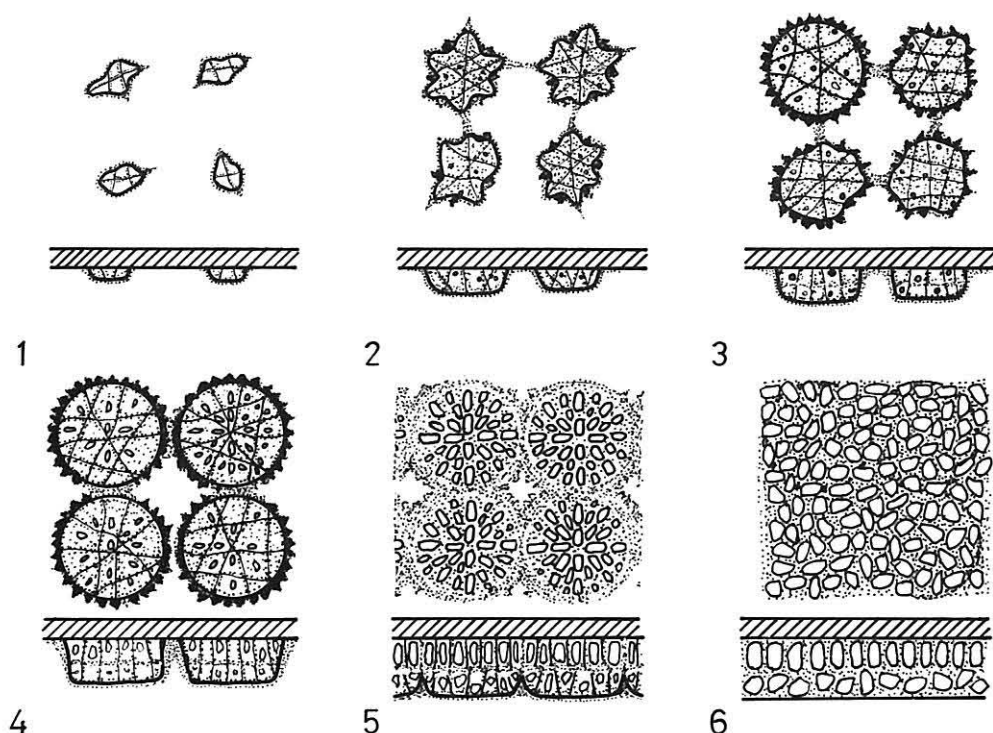
Text-figure 1 Stylized diagram of the mineralization and aggregation process in the larval shell of Haliotis . Horizontal and profile views of the organic spherules are illustrated.
